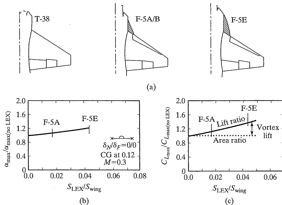
Figure 7.54 Effect of wing leading-edge extensions on the maximum angle of attack and the maximum lift for the F-5 family of aircraft: (a) configurations; (b) maximum angle of attack; (c) maximum lift. [From Stuart (1978).]
