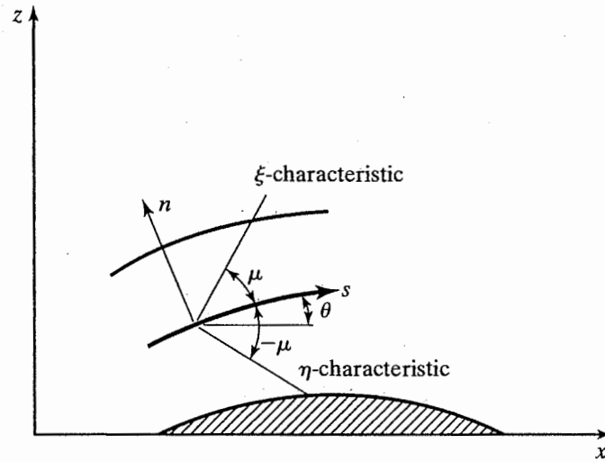
Figure 8.8 Supersonic flow around an airfoil in natural (streamline) coordinates.
