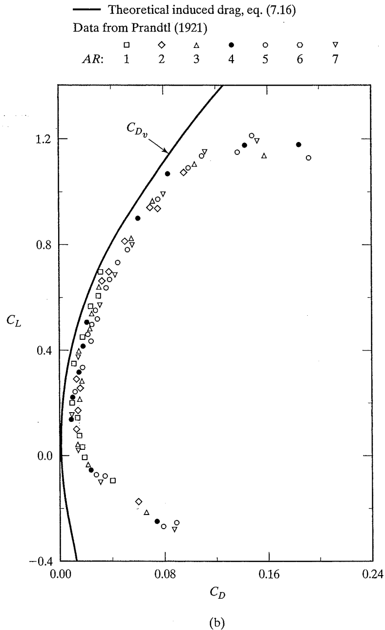
Figure 7.9 ( continued ) (b) drag polars converted to AR = 5 .
