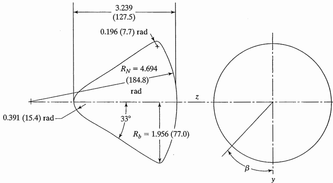
Figure 12.31 Clean (no protuberances) Apollo Command Module. Dimensions in meters (inches).
