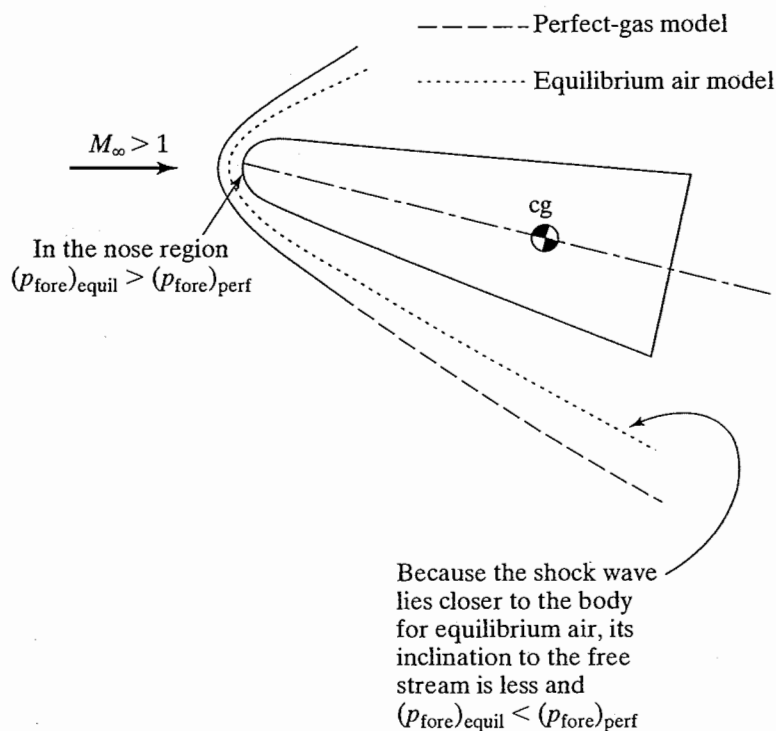
Figure 12.35 Hypersonic flow past an inclined spherically blunted cone comparing perfect-gas and equilibrium-air pressures.
