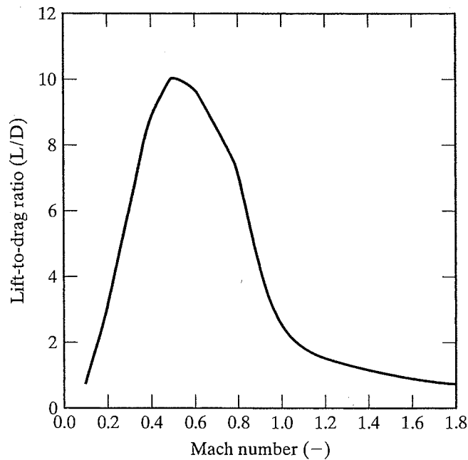
Figure 5.32 L/D ratio as a function of the Mach number for an F-16C flying at 20,000 ft.
