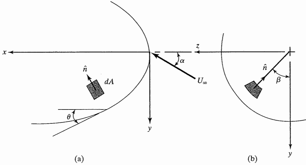
Figure 12.13 Coordinate system nomenclature for axisymmetric configurations; (a) side view; (b) front view.
