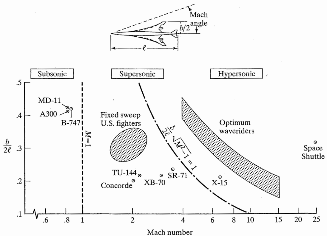
Figure 11.37 Aircraft classification by speed regime. [Taken from Harris (1992).]
