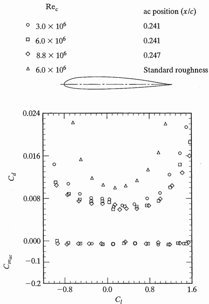
Figure 5.13 Section drag coefficient and section moment coefficient (with respect to the ac) for a NACA 23012 airfoil. [Data from Abbott and von Doenhoff (1949).]
