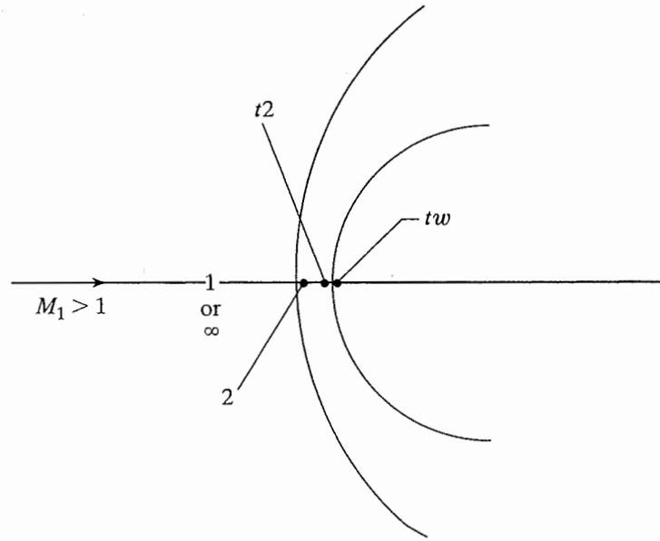
Figure 12.4 Nomenclature for the stagnation region. 1 or \infty , free-stream conditions; 2, conditions immediately downstream of the shock wave; t2 , conditions at the stagnation point (downstream of the normal portion of the shock wave) but outside the boundary layer; tw , conditions at the wall at the downstream stagnation point.
