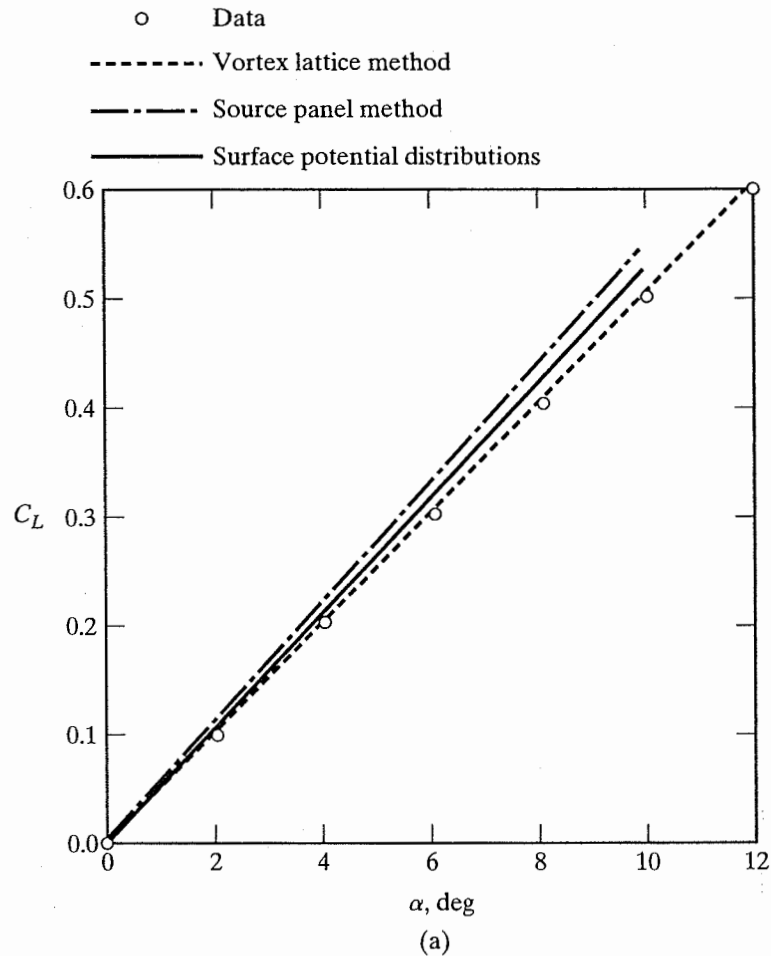
Figure 7.23 Comparison of the lift coefficient as a function of angle of attack: (a) \Lambda_{c/4} = 45^\circ , NACA 64A010 section, AR = 3.0 , \lambda = 0.5 , aft swept wing. [From Margason et al. (1985).]
