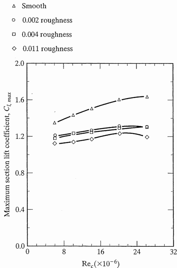
Figure 5.17 Effect of roughness near the leading edge on the maximum section lift for the NACA, 63(420)-422 airfoil. [Data from Abbott and von Doenhoff (1949).]
