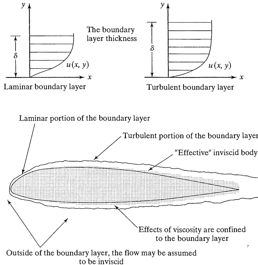
Figure 2.13 Viscous boundary layer on an airfoil.
