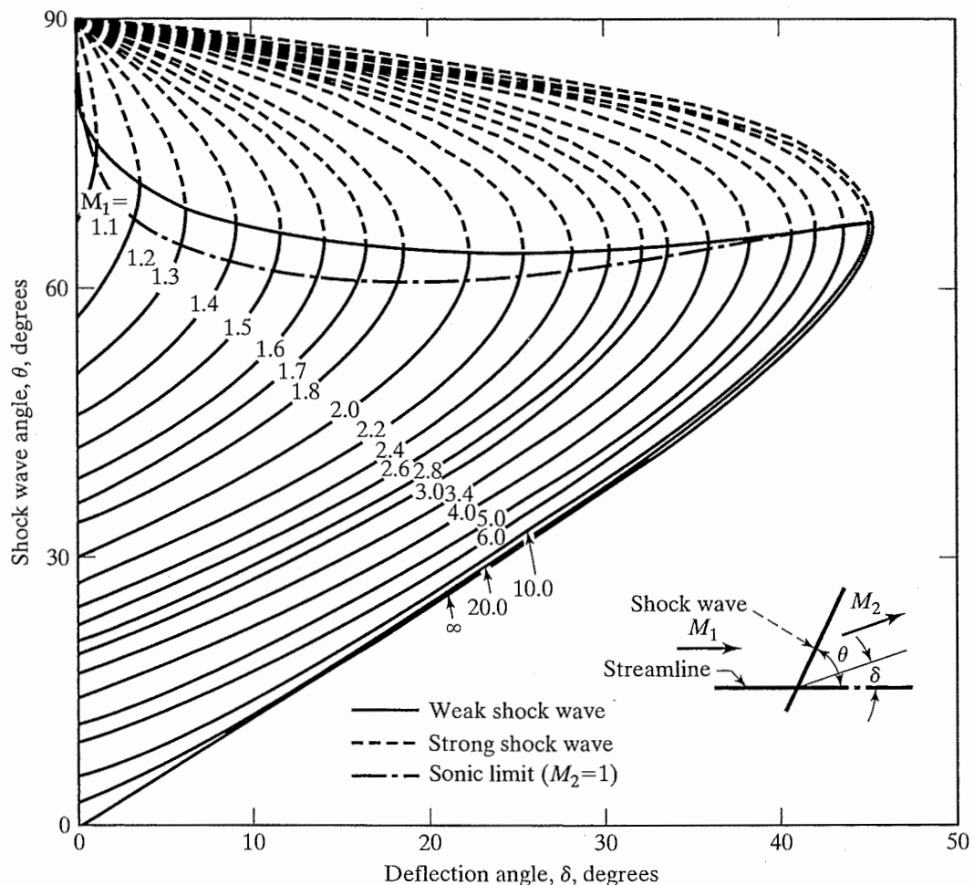
Figure 8.12 Variation of shock-wave parameters with wedge flow-deflection angle for various upstream Mach numbers, \gamma = 1.4 : (a) shock-wave angle.
