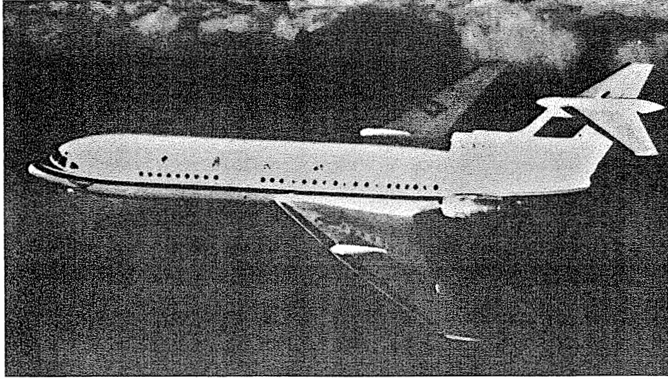
Figure 7.35 Trident illustrating boundary-layer fences on the wing. (Courtesy of British Aerospace.)
