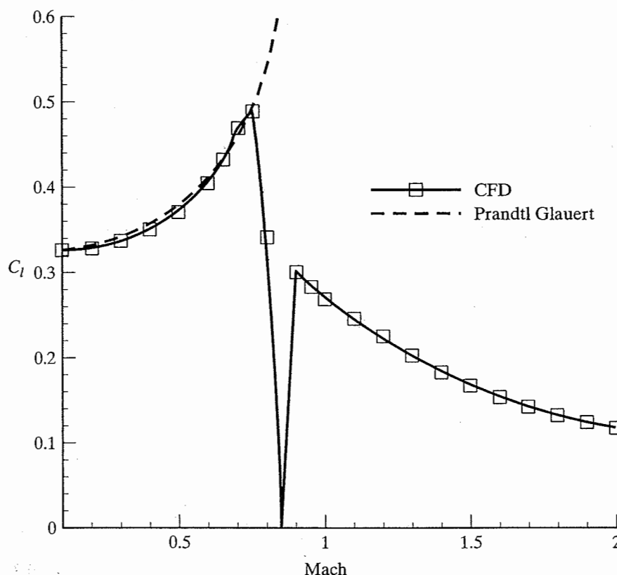
Figure 9.12 Section lift coefficient for a NACA 0012 airfoil as a function of the free-stream Mach number. [As provided by Forsythe and Blake (2000).]
