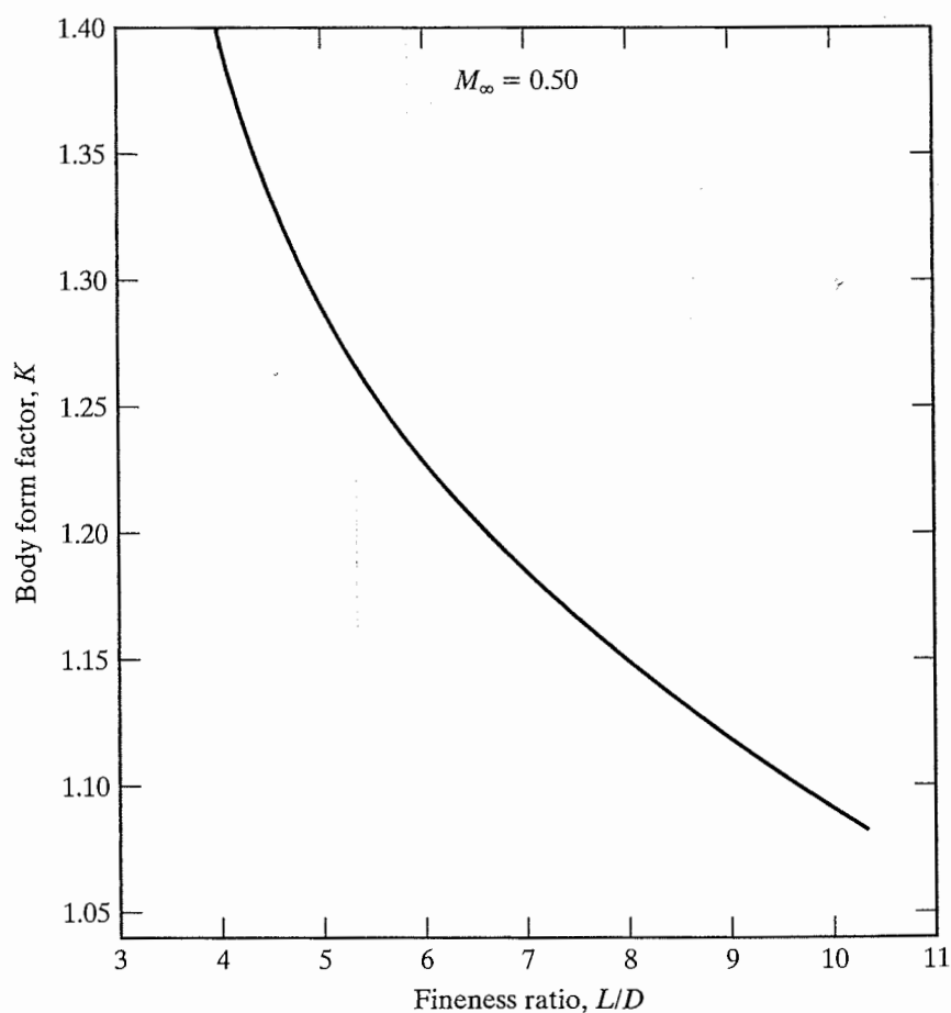
Figure 5.22 Body form factor as a function of fuselage fineness ratio. [From Shevell (1989).]
