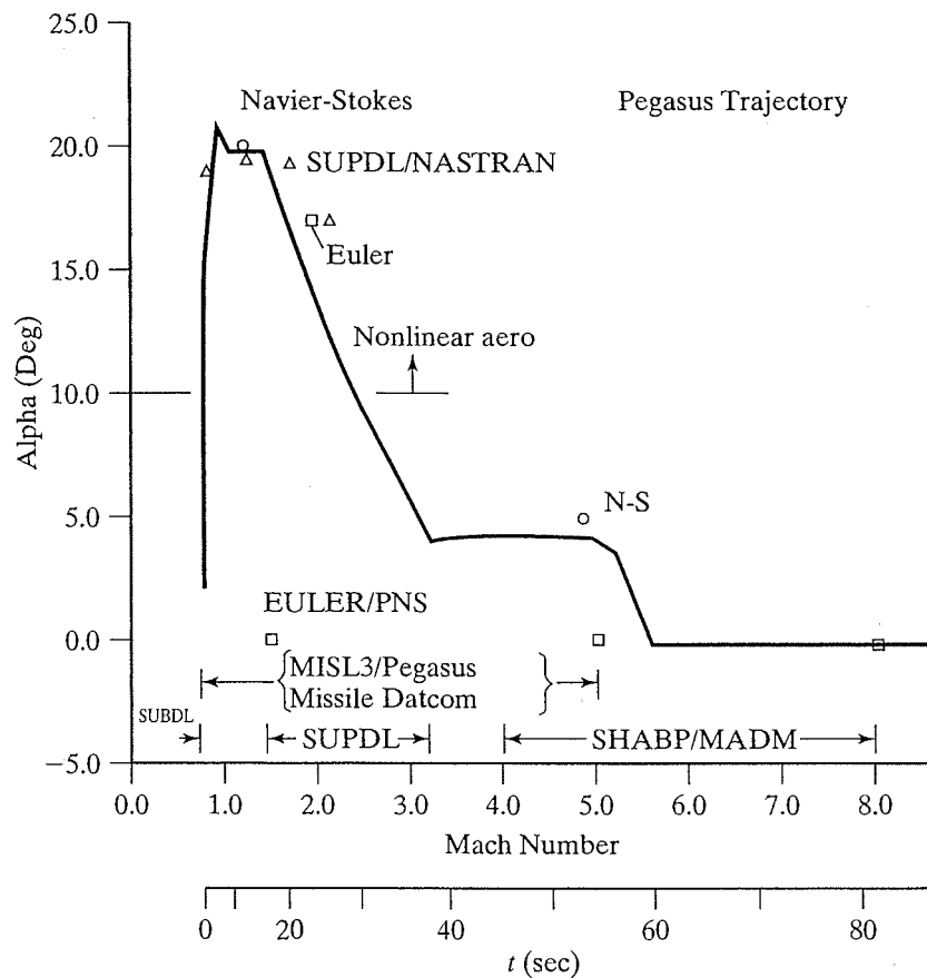
Figure 14.1 Aerodynamic analysis flight envelope; CFD tools used for \alpha/M_\infty space for the Pegasus TM . [Taken from Mendenhall et al. (1990).]
