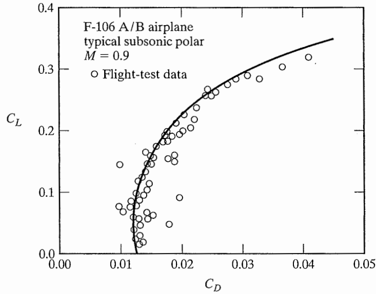
Figure 5.28 Flight data for a drag polar for F-106A/B aircraft at a Mach number of 0.9. [Taken from Piszkin et al. (1961)]
