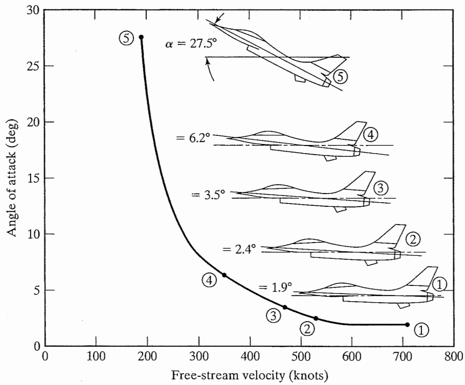
Figure 5.27 Correlation between the angle of attack and the velocity to maintain an F-16C in steady, level unaccelerated flight.
