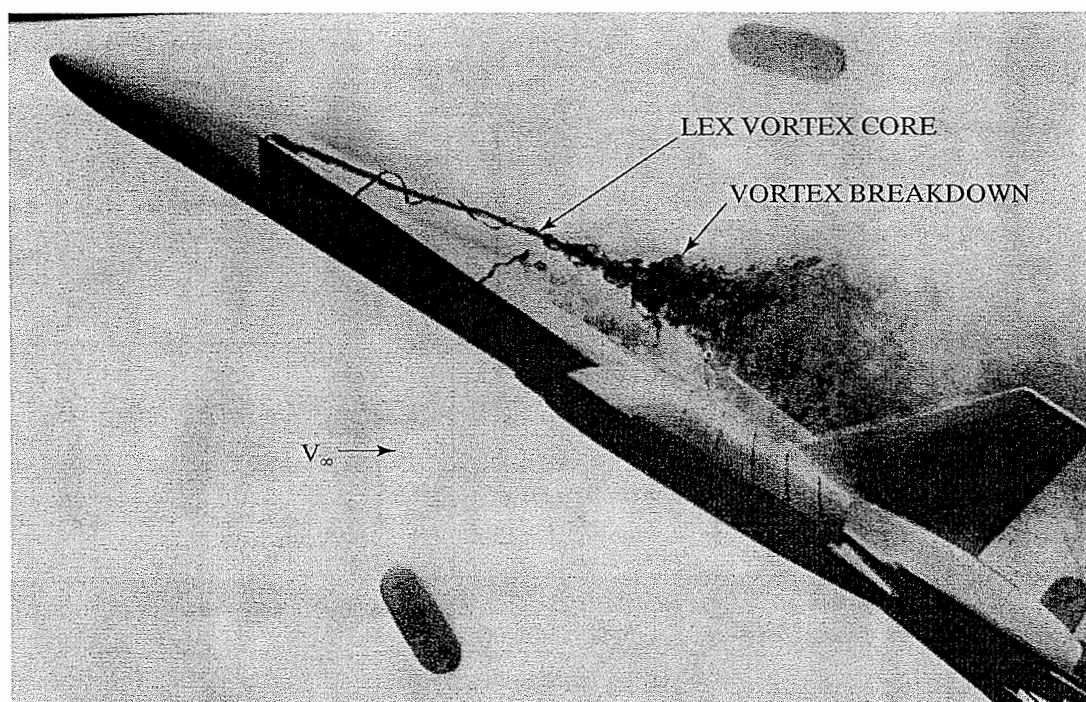
Figure 7.52 Flow visualization of a LEX vortex on a Subscale Advanced Fighter Model; \alpha = 32^\circ , Reynolds number = 10^4 from the Northrop Water Tunnel. [Taken from Erickson (1982).]
