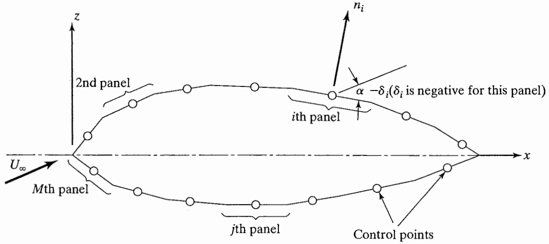
Figure 3.26 Source density distribution of the body surface.
