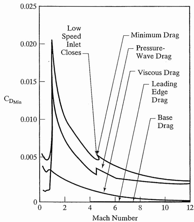
Figure 12.34 Minimum drag buildup for baseline vehicle. [Taken from Bogar et al. (1996b).]
