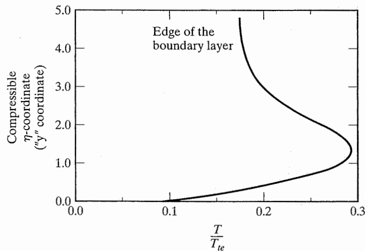
Figure 8.17 Static temperature distribution across a compressible, laminar boundary layer; M_e = 4.84 T_w = 0.095 T_{te} .
