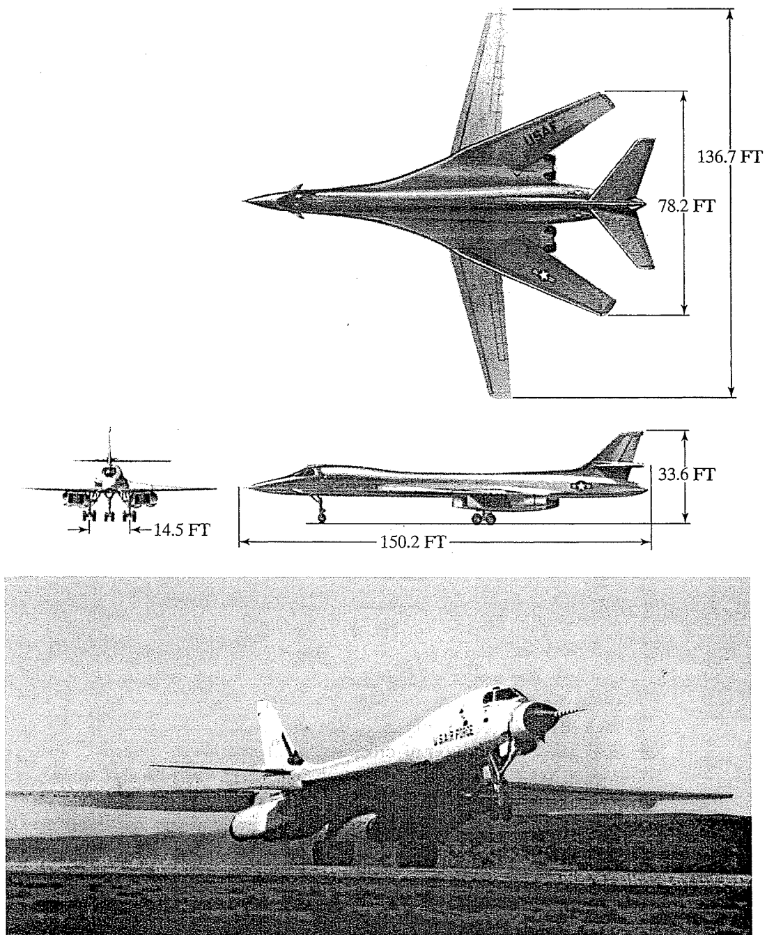
Figure 9.20 Variable geometry (swing-wing) aircraft, the Rockwell International B-1: (a) three-view sketches illustrating the variable-geometry wing; (b) low-speed configuration. (Courtesy of Rockwell International.)
