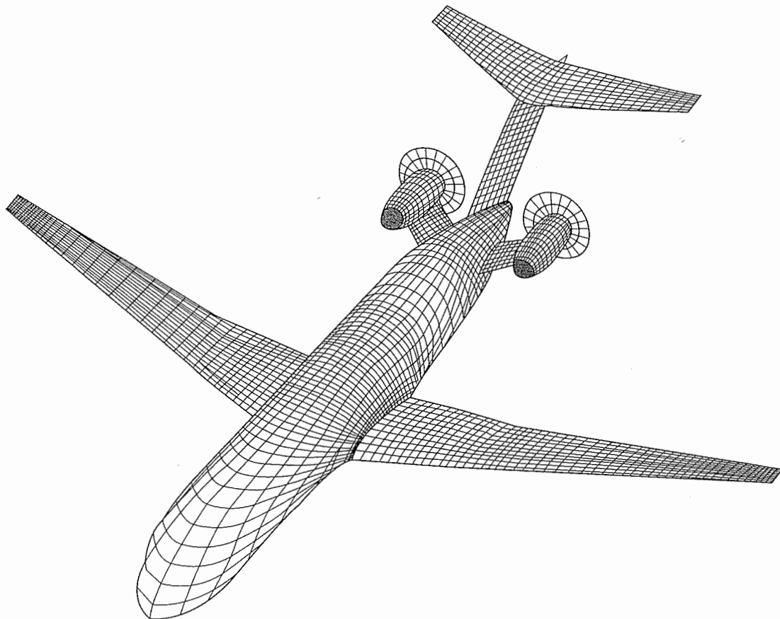
Figure 9.33 Structured surface-fitted grid for an advanced prop-fan airplane. [From Kusunose et al. (1987).]
