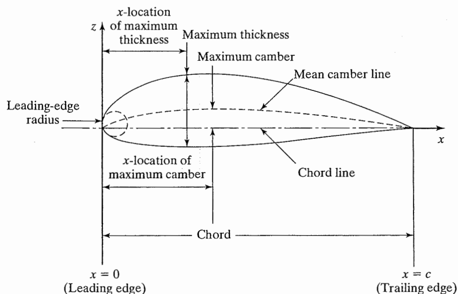
Figure 5.5 Airfoil-section geometry and its nomenclature.
