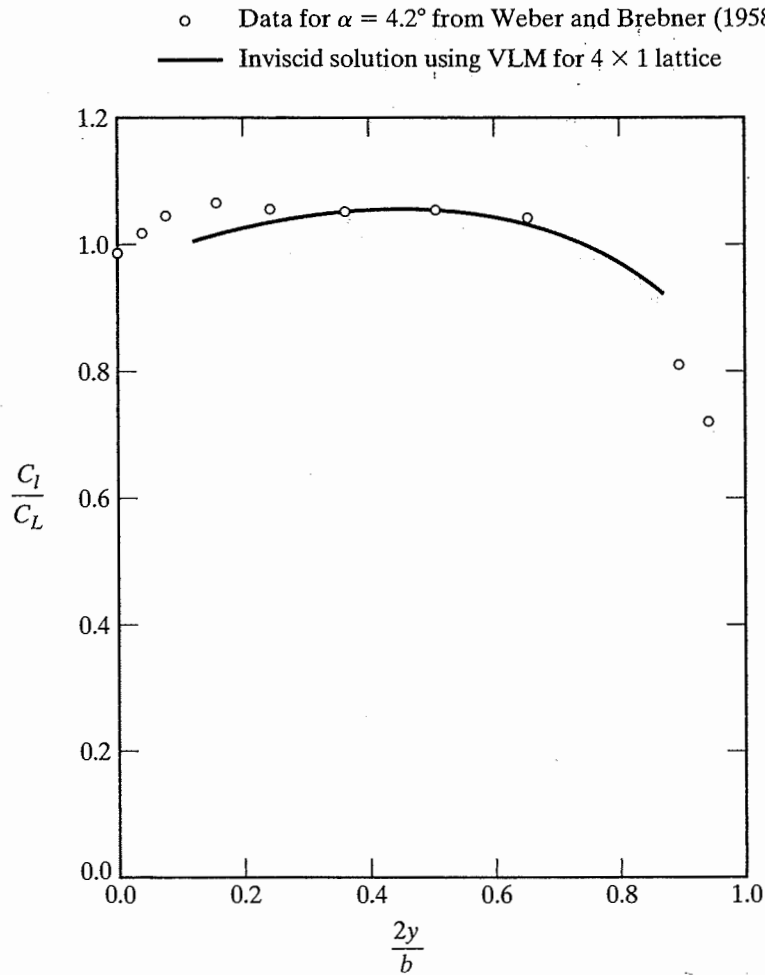
Figure 7.33 Comparison of the theoretical and the experimental spanwise lift distribution for the wing of Fig. 7.31.
