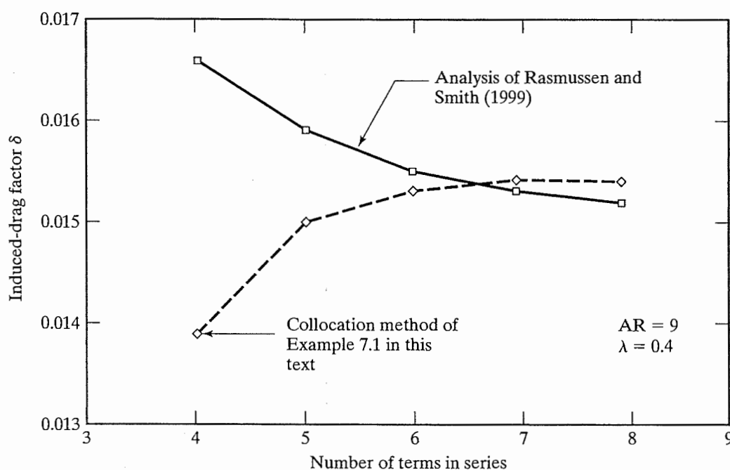
Figure 7.19 Convergence properties of induced-drag factor \delta for tapered wing, \lambda = 0.4 . [Taken from Rasmussen and Smith (1999).]
