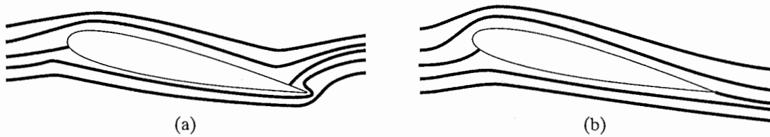
Figure 6.3 Streamlines around the airfoil section: (a) zero circulation, stagnation point on the rear upper surface; (b) full circulation, stagnation point on the trailing edge.
