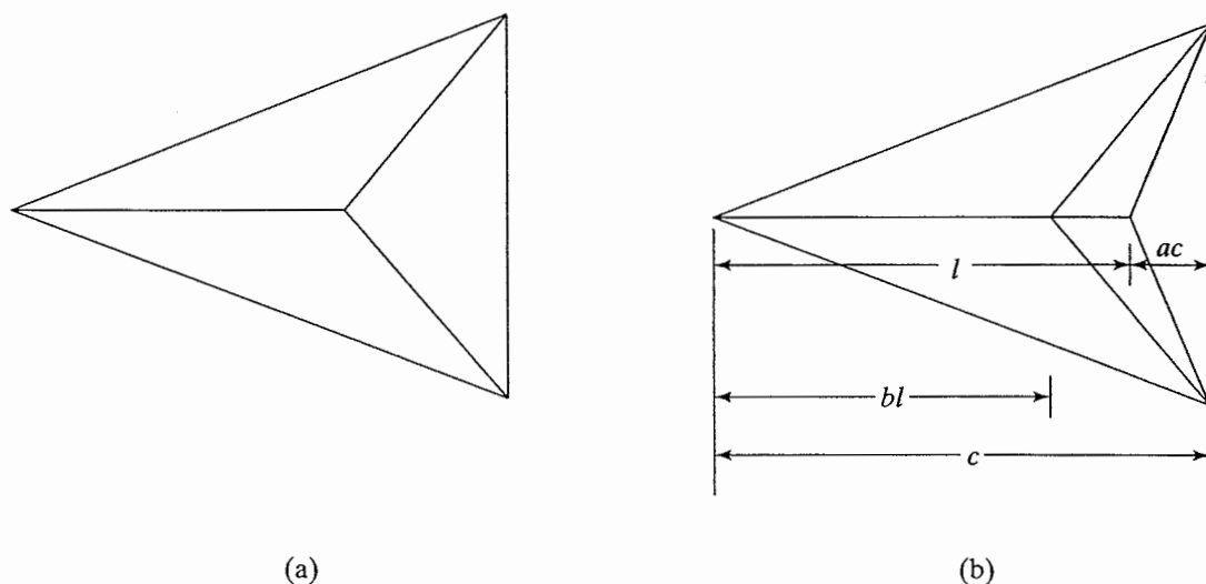
Figure 11.17 Delta- and arrow-wing planforms with double-wedge sections: (a) delta planform; (b) arrow planform.
