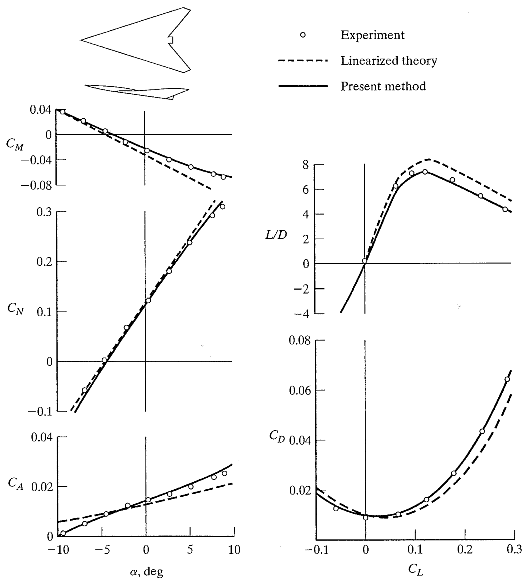
Figure 11.35 Comparison of the predicted and the measured forces and moments for 72.65° swept leading-edge arrow wing; M_\infty = 2.6 ; design value of C_L = 0.12 . [Taken from Carlson and Mack (1980).]
