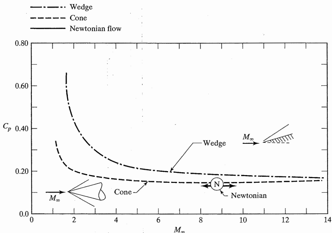
Figure 12.3 Pressure coefficient for the flow of perfect air past a wedge and a cone; deflection angle is 15^\circ .
