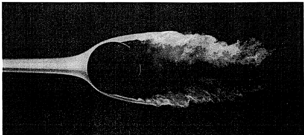
Figure 3.18 Smoke visualization of flow pattern for subcritical flow around a cylinder. (Photograph by F. N. M. Brown, courtesy of T. J. Mueller of University of Notre Dame.)
