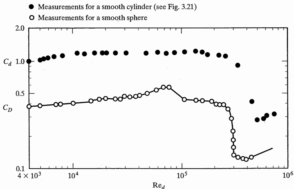
Figure 3.30 Drag coefficient for a sphere as a function of the Reynolds number. [From Schlichting, Boundary-Layer Theory (1968), with permission of McGraw-Hill.]
