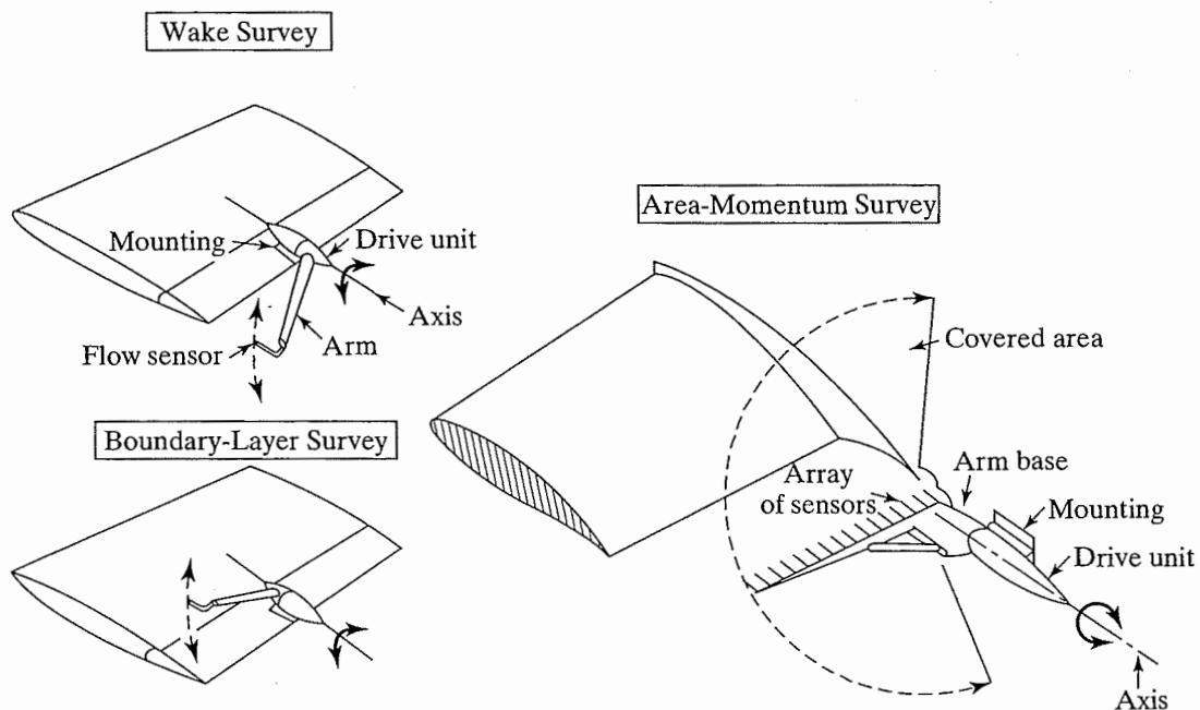
Figure 5.14 Airborne traversing probe concept and configurations. [From Bowes (1974).]
