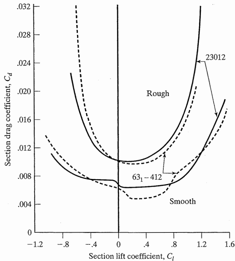
Figure 6.13 Drag characteristics of NACA laminar flow and conventional airfoil sections with both smooth and rough leading edges. [Loftin (1985).]
