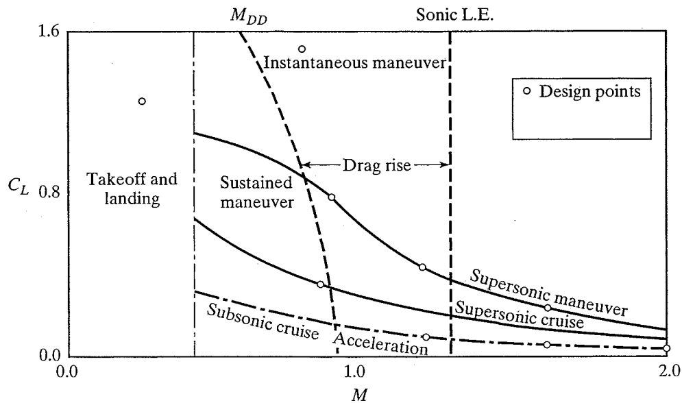
Figure 13.18 Typical performance map for fighters. [From Bradley (1981).]
