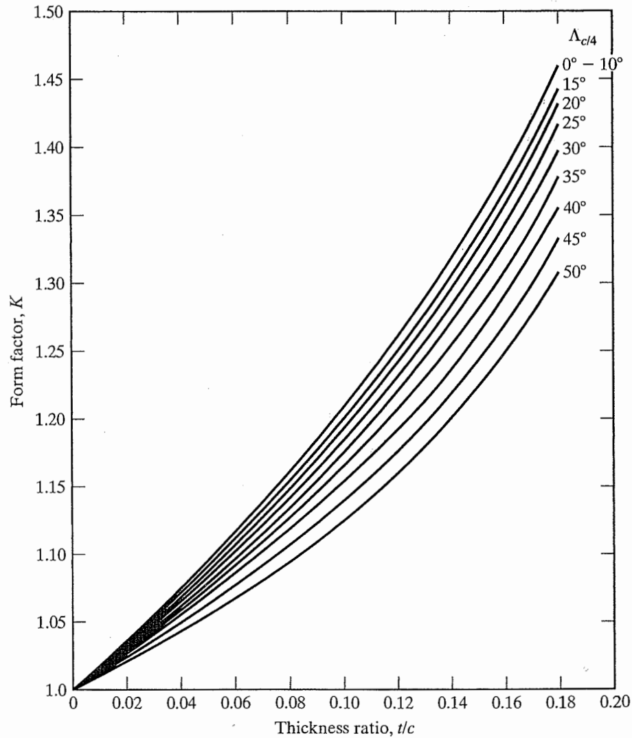
Figure 5.20 Wing form factor as a function of wing thickness ratio and quarter-chord sweep angle. [From Shevell (1989).]
