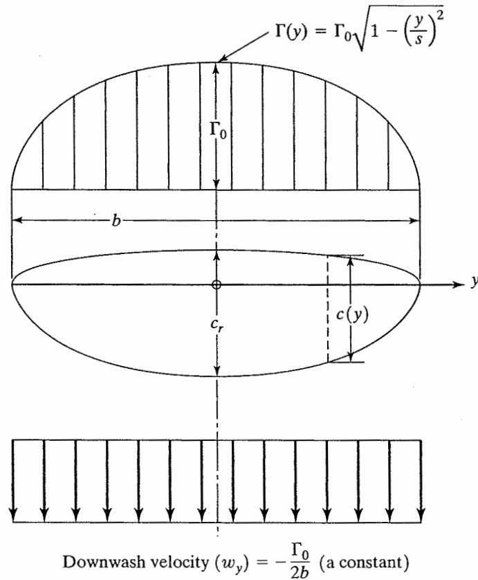
Figure 7.7 Elliptic-circulation distribution and the resultant downwash velocity.
