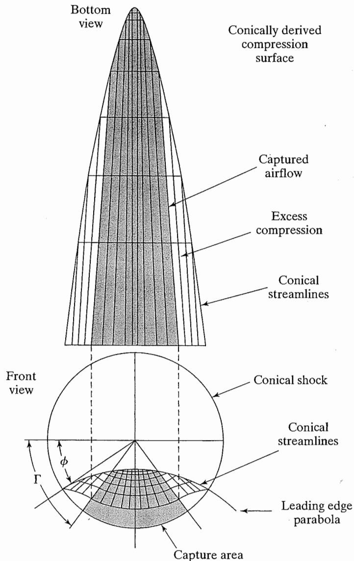
Figure 12.28 Compression surface derived from a conical flow field. [Taken from Cervisi and Grantz (1994).]
