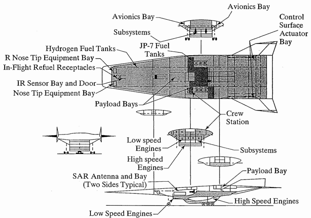
Figure 12.33 Mach 10 dual-fuel lifting-body cruise configuration. [Taken from Bogar et al. (1996b).]
