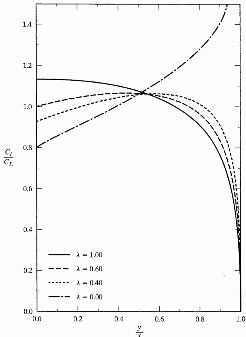
Figure 7.17 Effect of taper ratio on the spanwise variation of the lift coefficient for an untwisted wing.
