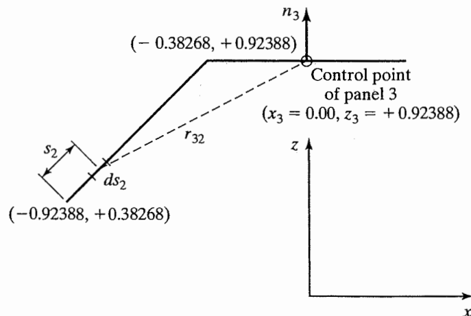
Figure 3.28 Detailed sketch for calculation of the contribution of the source distribution on panel 2 to the normal velocity at the control point of panel 3.
