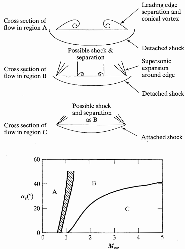
Figure 12.21 Types of flow on thin delta wings at supersonic speeds. [As taken from Squire (1976a).]
