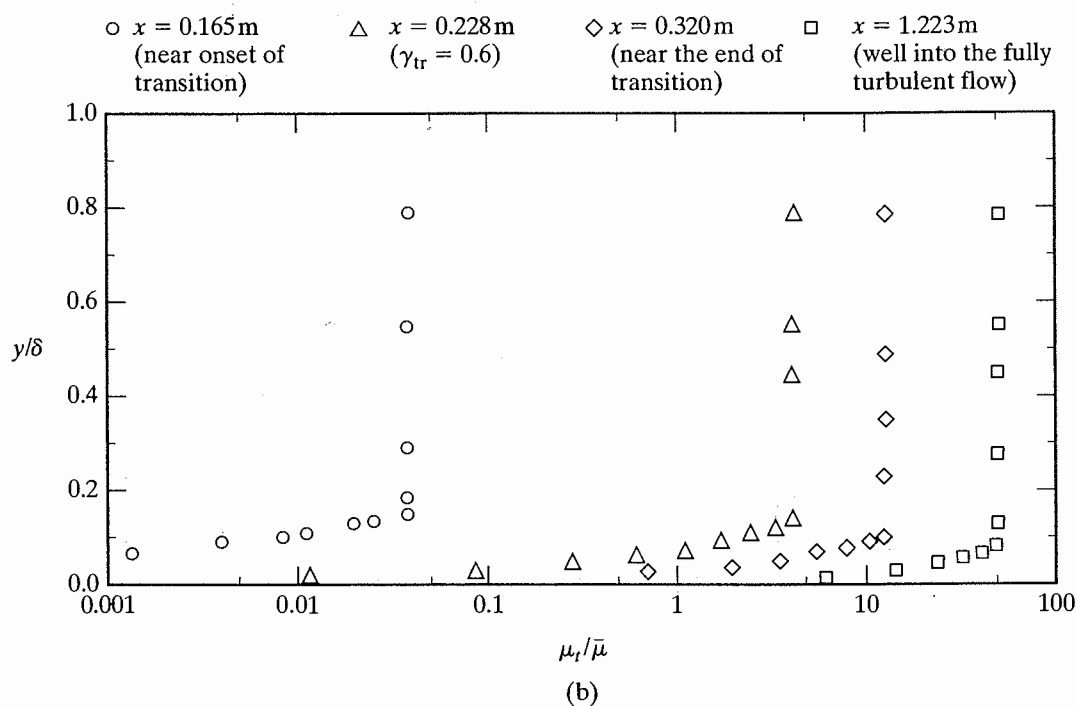
Figure 4.16 Sample of computed boundary layer for incompressible flow past a flat plate, u_e = 114.1 ft/s, T_e = 542^\circ R , P_e = 2101.5 psf, T_w = 540^\circ R : (a) skin friction distribution; (b) turbulent viscosity/thermodynamic viscosity ratio.
