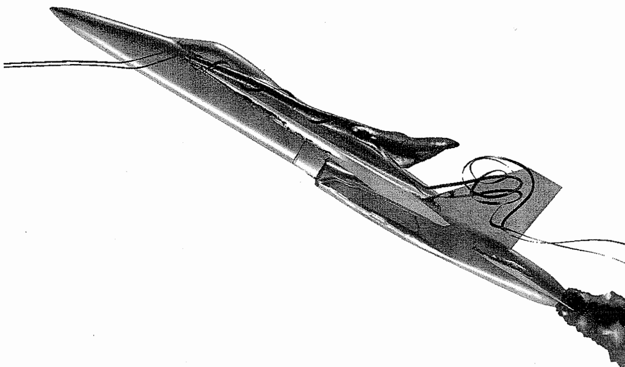
Figure 7.53 Flow-field computations for an F-18C at an angle of attack of 32^\circ , M_\infty = 0.25 , Re_L = 15 \times 10^6 . [Provided by Wurtzler and Tomaro (1999).]
