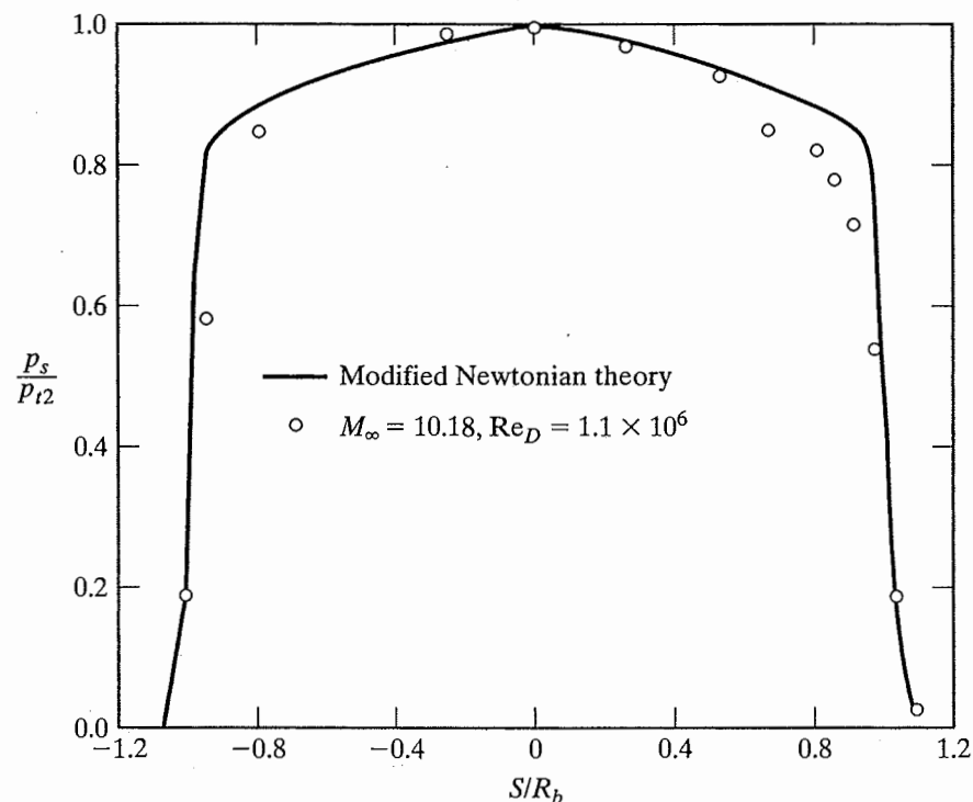
Figure 12.30 Comparison of the modified Newtonian pressures and the experimental pressures for the Apollo Command Module at \alpha = 0^\circ . [Taken from Bertin (1966).]
