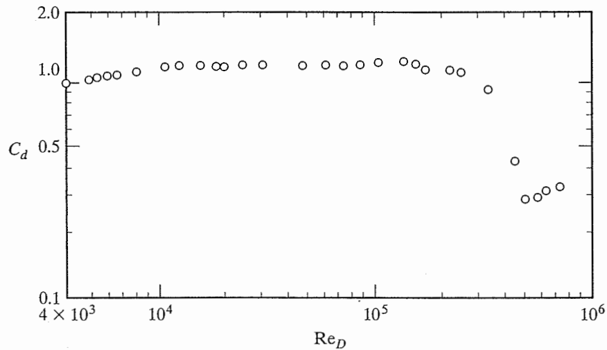
Figure 3.21 Drag coefficient for a smooth circular cylinder as a function of the Reynolds number. [From Boundary Layer Theory by H. Schlichting (1968), used with permission of McGraw-Hill Book Company.]
