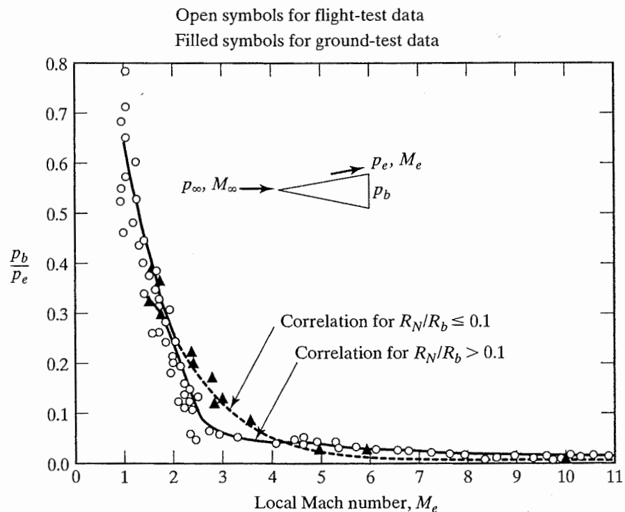
Figure 12.19 Base pressure ratio as a function of the local Mach number for turbulent flow. [From Cassanto (1973).]
