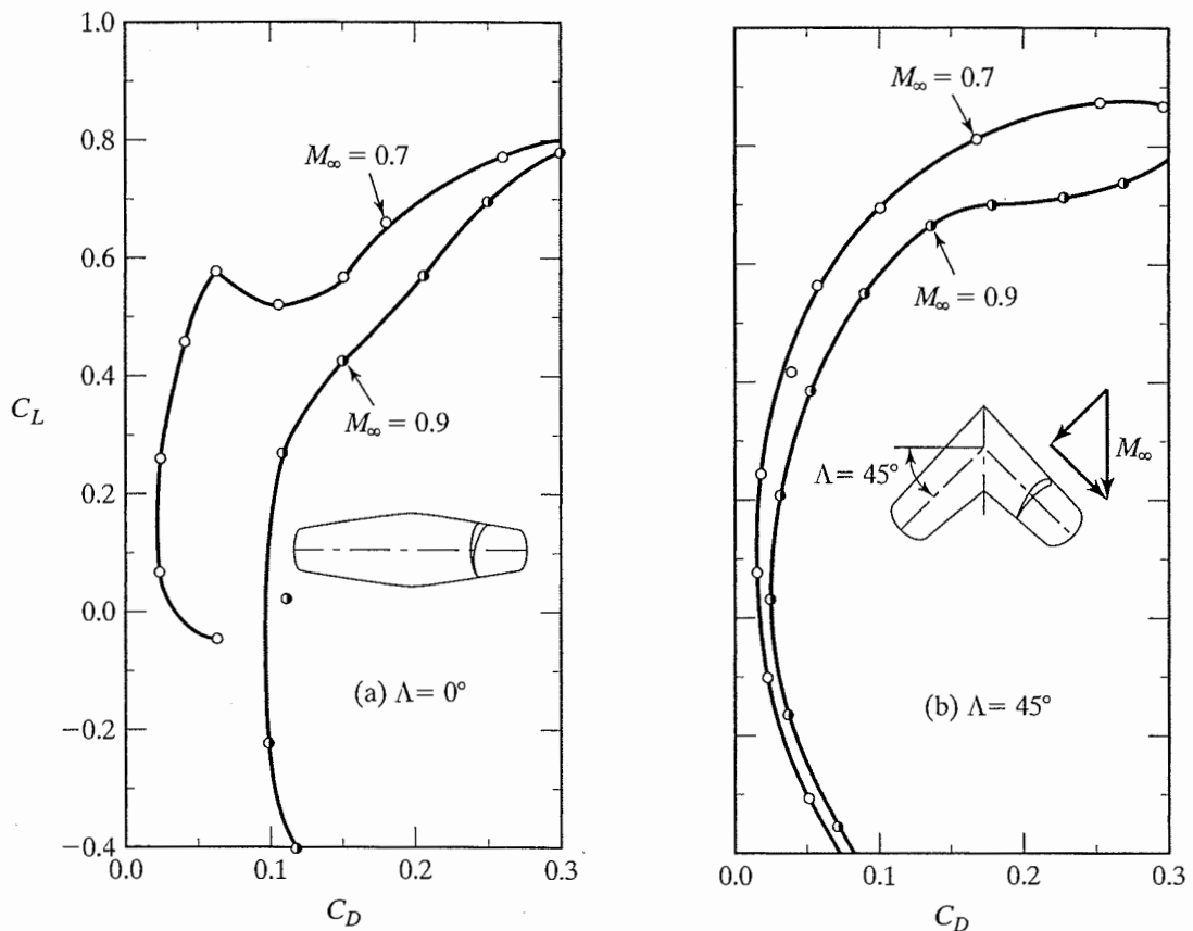
Figure 9.18 Comparison of the transonic drag polar for an unswept wing with that for a swept wing. [Data from Schlichting (1960).]
