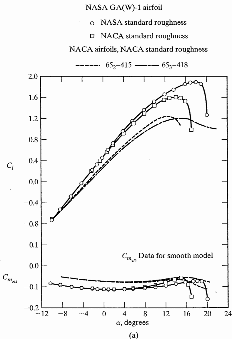
Figure 6.23(a) Aerodynamic coefficients for a NASA GA(W)-1 airfoil, for a NACA 65 2 -415 airfoil, and for a NACA 65 3 -418 airfoil; M_\infty = 0.20 , Re_c = 6 \times 10^6 : (a) lift coefficient and pitching moment coefficient curves; (b) drag polars. [Data from McGhee and Beasley (1973).]
