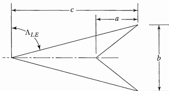
Figure 7.41 Wing geometry nomenclature.
