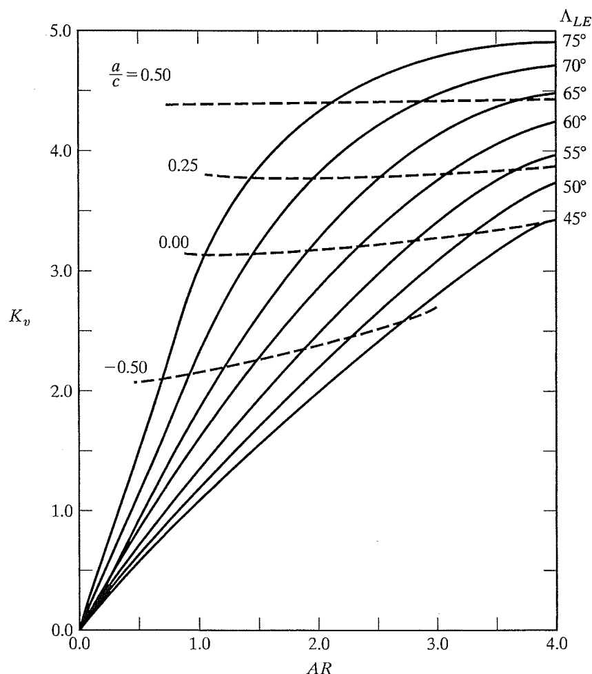
Figure 7.43 Variation of vortex-lift constant with planform parameters. [Taken from Pollhamus (1971b).]
