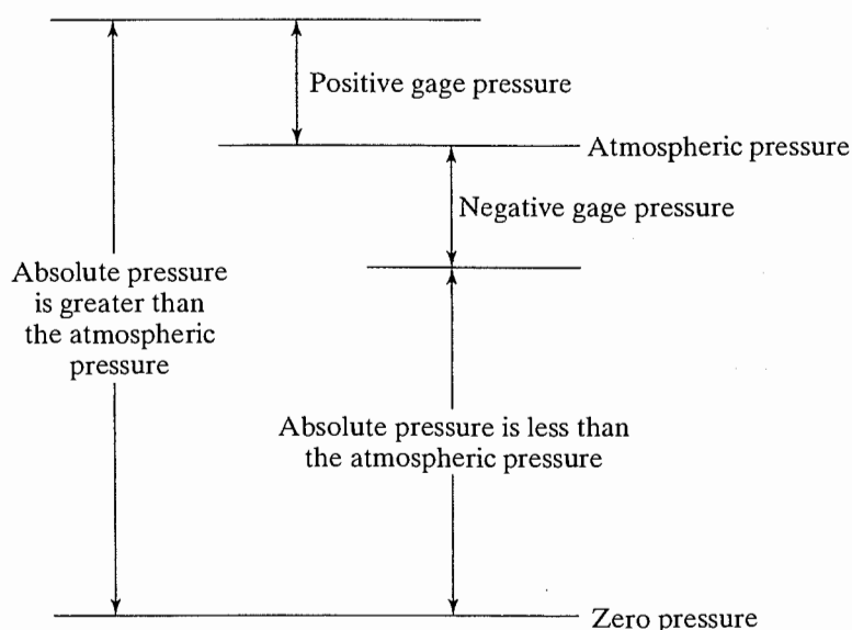
Figure 1.1 Terms used in pressure measurements.
