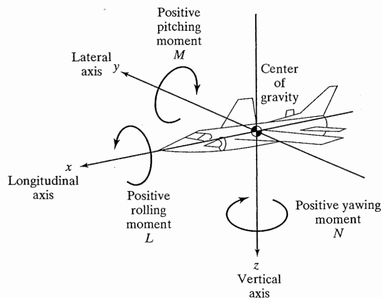
Figure 5.4 Reference axes of the airplane and the corresponding aerodynamic moments.
