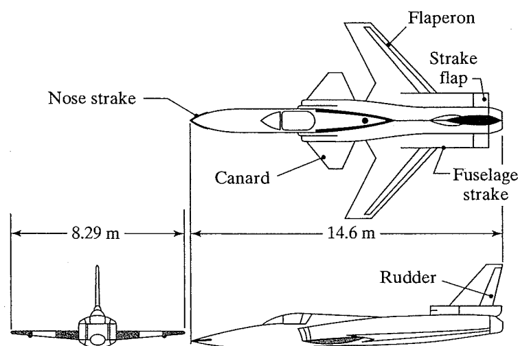
Figure 9.31 Three-view sketch of full-scale X-29 configuration.
