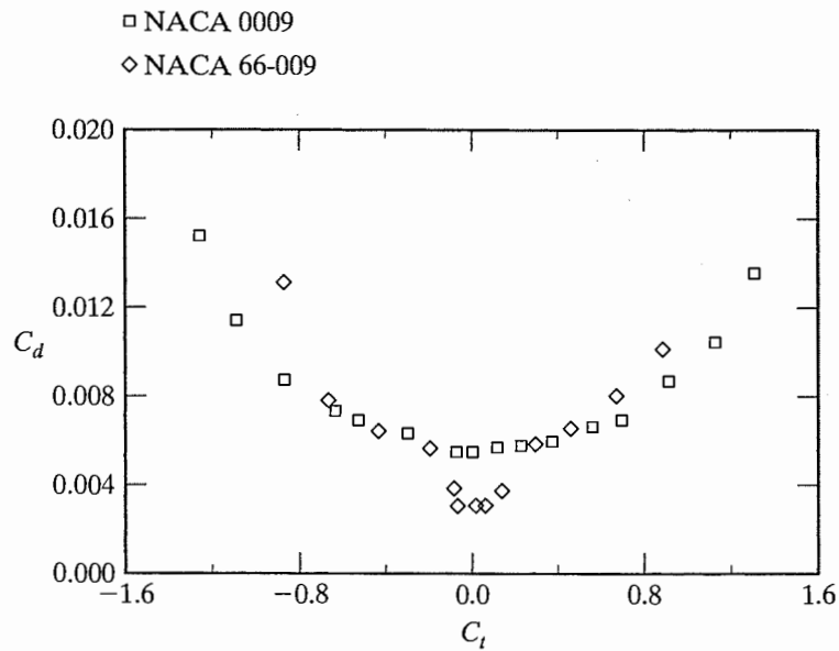
Figure 5.16 Section drag coefficients for NACA 0009 airfoil and the NACA 66-009 airfoil, Re_c = 6 \times 10^6 . [Data from Abbott and von Doenhoff (1949).]
