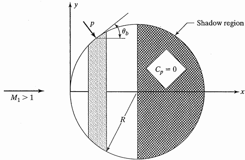
Figure 12.10 Sketch for calculating the modified Newtonian pressure drag on a sphere, Example 12.1.
