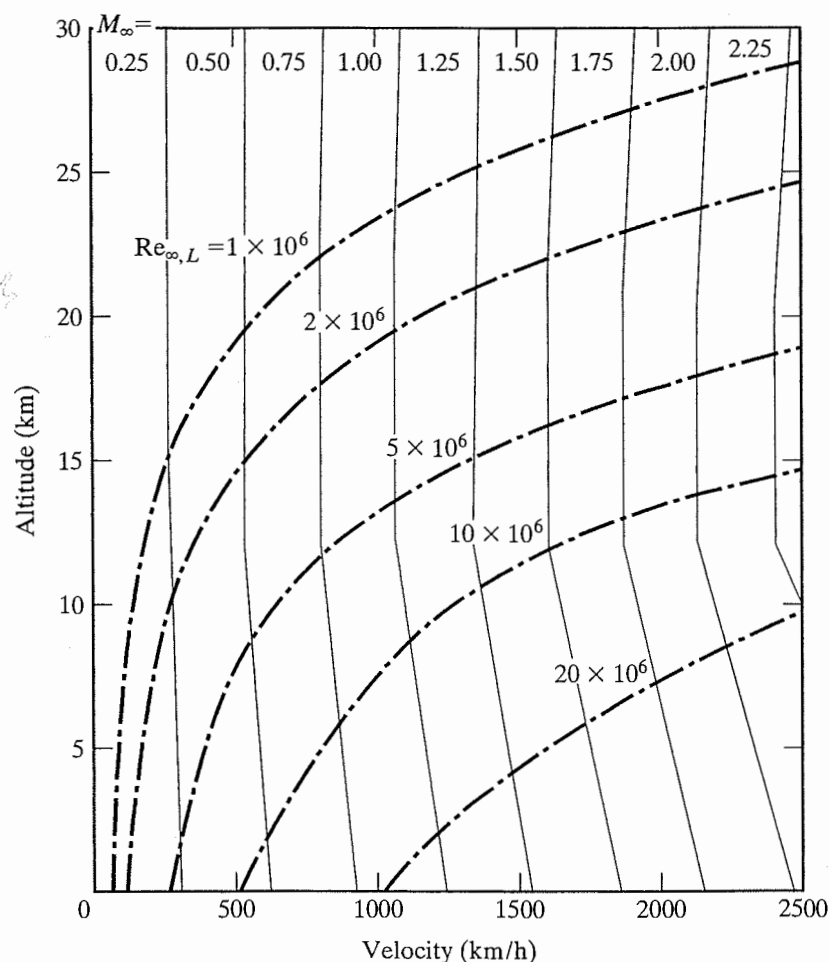
Figure 2.12 Reynolds number/Mach number correlations as a function of velocity and altitude for U.S. Standard Atmosphere.
