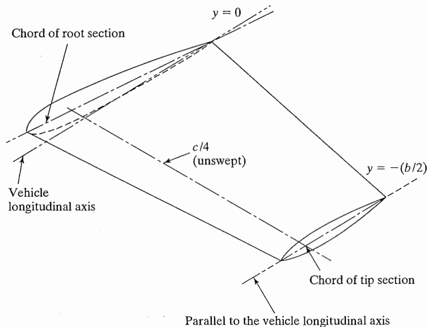
Figure 5.7 Unswept, tapered wing with geometric twist (wash out).
