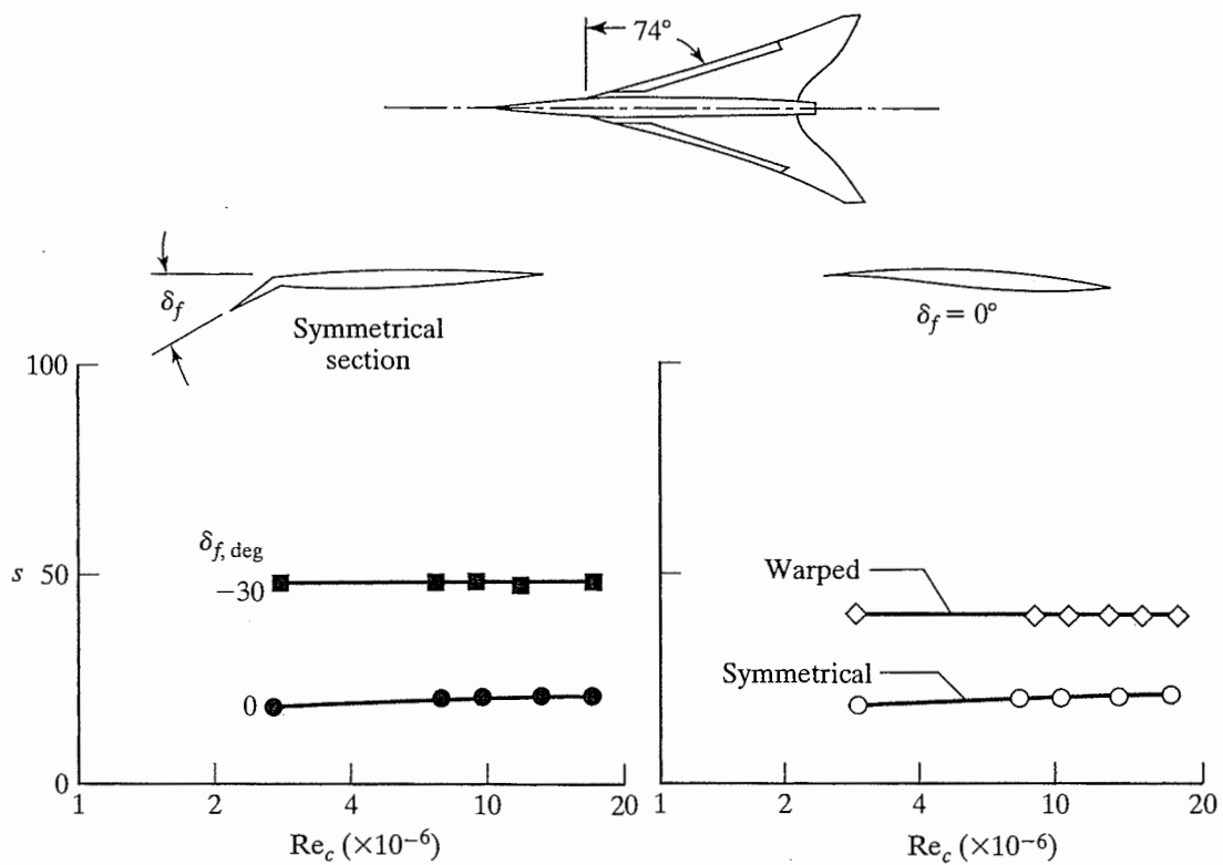
Figure 7.37 The effect of leading-edge flaps and wing warp on the effective leading-edge suction ( s ) for C_{L,opt} , M < 0.30 . [Taken from Henderson (1966).]
