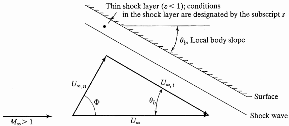
Figure 12.1 Nomenclature for Newtonian flow model.
