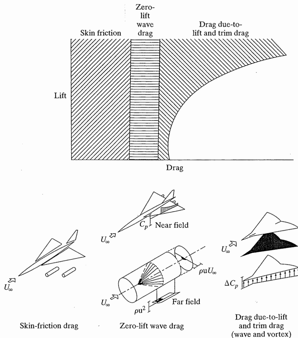
Figure 11.1 Drag buildup using superposition method of drag analysis. [From Middleton and Lundry (1980a).]
