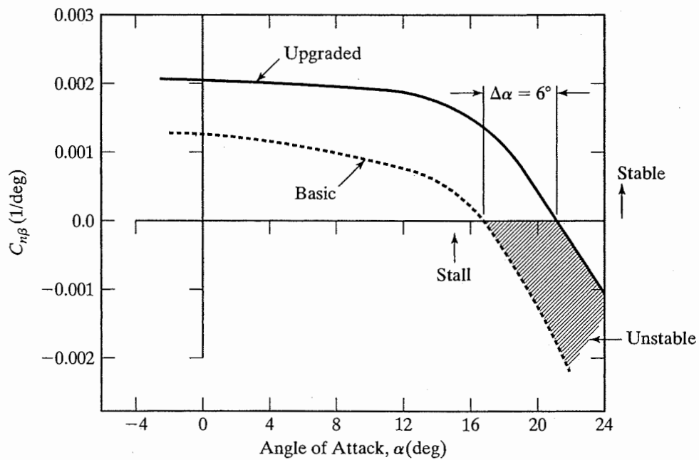
Figure 13.34 Combined effect of fin extension, strakes, and drooped inboard leading edges on lateral-directional stability. [From Gato and Masiello (1987).]
