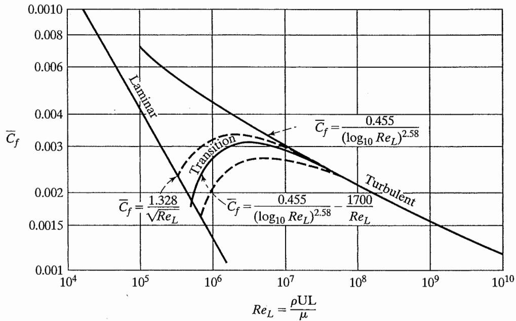
Figure 4.19 Variation of total skin-friction coefficient with Reynolds number for a smooth, flat plate. [From Dommasch, et al. (1967).]
