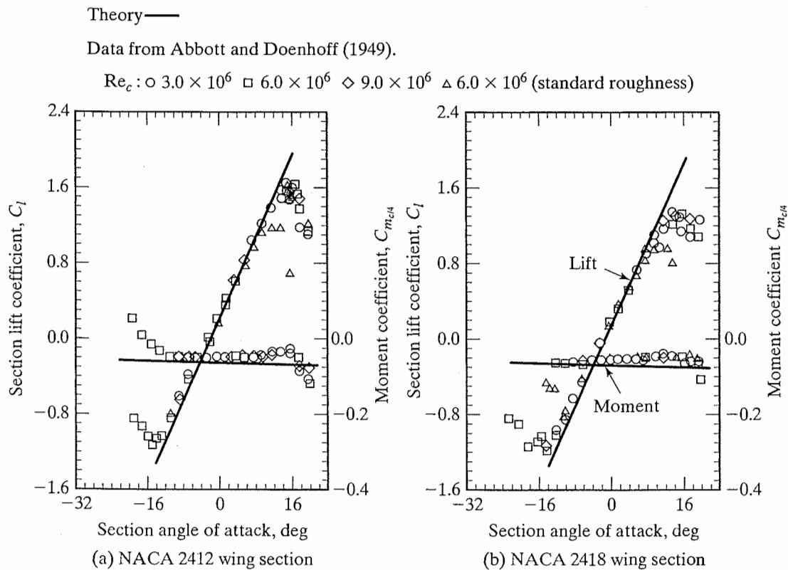
Figure 6.8 Comparison of the aerodynamic coefficients calculated using thin airfoil theory for cambered airfoils: (a) NACA 2412 wing section; (b) NACA 2418 wing section. [Data From Abbott and von Doenhoff (1949).]
