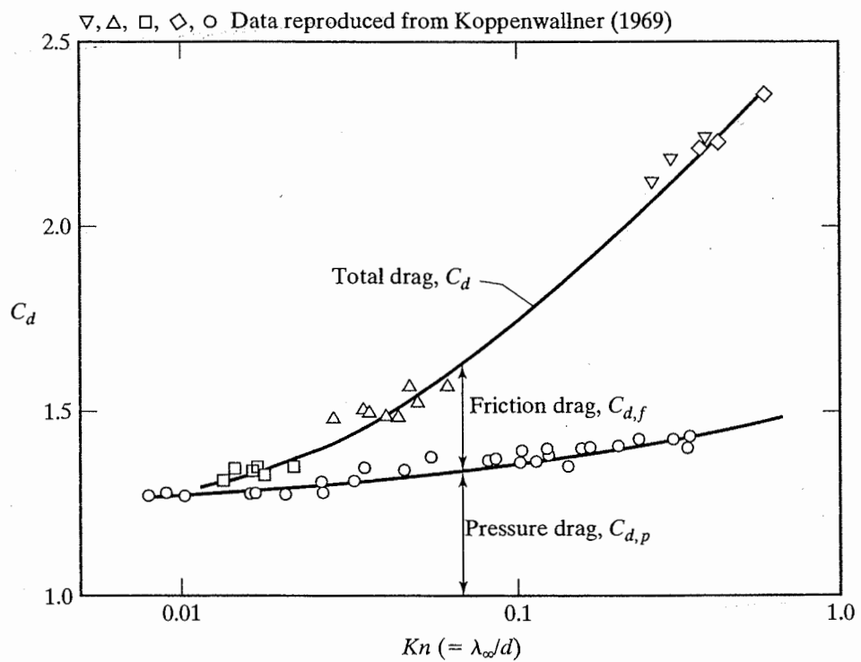
Figure 12.12 Contribution of the total drag due to friction drag and to pressure drag. [From Koppenwallner (1969).]
