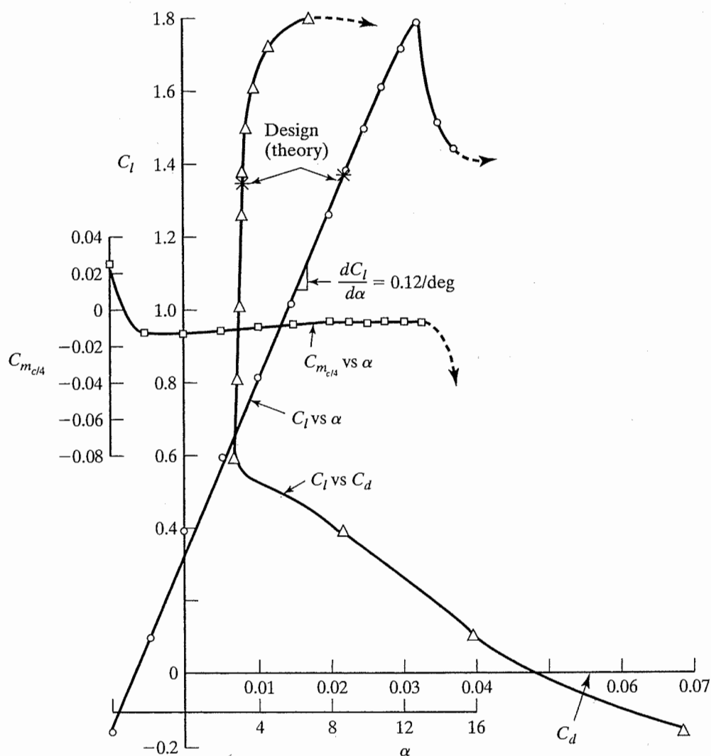
Figure 6.21 Experimental lift curve, drag polar, and pitching curve for a high-lift, single-element airfoil, Re_c = 3 \times 10^6 . [From Liebeck (1973).]
