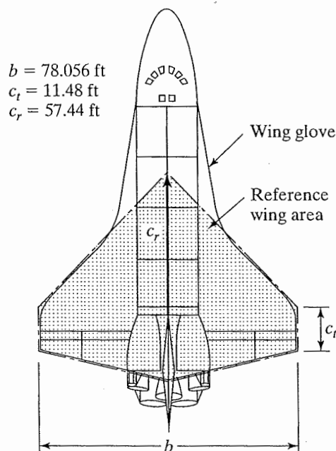
Figure 5.9 Sketch of Space Shuttle Orbiter geometry for Example 5.2.
