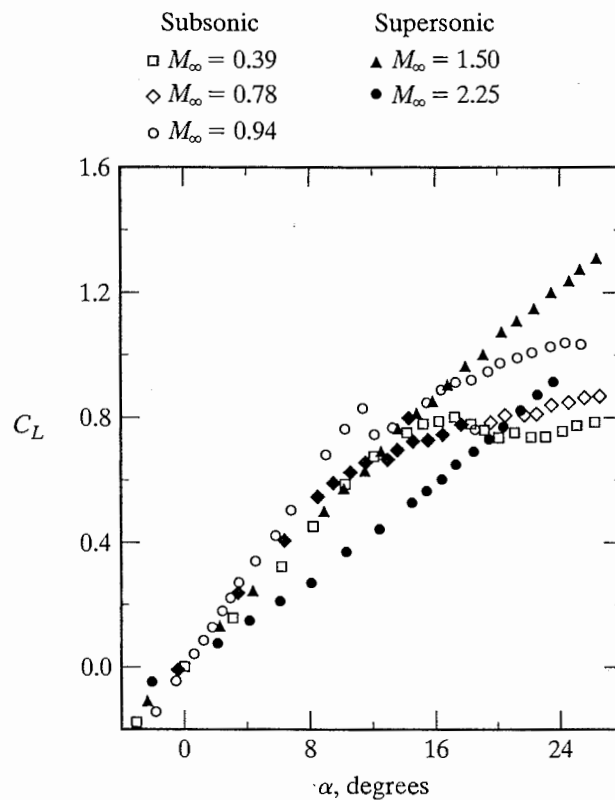
Figure 9.14 Effect of Mach number on the lift-coefficient/angle-of-attack correlation for a rectangular wing, AR = 2.75 . [Data from Stahl and Mackrodt (1965).]
