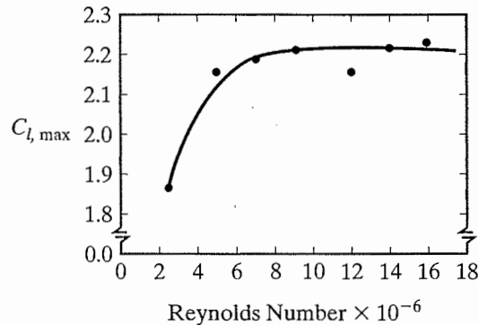
Figure 6.33 The effect of Reynolds number on C_{l,max} , \delta_n = 34^\circ , \delta_f = 35^\circ , \delta_s = 22.94^\circ . [Taken from Hobbs (1996).]
