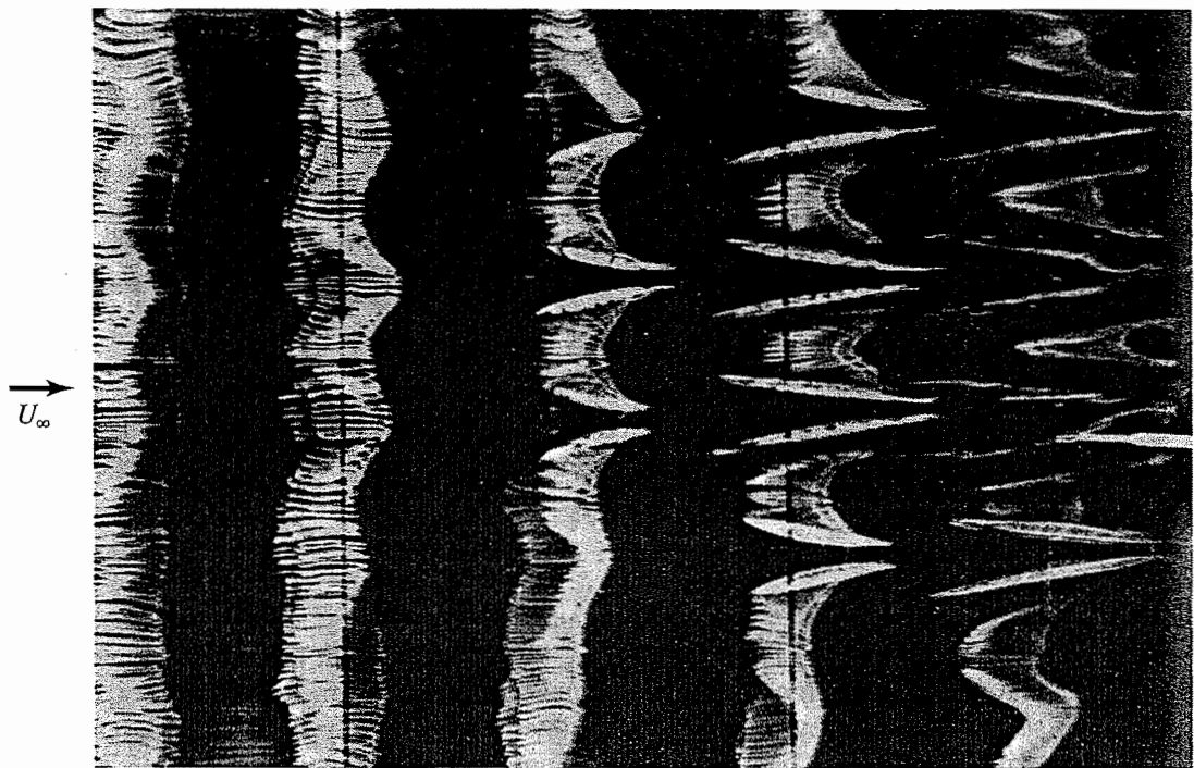
Figure 4.13 Flow visualization of the transition process on a flat plate. (Photograph supplied by A. S. W. Thomas, Lockheed Aeronautical Systems Company, Georgia Division.)
