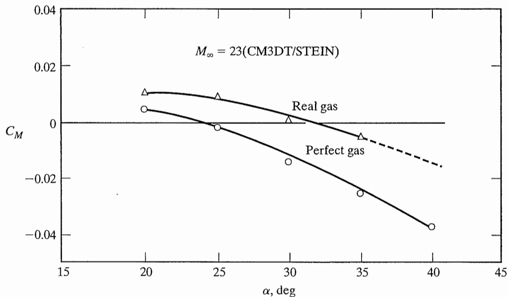
Figure 12.37 Comparison of perfect-gas and equilibrium-air calculations of the pitching moment for Space Shuttle Orbiter at M_\infty = 23 . [From Maus et al. (1984).]
