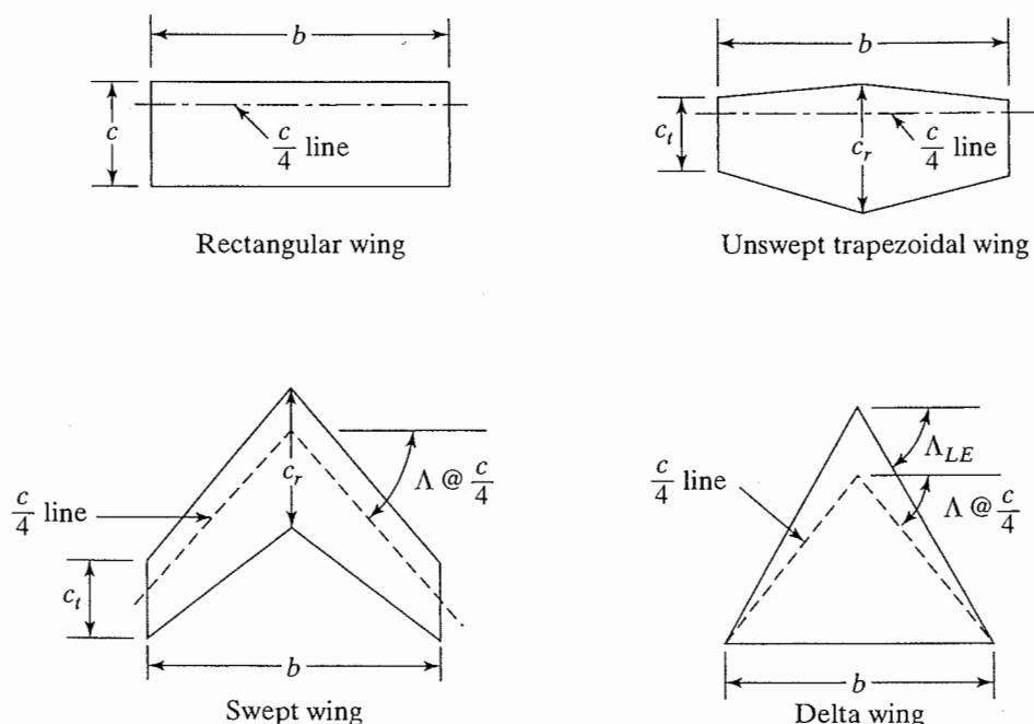
Figure 5.6 Geometric characteristics of the wing planform.
