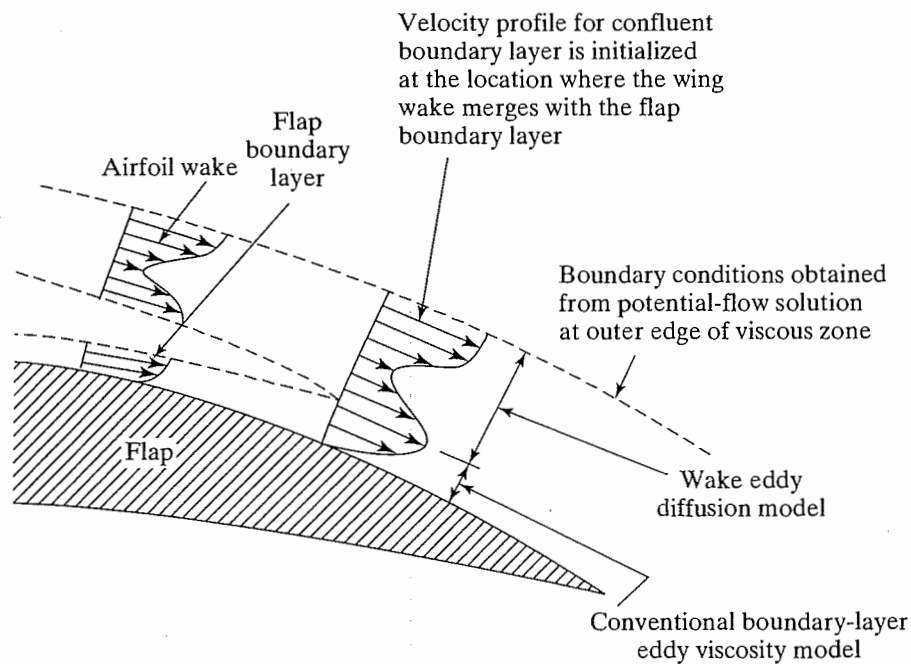
Figure 6.28 Flow model for merging of the wake from the principal airfoil with the boundary layer on the flap to form the confluent boundary layer on the upper surface of the flap. [From Olson et al. (1978).]
