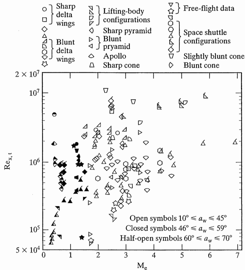
Figure 12.40 Transition Reynolds number as a function of local Mach number.
