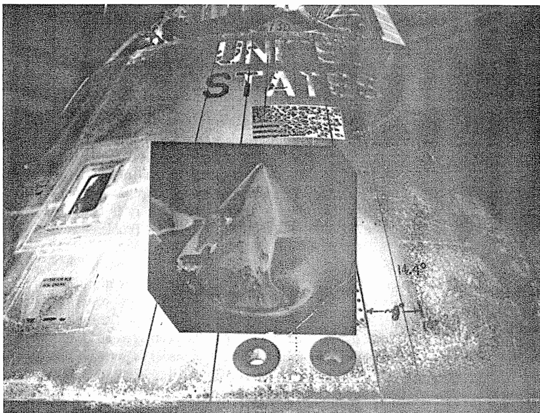
Figure 8.18 Comparison between the oil flow pattern (indicating skin friction) obtained in the wind tunnel and the char patterns on a recovered Apollo spacecraft. (Courtesy of NASA.)
