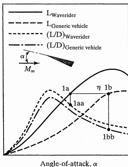
Figure 12.23 Curves of lift and (L/D) versus angle of attack: Comparison between a waverider and a generic vehicle. [From Anderson et al. (1990).]
