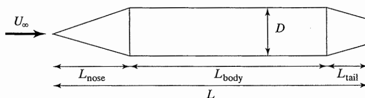
Figure 5.21 Geometry of a fuselage with circular cross sections.
