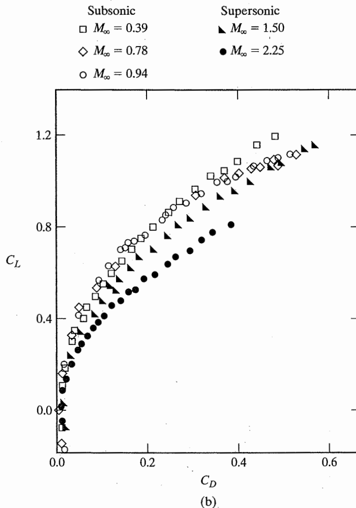
Figure 9.19 (continued) (b) drag polar.
