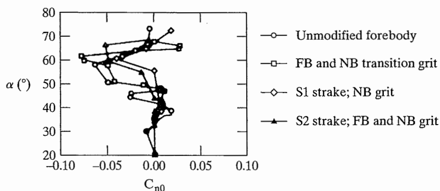
Figure 7.57 Variation of yawing moment asymmetry with angle of attack for an X-31 for a 1-g maneuver. [Taken from Cobleigh (1994).]
