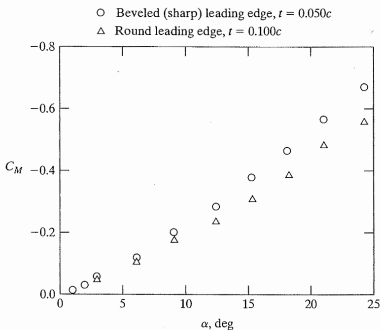
Figure 7.48 Moment coefficient (about the apex) for thin, flat delta wings for which AR = 1.5 , Re_c = 6 \times 10^6 . [Data from Bartlett and Vidal (1955).]
