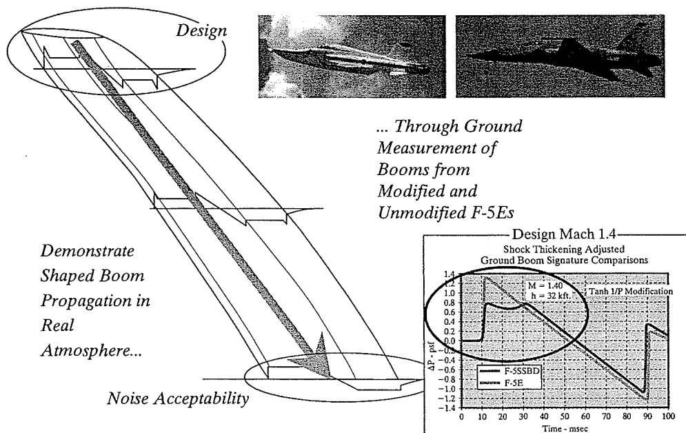
Figure 11.36 Impact of forebody shaping on N-wave production for the F-5E [From Pawlowski et al. (2005).]
