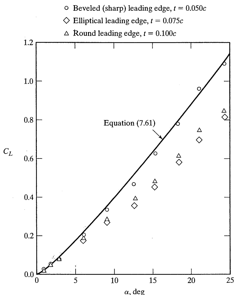
Figure 7.45 Effect of the leading-edge shape on the measured lift coefficient for thin, flat delta wings for which AR = 1.5 , Re_c = 6 \times 10^6 . [Data from Bartlett and Vidal (1955).]
