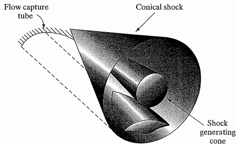
Figure 12.24 Derivation of waverider configurations from a conical flow field.
