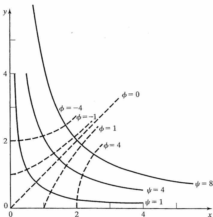
Figure 3.8 Equipotential lines and streamlines for Example 3.3.
