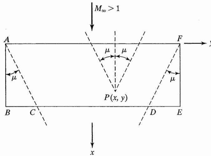
Figure 11.2 Rectangular wing in a supersonic stream.
