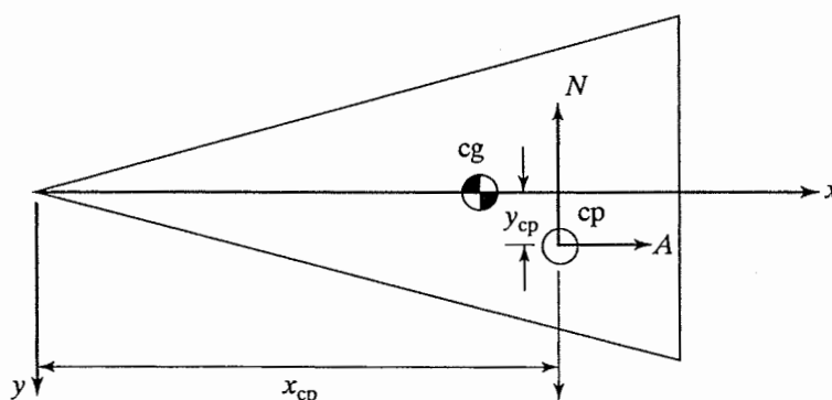
Figure 12.17 Aerodynamic forces acting at the center of pressure as effectively producing the aerodynamic pitching moment.
