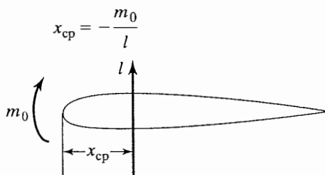
Figure 6.7 Center of pressure for a thin, cambered airfoil.
