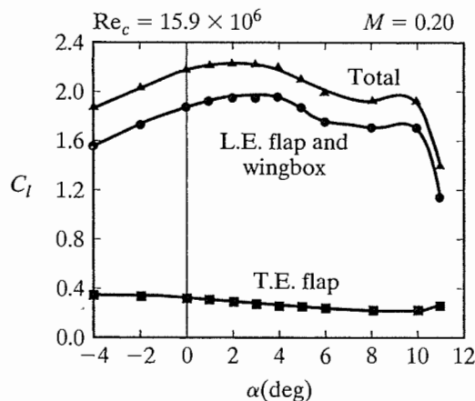
Figure 6.32 Total and component lift curves, \delta_n = 34^\circ , \delta_f = 35^\circ , \delta_s = 22.94^\circ . [Taken from Hobbs (1996).]
