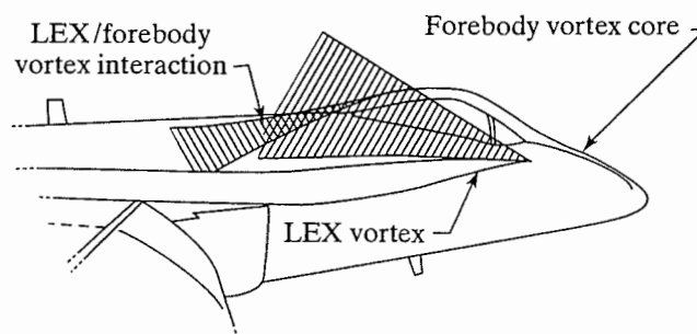
Figure 7.59 Wingtip view of forebody vortex system. [Taken from Del Frate and Zuniga (1990).]
