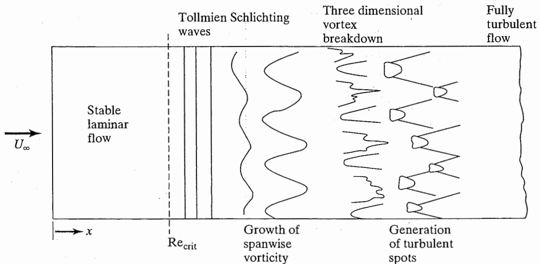
Figure 4.12 Idealized sketch of the transition process on a flat plate. (Based on the sketch from Viscous Fluid Flow by F. M. White. Copyright © 1974 by McGraw-Hill Book Company.)
