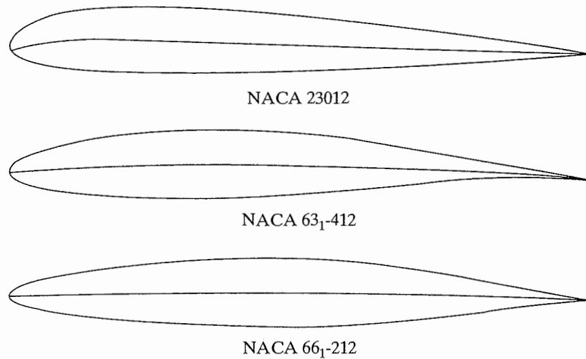
Figure 6.12 Shapes of two NACA laminar-flow airfoil sections compared with the NACA 23012 airfoil section. [Loftin (1985).]
