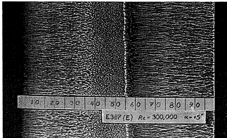
Figure 6.16 Laminar separation bubble on an airfoil shown by surface oil flow where separation and reattachment are visible. [Selig (2003).]
