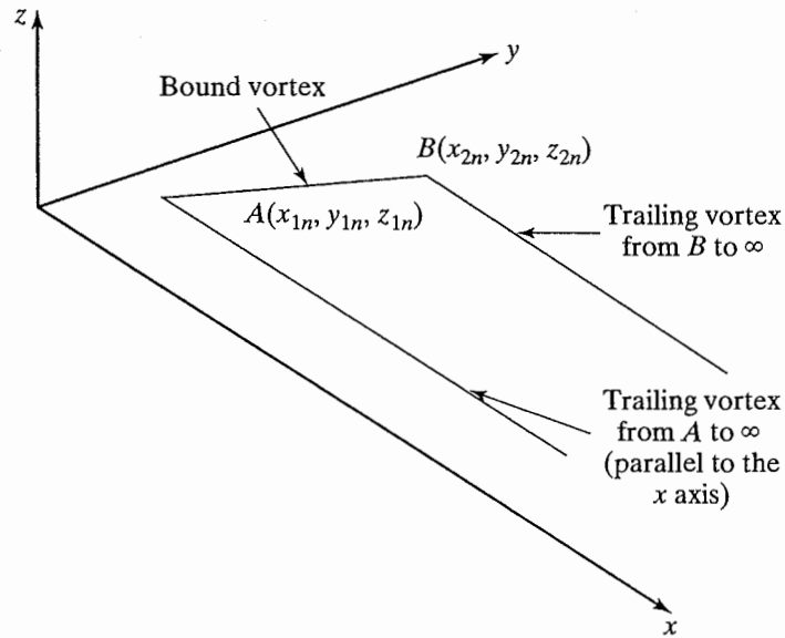
Figure 7.28 “Typical” horseshoe vortex.
