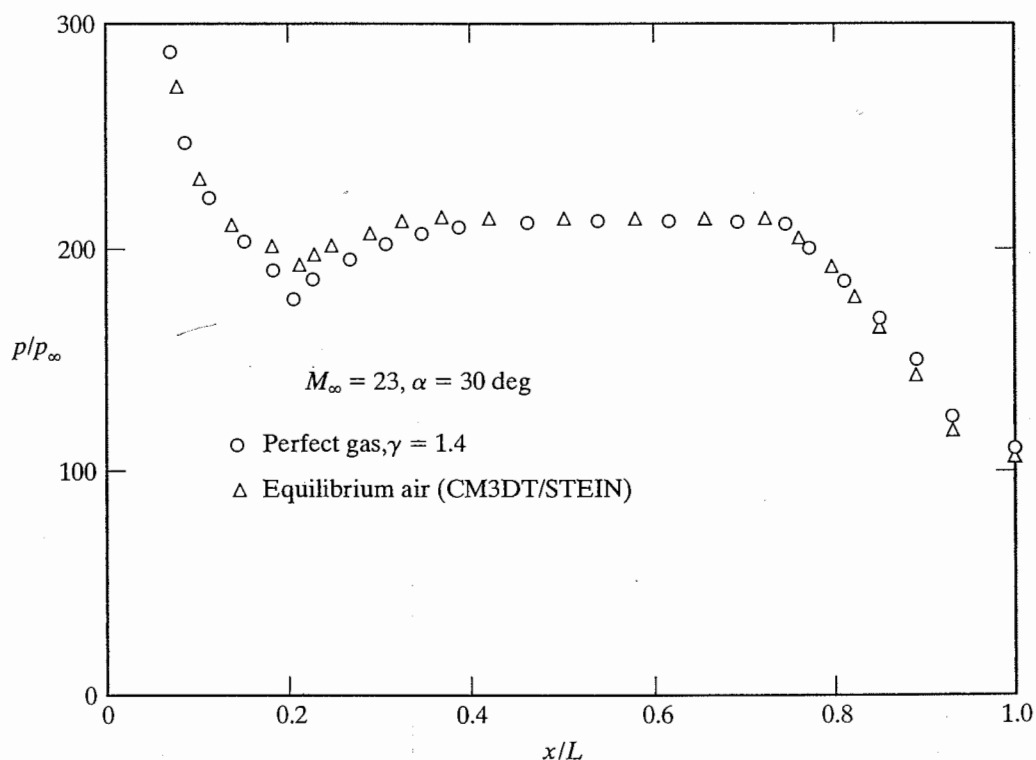
Figure 12.36 Comparison of perfect-gas and equilibrium-air calculations of the windward pitch-plane pressure distribution for the Space Shuttle Orbiter at \alpha = 30^\circ . [From Maus et al. (1984).]
