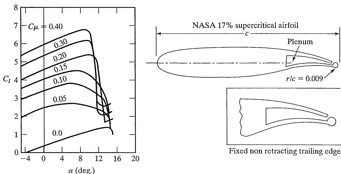
Figure 13.17 Sectional lift characteristics for a 17% thick CCW/-supercritical airfoil. [From Englar (1987).]
