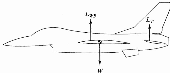
Figure 5.3 Moment balance to trim an aircraft.
