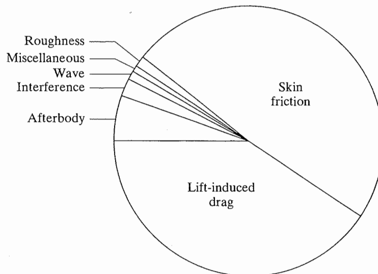
Figure 5.29 Contributions of different drag sources for a typical transport aircraft. [From Thomas (1985).]
