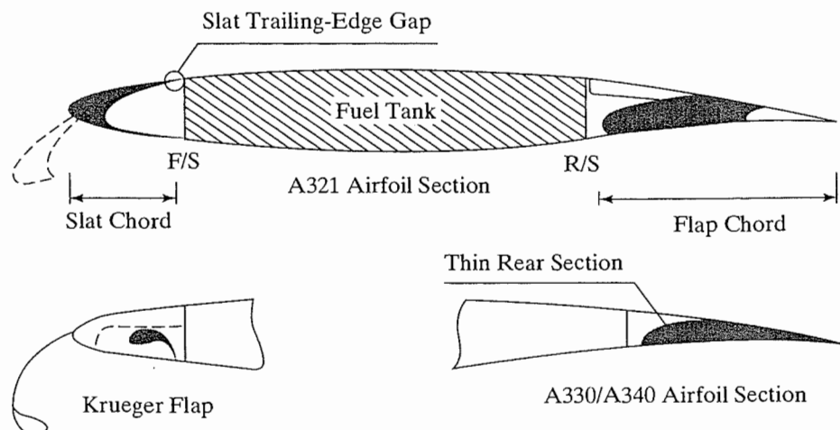
Figure 6.25 General constraints on the design of high-lift multi-element airfoil sections. [Taken from Flaig and Hilbig (1993).]
