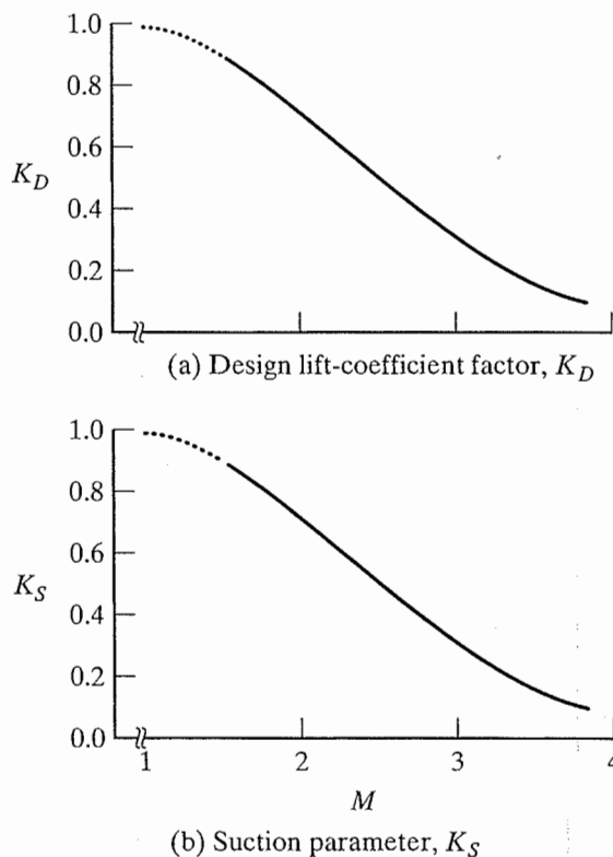
Figure 11.33 Empirical method factors used to select the optimum design lift coefficients and to predict achievable suction parameters. [Taken from Carlson and Mann (1992).]
