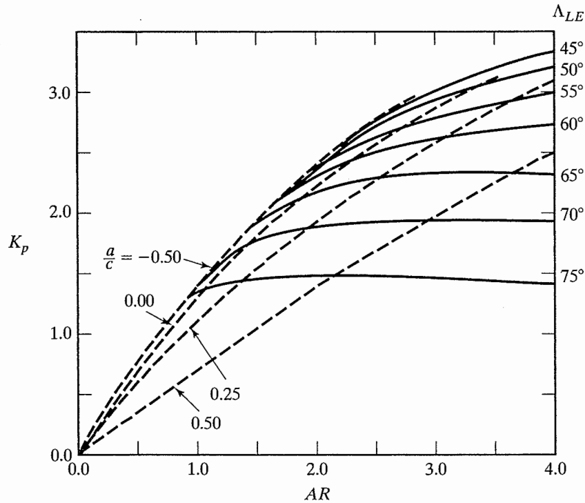
Figure 7.42 Variation of potential-flow lift constant with planform parameters. [Taken from Pollhamus (1971b).]
