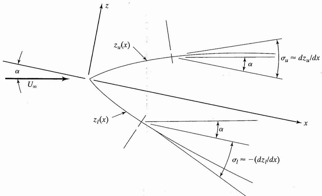
Figure 10.3 Detailed sketch of an airfoil section.
