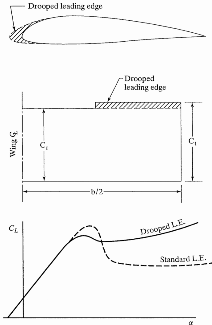
Figure 7.20 Drooped leading-edge characteristic. [Taken from Anderson, Corda, and Van Wie (1980).]
