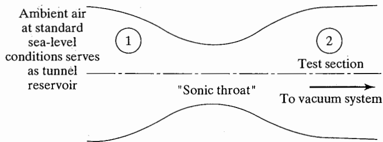
Figure 8.4 Indraft, supersonic wind tunnel.
