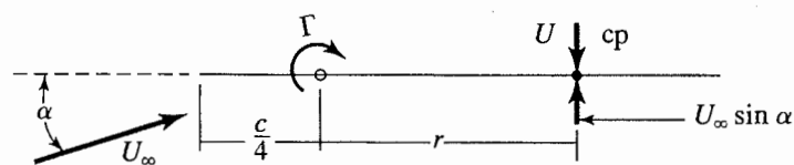
Figure 7.26 Planar airfoil section indicating location of control point where flow is parallel to the surface.
