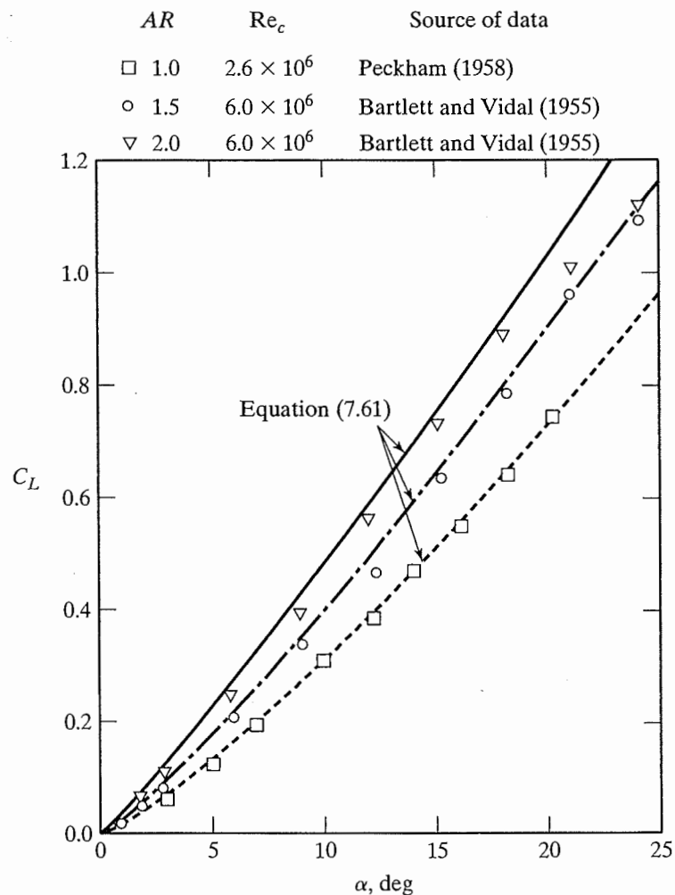
Figure 7.44 Comparison of the calculated and the experimental lift coefficients for thin, flat delta wings with sharp leading edges.
