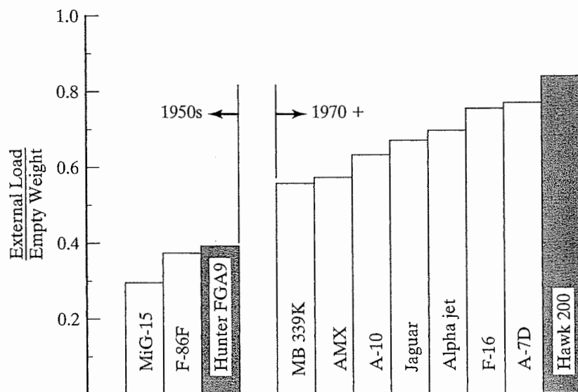
Figure 13.40 Capability of aircraft to carry stores externally. [As taken from Whitford (1991).]
