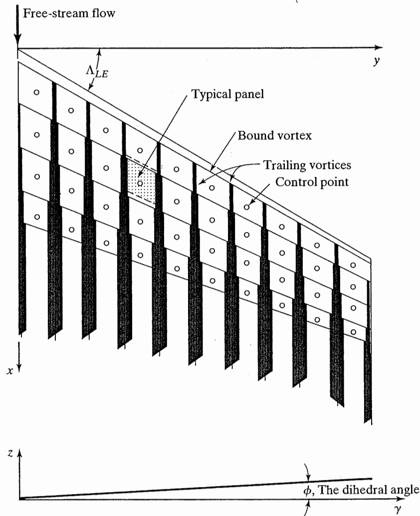
Figure 7.24 Coordinate system, elemental panels, and horseshoe vortices for a typical wing planform in the vortex lattice method.
