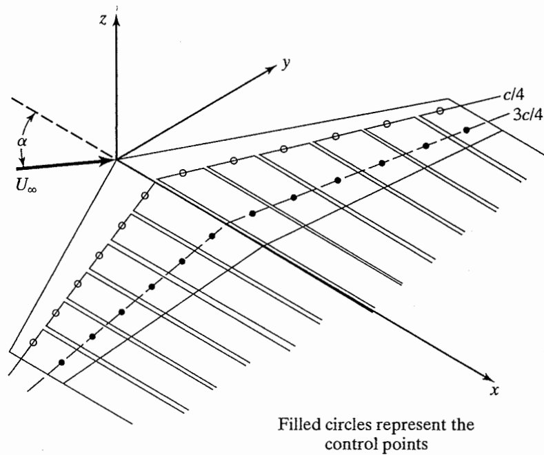
Figure 7.25 Distributed horseshoe vortices representing the lifting flow field over a swept wing.
