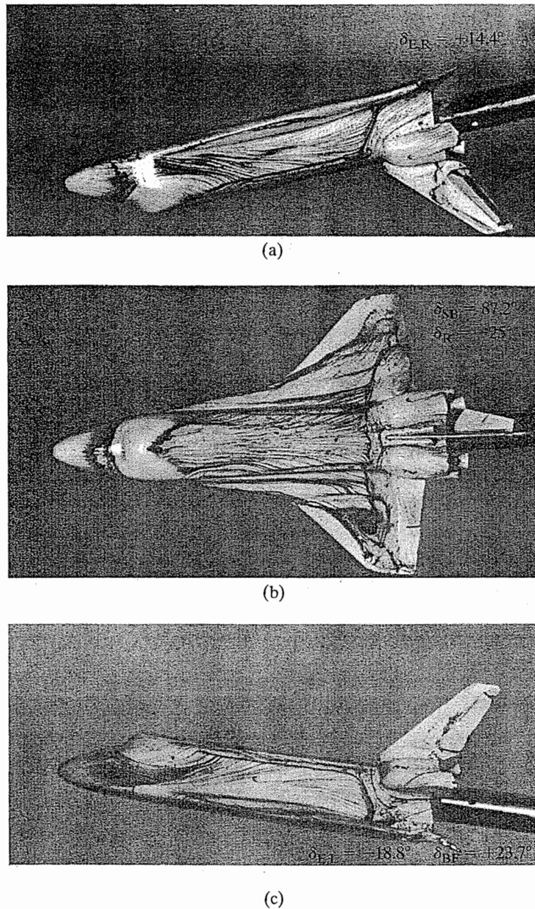
Figure 11.46 Oil flow patterns for Space Shuttle Orbiter at M_\infty = 1.25 and \alpha = 10^\circ : (a) view of right side; (b) top view; (c) view of left side. (Courtesy of Johnson Space Center, NASA.)
