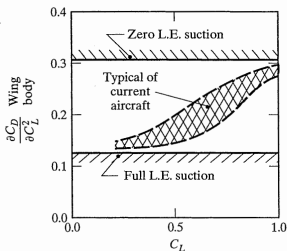
Figure 7.39 Typical variation of drag-due-to-lift parameter; aspect ratio = 2.5; subsonic speeds. [Taken from Henderson (1966).]
