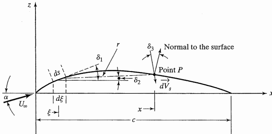
Figure 6.5 Thin-airfoil geometry parameters.
