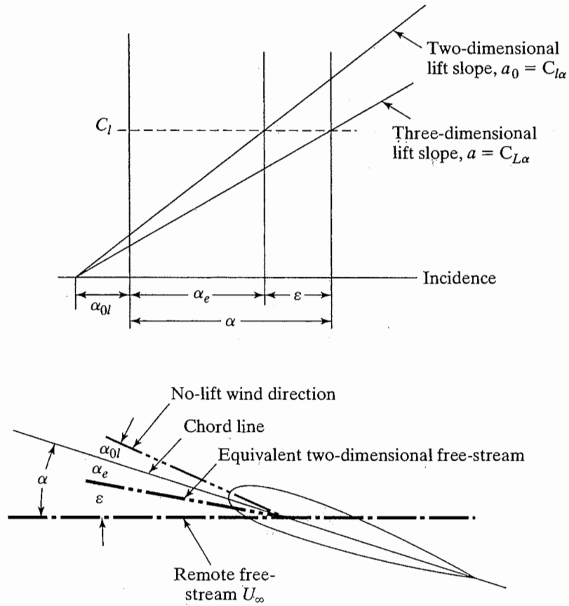
Figure 7.12 Nomenclature for wing/airfoil lift.
