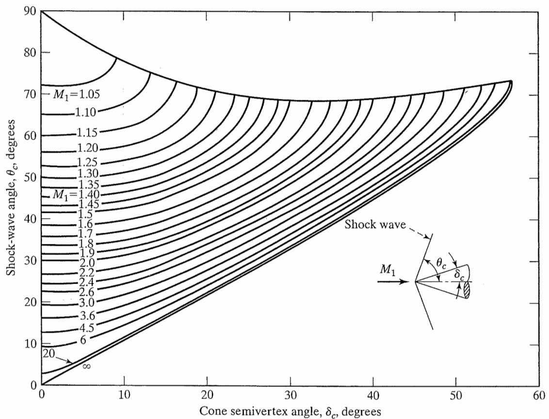
Figure 8.15 Variations of shock-wave parameters with cone semivertex angle for various upstream Mach numbers, \gamma = 1.4 : (a) shock-wave angle.
