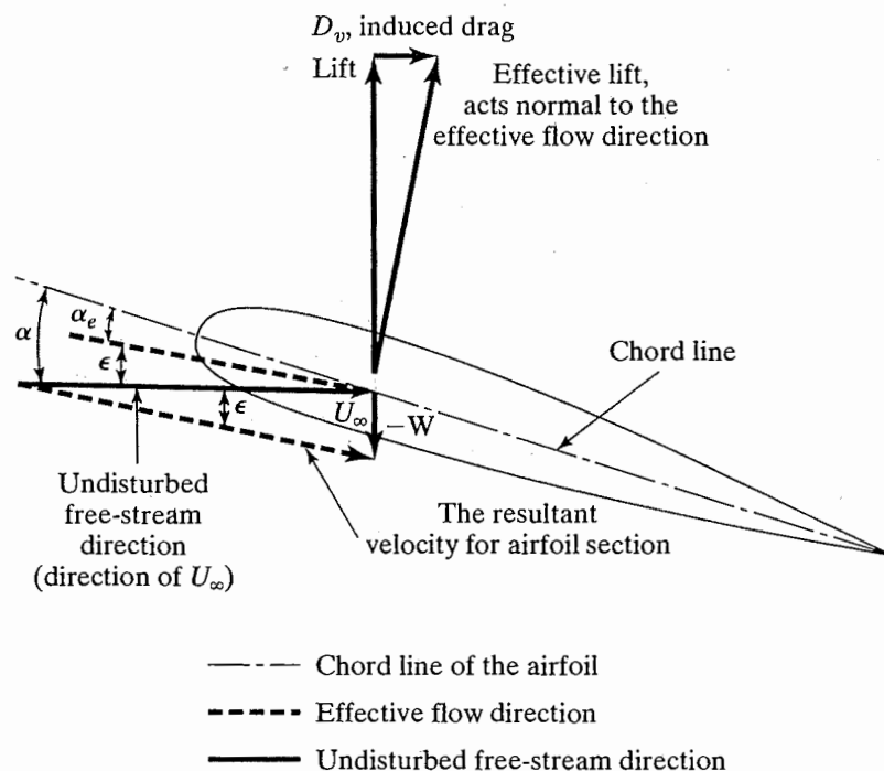
Figure 7.6 Induced flow.
