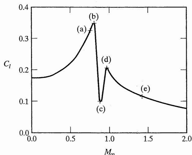
Figure 9.7 Section lift coefficient as a function of Mach number to illustrate the effect of compressibility. [From Farren (1956).] Refer to Fig. 9.8 for the flow fields corresponding to the lettered points on this graph.
