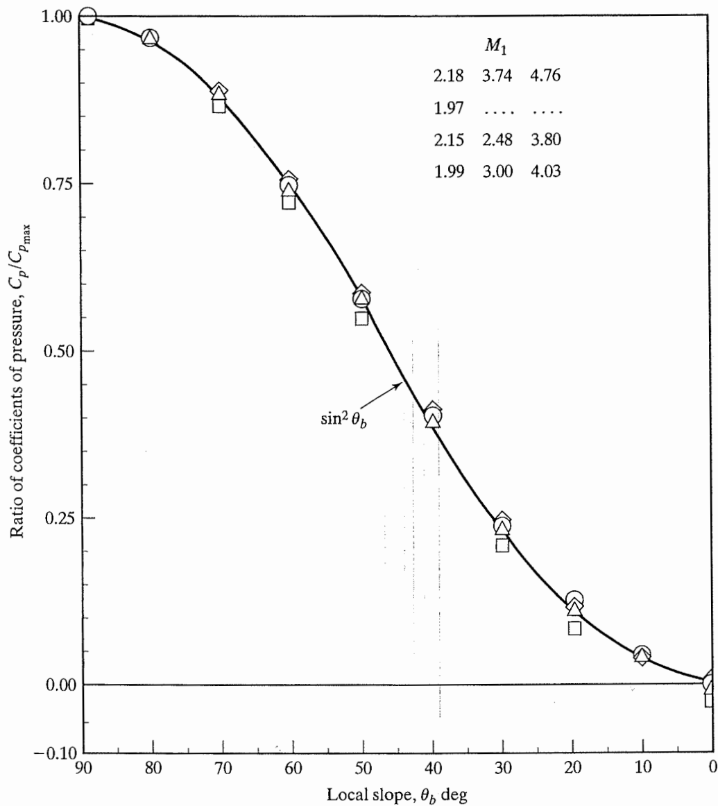
Figure 12.9 Correlation between C_p/C_{p,\max} ratio and local body slope. [From Isaacson and Jones (1968).]
