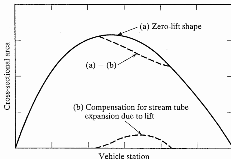
Figure 9.30 Second-order area rule considerations. [From Whitcomb (1976).]
