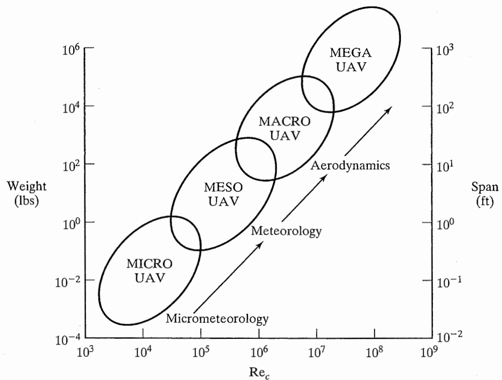
Figure 7.60 Classification of UAVs by weight, span, and Reynolds number. [From Wood (2002).]
