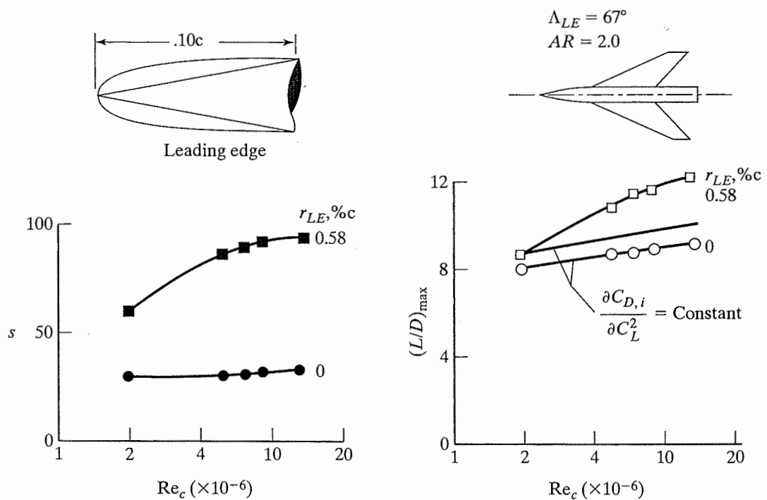
Figure 7.38 The effect of the leading-edge shape, C_{L,opt} , M < 0.30 . [Taken from Henderson (1966).]
