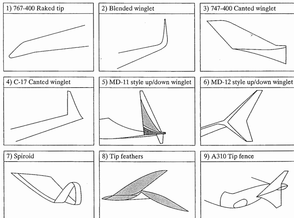
Figure 13.27 An assortment of wing-tip device configurations. [From McLean (2005).]
