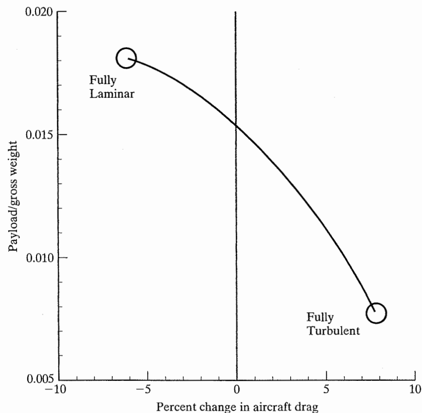
Figure 12.39 Effect of transition on NASP design.
