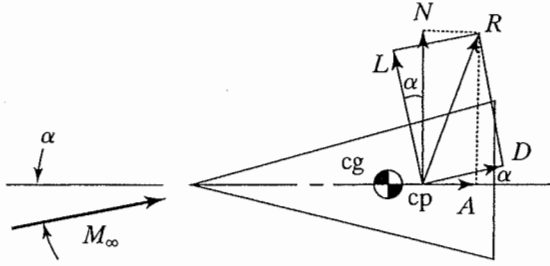
Figure 12.16 Resolving the forces acting on a vehicle.
