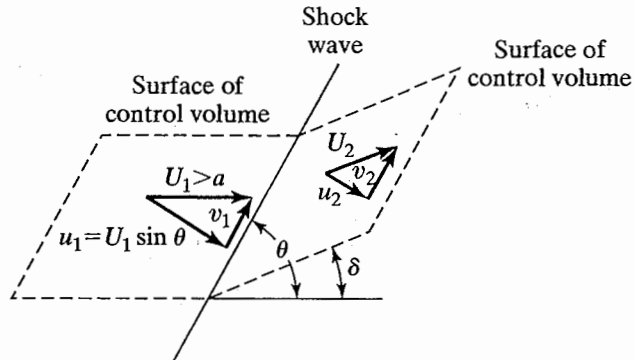
Figure 8.11 Control volume for analysis of flow through an oblique shock wave.
