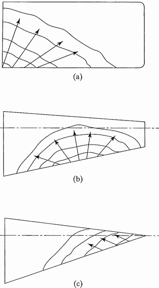
Figure 7.18 Typical stall patterns: (a) rectangular wing, \lambda = 1.0 ; (b) moderately tapered wing, \lambda = 0.4 ; (c) pointed wing, \lambda = 0.0 .
