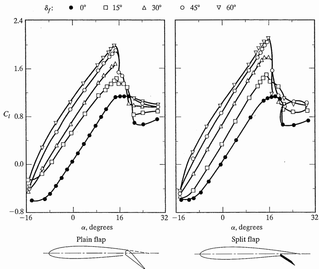
Figure 13.9 Effect of flap angle on the sectional lift coefficient for a NACA 23012 airfoil section, Re_c = 6 \times 10^5 . [Data from Schlichting and Truckenbrodt (1969).]
