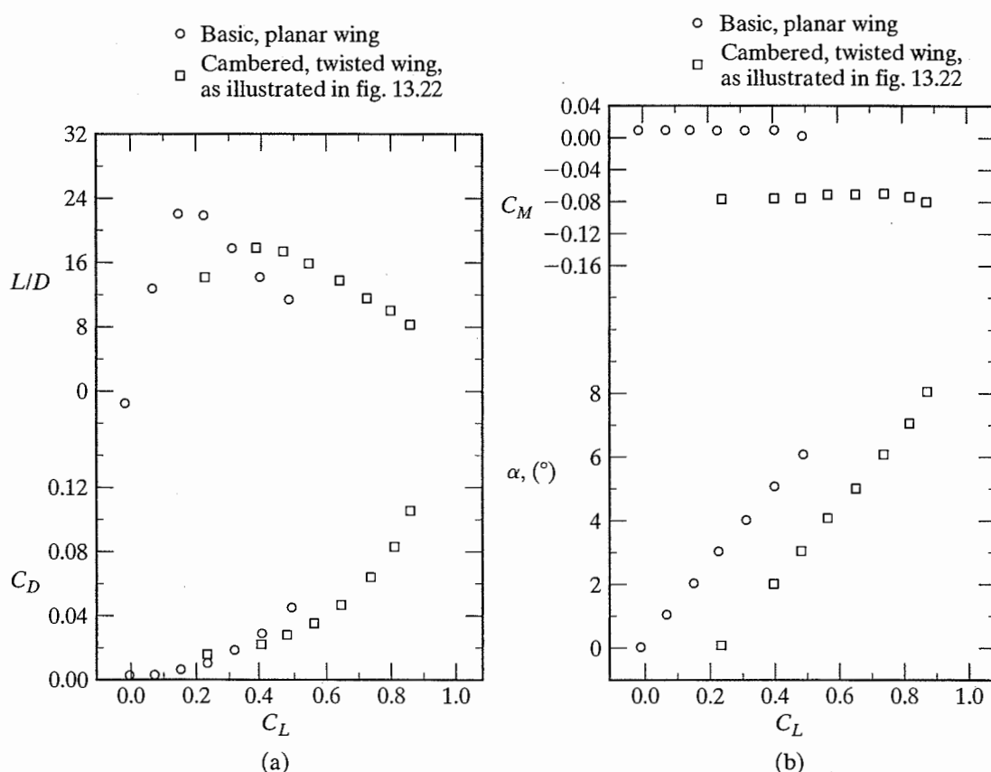
Figure 13.23 Effect of twist and camber on the longitudinal aerodynamic characteristics M_\infty = 0.80 , Re_c = 7.4 \times 10^6 : (a) lift-to-drag ratio and the drag polar, (b) pitching moment and lift coefficients. [From Ferris (1977).]
