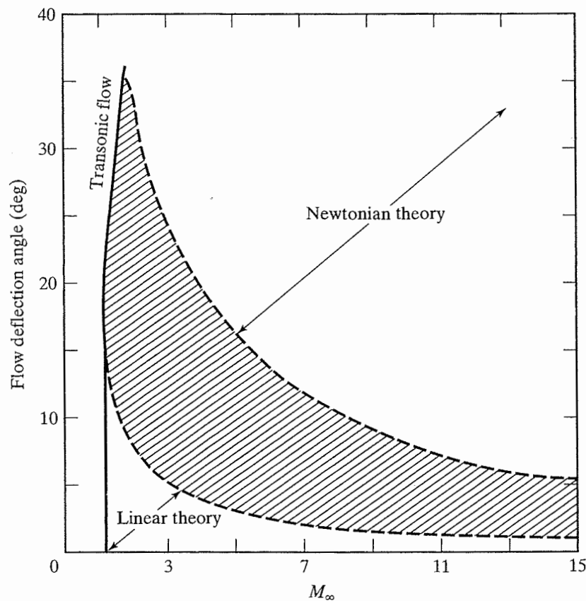
Figure 12.2 Regions of applicability of inviscid flow theories for the surface pressure on a sharp cone. [From Marconi, et al. (1976).]
