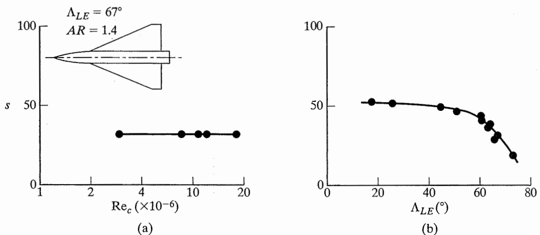
Figure 7.36 The variation of the effective leading-edge suction ( s ) as (a) a function of the Reynolds number and (b) of the leading-edge sweep angle for a wing with a sharp leading edge, C_{L,opt} , and M < 0.30 . [Taken from Henderson (1966).]
