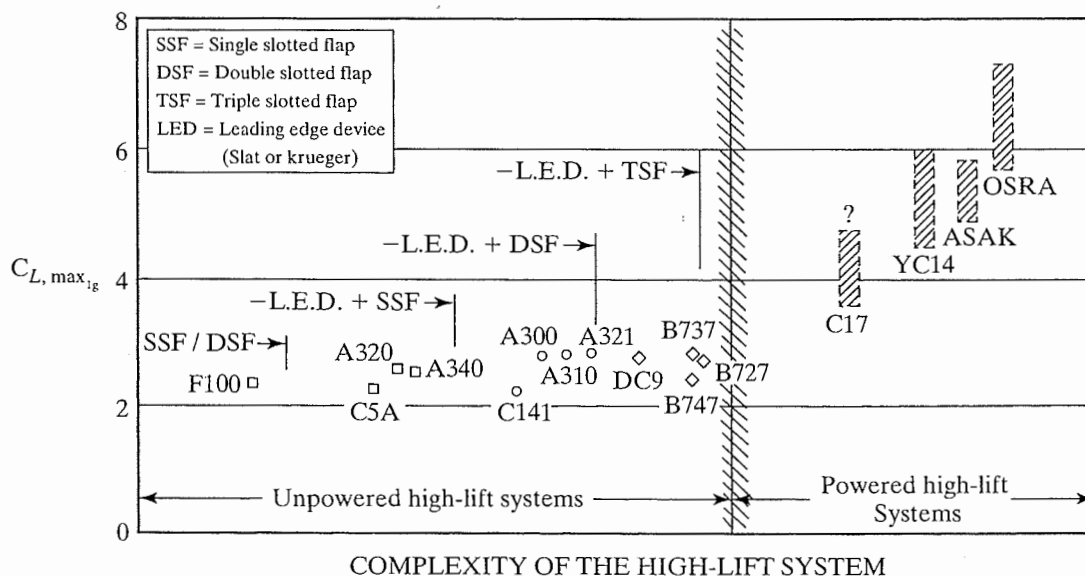
Figure 6.26 The maximum lift coefficient as a function of the complexity of the high-lift system. [Taken from Flaig and Hilbig (1993).]
