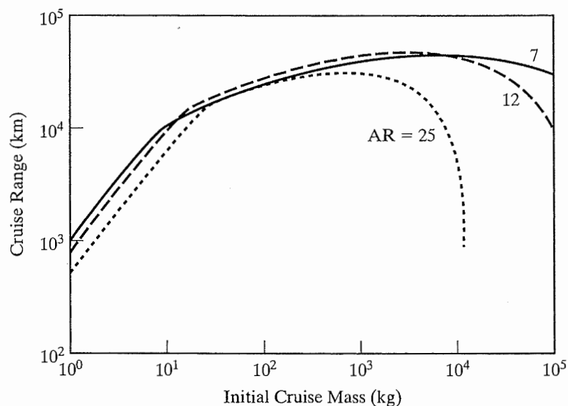
Figure 7.61 The influence of wing aspect ratio on aircraft range as a function of mass (all other factors kept constant). [From Drela et al. (2003).]
