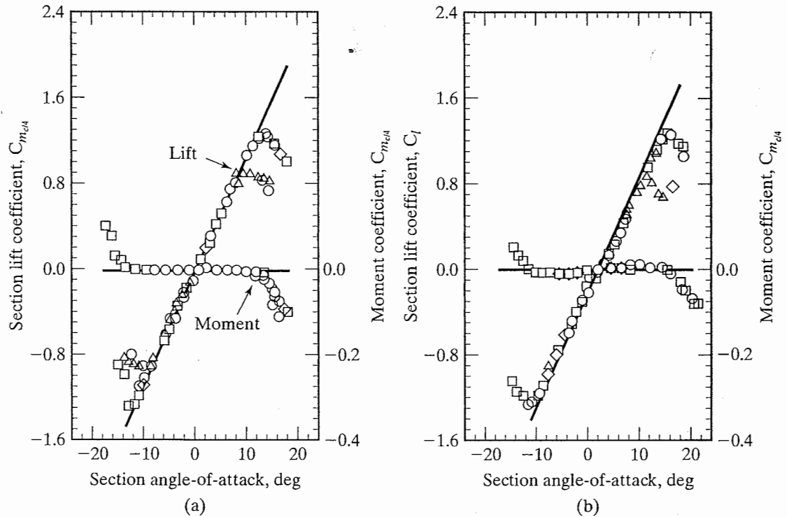
Figure 6.6 Comparison of the aerodynamic coefficients calculated using thin-airfoil theory for symmetric airfoils: (a) NACA 0009 wing section; (b) NACA 0012-64 wing section. [Data from Abbott and von Doenhoff (1949)].
