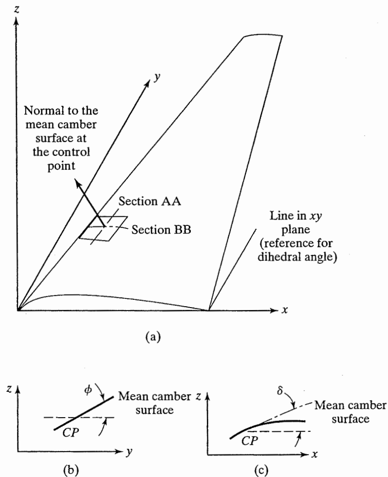
Figure 7.30 Nomenclature for the tangency requirement: (a) normal to element of the mean camber surface; (b) section AA; (c) section BB.
