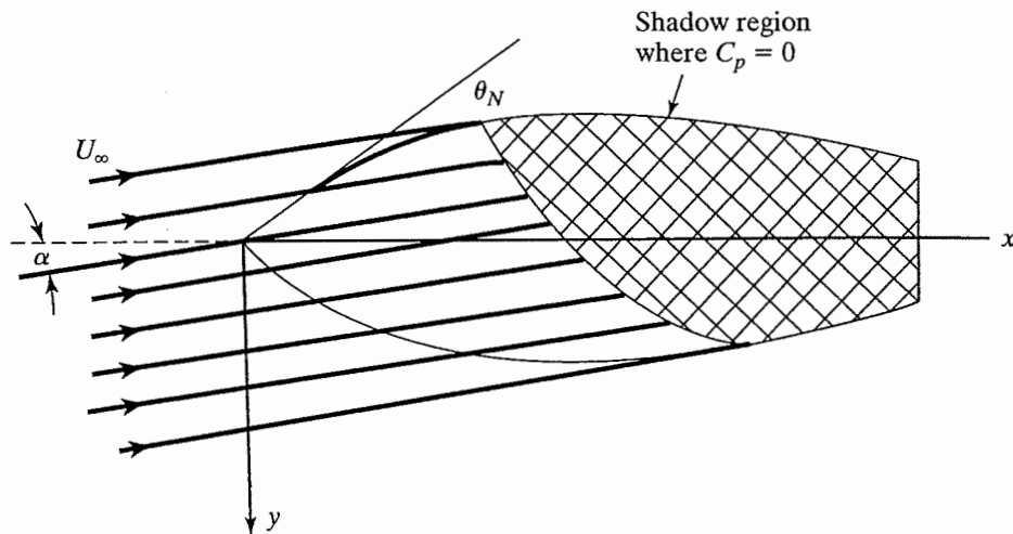
Figure 12.14 Region where C_p = 0 , that is, that portion of the body which lies in the “shadow of the free stream.”
