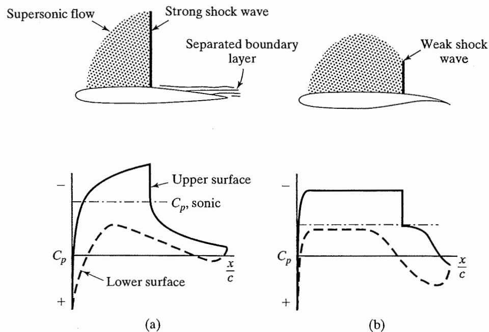
Figure 9.16 Comparison of transonic flow over a NACA 64A series airfoil with that over a “supercritical” airfoil section: (a) NACA 64A series, M = 0.72 ; (b) supercritical airfoil, M = 0.80 . [From Ayers (1972).]
