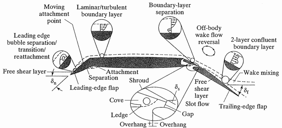
Figure 6.31 Sketch of the flow field for a military airfoil in a high-lift configuration. [A composite developed from information presented in Kern (1996) and Hobbs (1996).]
