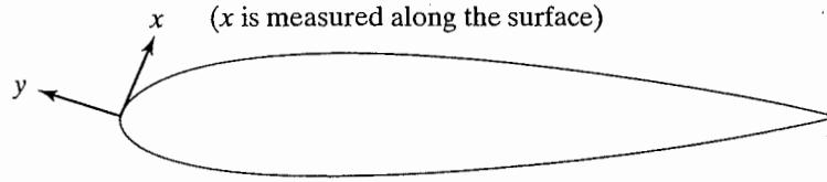
Figure 4.1 Coordinate system for the boundary-layer equations.
