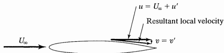
Figure 9.2 Velocity components for subsonic, compressible flow past a thin airfoil at a small angle of attack.
