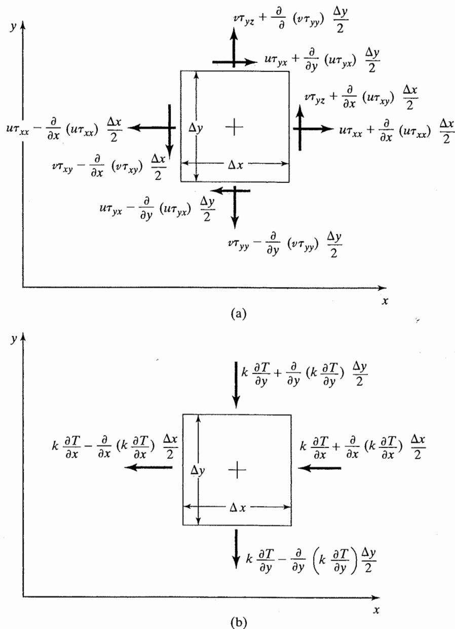
Figure 2.15 Heat-transfer and flow-work terms for the energy equation for a two-dimensional fluid element: (a) work done by stresses acting on a two-dimensional element; (b) heat transfer to a two-dimensional element.
