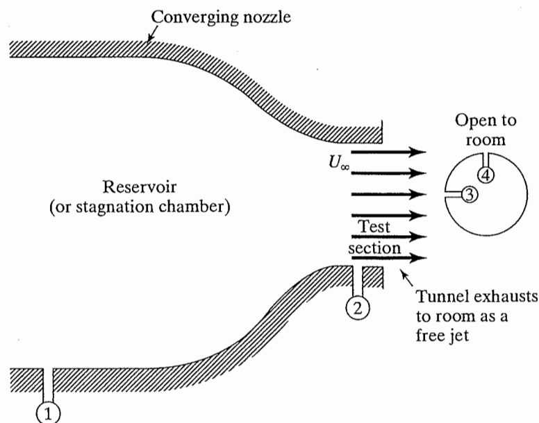
Figure 3.3 Open test-section wind tunnel used in Example 3.2.
