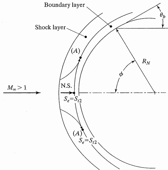
Figure 12.29 Sketch of the normal shock/isentropic expansion flow model for hypersonic flow over a blunt body. The air at the edge of the boundary layer at point A has passed through the (nearly) normal part of the shock wave. Thus, the entropy of the air particles at the edge of the boundary layer ( S_e ) is essentially equal to S_{t2} at all stations. In essence, the air has passed through the normal part of the shock wave (NS) and has undergone an isentropic expansion (IE) to the local pressures.
