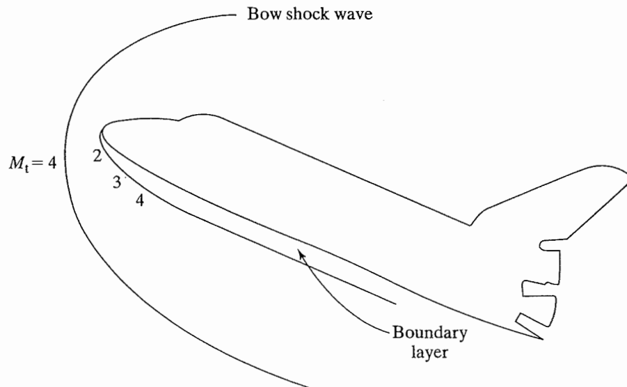
Figure 8.5 Shuttle flow field for Example 8.2.
