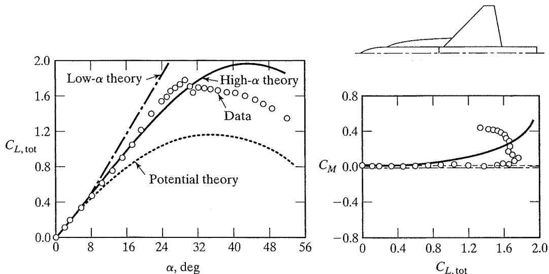
Figure 7.51 Predicted and measured C_{L,tot} and C_M for strake/wing configuration at M_\infty = 0.2 . [Taken from Lamar and Frink (1982).]
