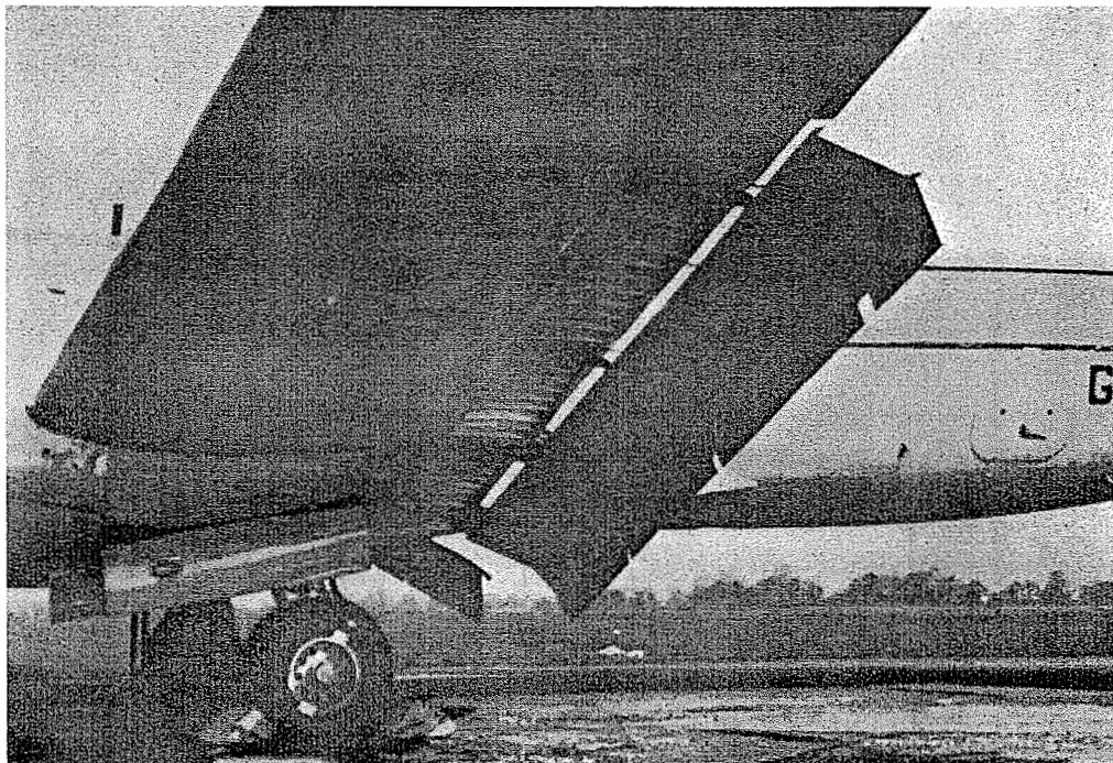
Figure 13.2 Multielement, high-lift configurations: (a) Fowler flap; (b) double-slotted flap; (c) leading-edge slat, Krueger leading-edge flap, spoiler, and triple-slotted flaps (representative of Boeing 727 wing section). (d) Fowler flaps on the HS 748. (Courtesy of British Aerospace.)
