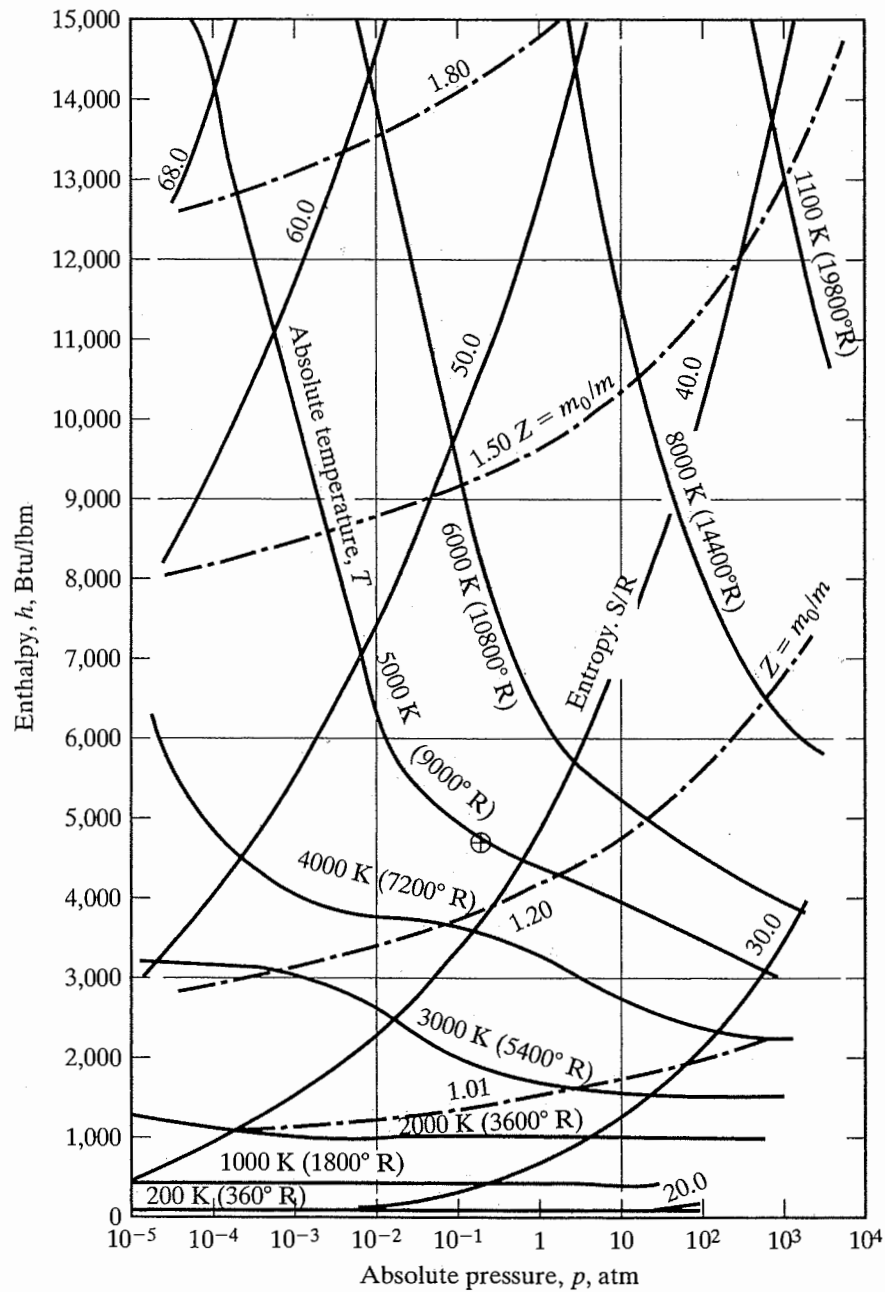
Figure 12.5 Thermodynamic properties of air in chemical equilibrium. [From Moeckel and Weston (1958).]
