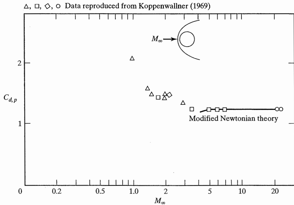
Figure 12.11 Pressure drag of a right circular cylinder as a function of Mach number. [From Koppenwallner (1969).]
