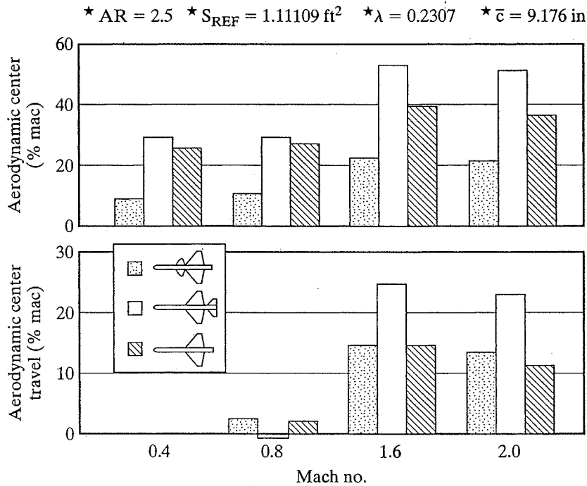
Figure 13.48 Variation of aerodynamic center with Mach number for canard, tail, and tailless arrangements with the 44-degree sweep trapezoidal wing. [From Nicholas et al. (1984).]
