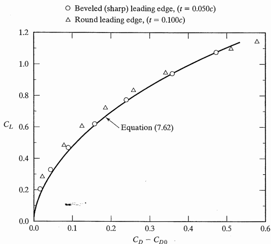
Figure 7.47 Drag correlation for thin, flat delta wings for which AR = 1.5 , Re_c = 6 \times 10^6 . [Data from Bartlett and Vidal (1955).]
