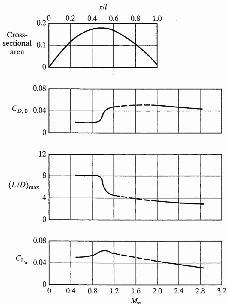
Figure 9.29 Area distribution and various aerodynamic parameters for a swept-wing cruise missile. [From Spearman and Collins (1972).]
