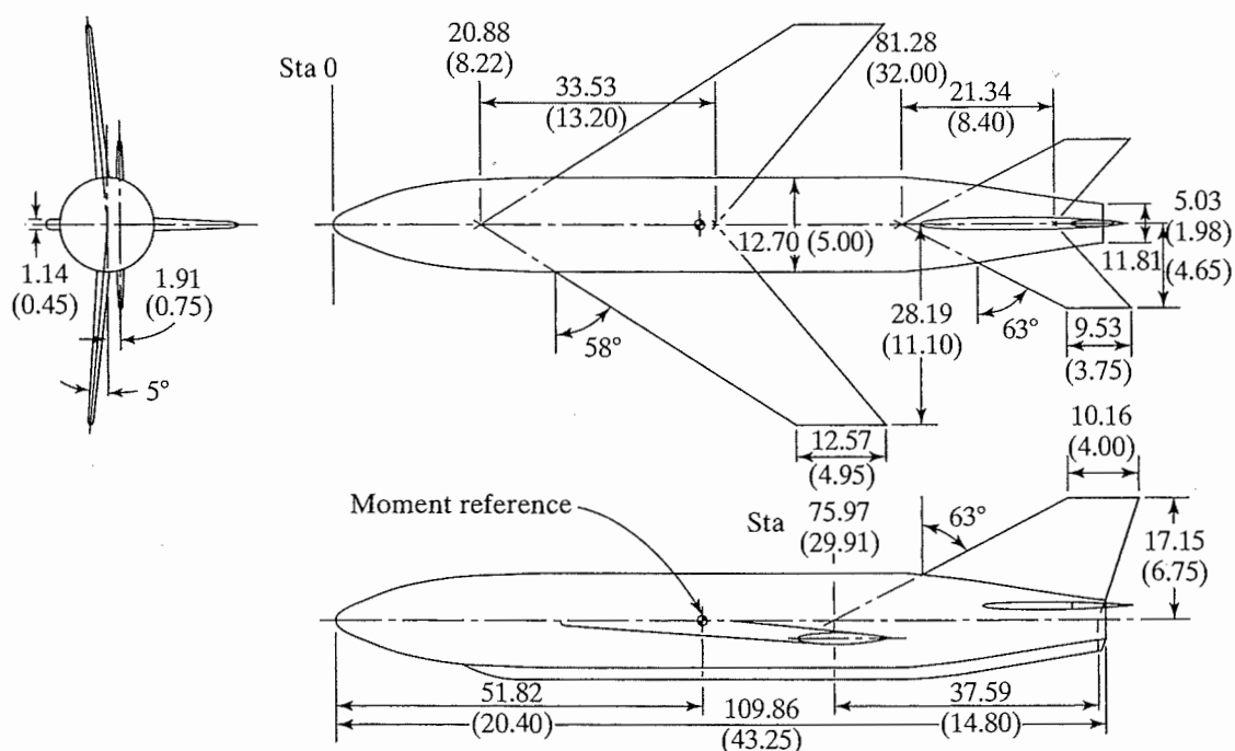
Figure 9.28 Details of a model of a swept-wing cruise missile. Linear dimensions are in centimeters (inches). [From Spearman and Collins (1972).]
