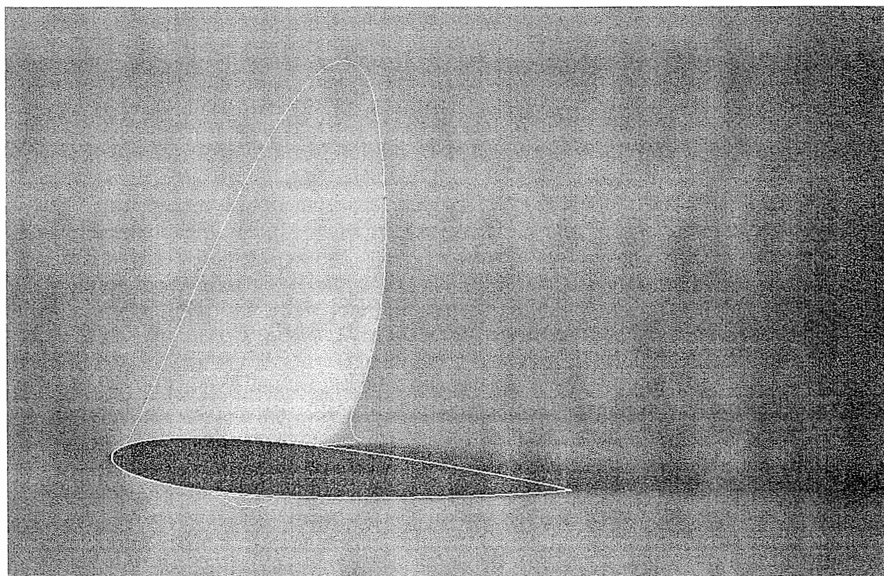
Figure 9.10 Constant-density contours for a NACA 0012 airfoil in a Mach 0.8 stream at \alpha = 3^\circ . [As provided by Forsythe and Blake (2000).]
