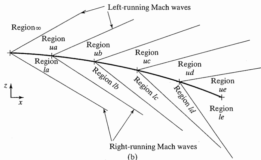
Figure 8.9 Mach waves for supersonic flow past a thin airfoil: (a) airfoil section; (b) wave pattern.
