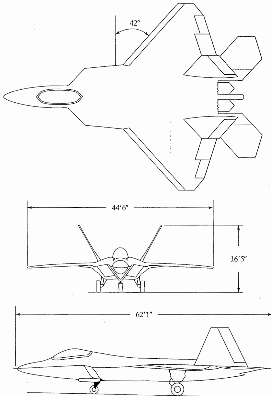
Figure 13.51 External configuration of the F-22. [As taken from Mullin (1992).]
