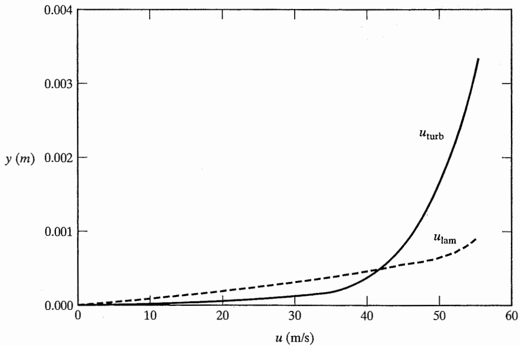
Figure 4.20 Velocity profiles for Example 4.4.
