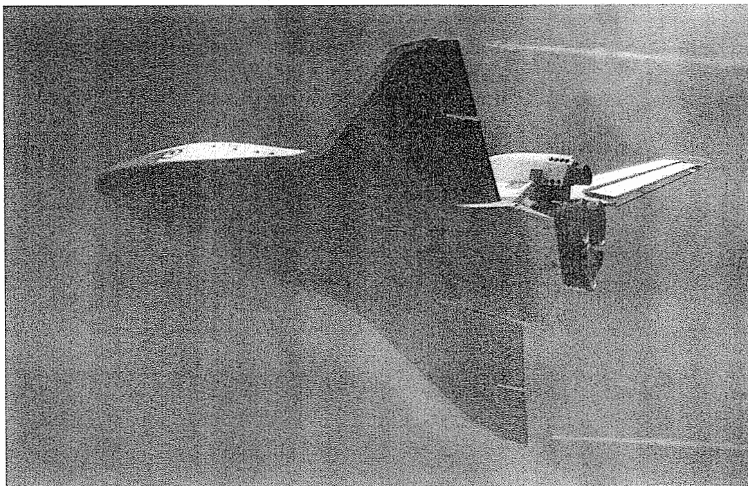
Figure 7.3 Condensation marks the wing-tip vortices of the Space Shuttle Orbiter Columbia . (Courtesy NASA.)
