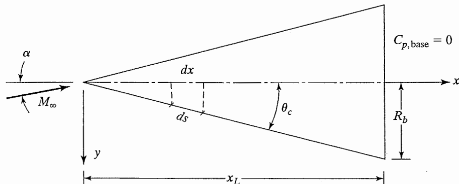
Figure 12.15 Nomenclature for hypersonic flow past a sharp cone.
