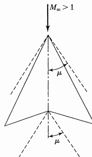
Figure 11.5 Arrow wing with a subsonic leading edge and a supersonic trailing edge.
