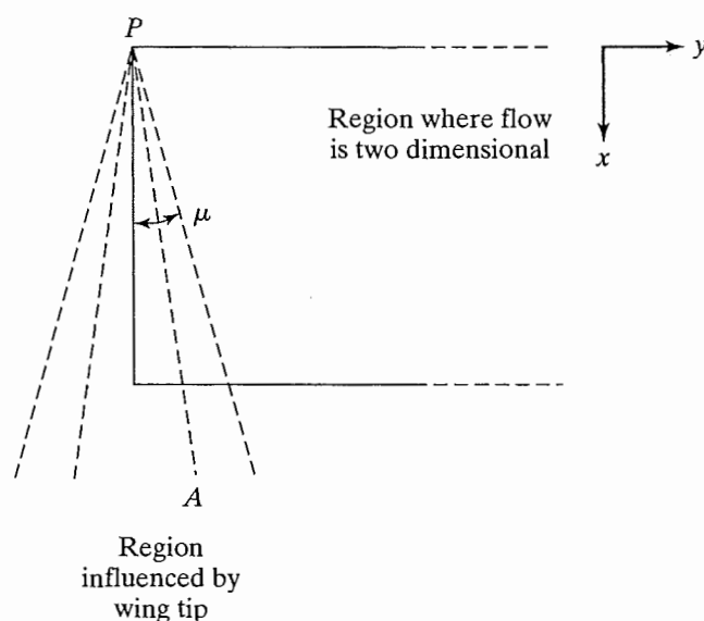
Figure 11.7 In a conical flow, properties are invariant along rays emanating from a point.
