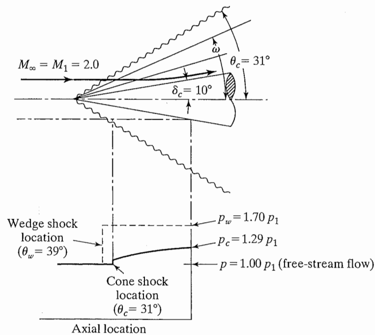
Figure 8.14 Supersonic flow past a sharp cone at zero angle of attack.
