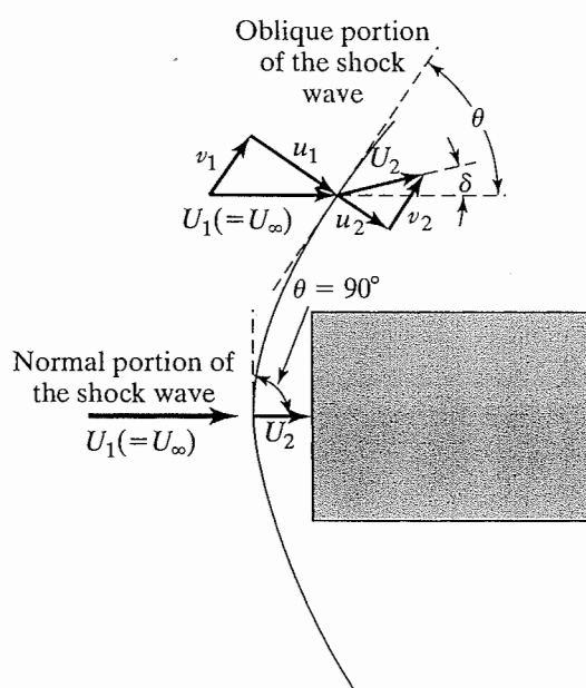
Figure 8.10 Curved shock wave illustrating nomenclature for normal shock wave and for oblique shock wave.
