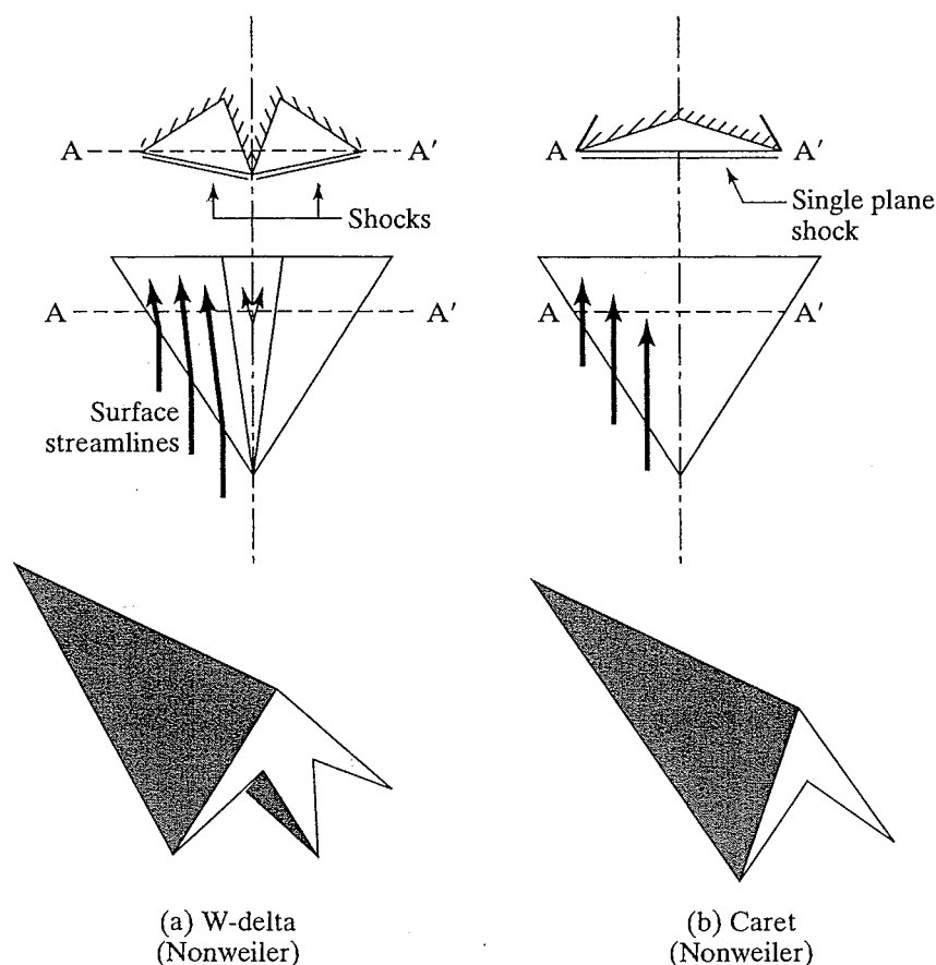
Figure 12.20 Shapes of all-wing delta planforms amenable to treatment by exact shock-wave theory, as proposed by Nonweiler (1959).
