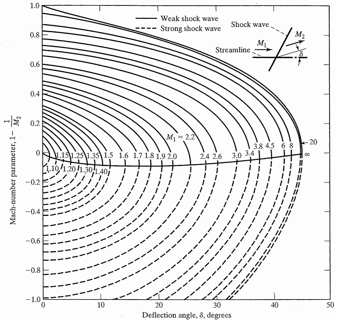
Figure 8.12 (continued) (c) downstream Mach number.
