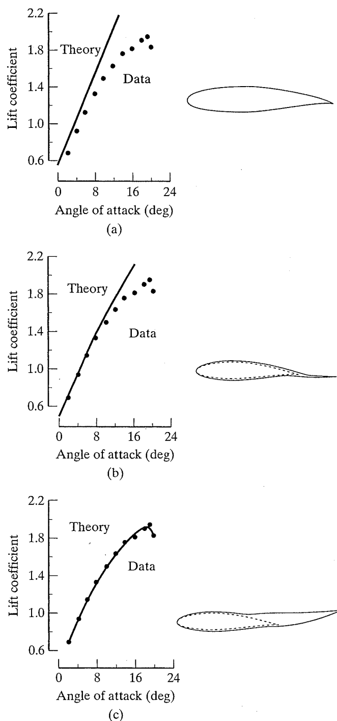
Figure 6.11 Relative importance of separation effects: (a) analysis of geometry alone; (b) analysis with boundary layer modeled; (c) analysis with boundary layer and separated wake modeled. [From Henderson (1978).]
