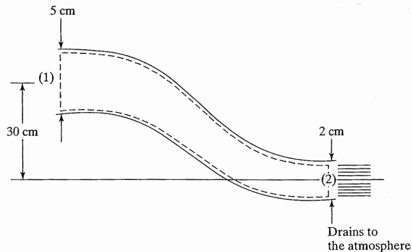
Figure 2.17 Pipe flow for Example 2.5.
