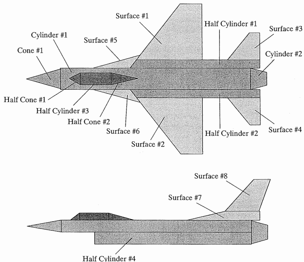
Figure 5.24 F-16 geometry approximated by simple shapes. [From Brandt et al. (2004).]
