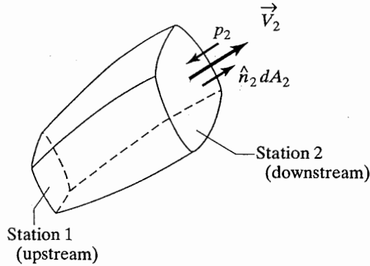
Figure 2.16 Streamtube for derivation of equation (2.36).
