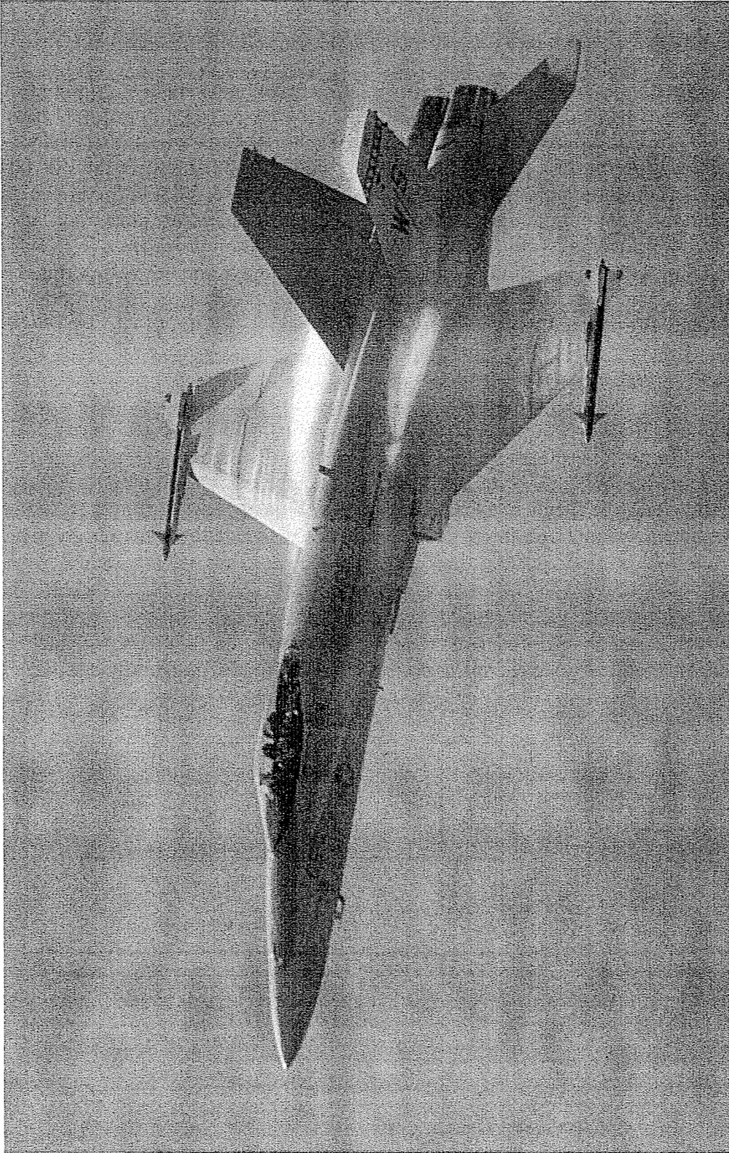
Figure 7.4 Concluded. (b) Streamwise vorticity from the F/A-18 Hornet wing leading edge during maneuver. (Copyrighted image reproduced courtesy of The Boeing Company.)
