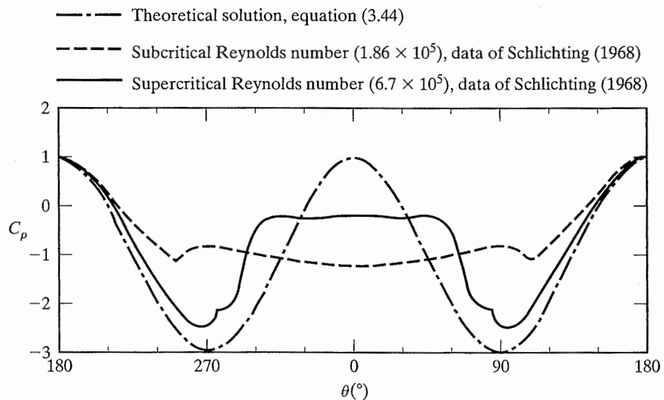
Figure 3.17 Theoretical pressure distribution around a circular cylinder, compared with data for a subcritical Reynolds number and that for a supercritical Reynolds number. [From Boundary Layer Theory by H. Schlichting (1968), used with permission of McGraw-Hill Book Company.]
