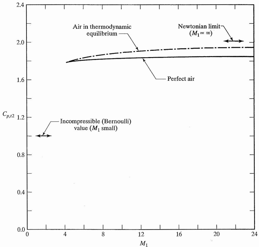
Figure 12.8 Pressure coefficient at the stagnation point of a sphere ( R_N = 0.3048 m) at an altitude of 45,721 m.
