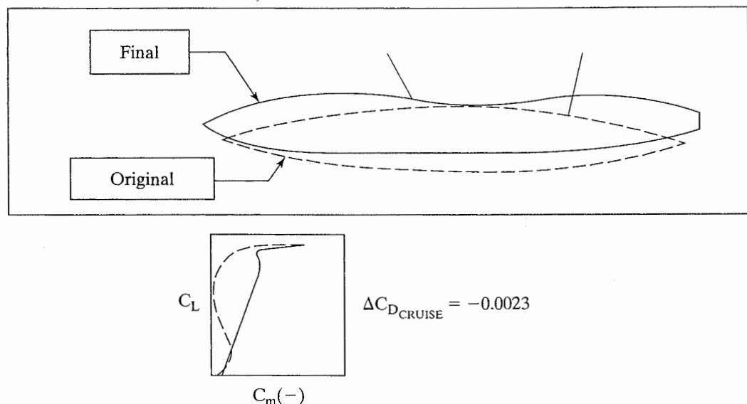
Figure 9.26 Application of area rule to the design of the tip tank for the F-5A/B aircraft. [From Stuart (1978).]
