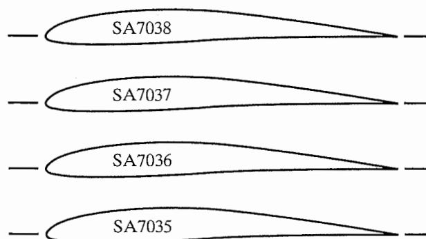
Figure 6.17 Candidate airfoils for radio controlled sailplanes. [Selig (2003)].
