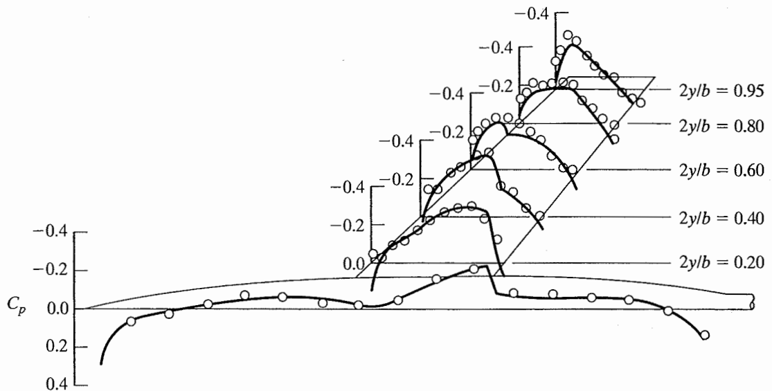
Figure 9.32 Comparison of computed and experimental pressure coefficients C_p for swept-wing/fuselage configuration, M_\infty = 0.93 ; \alpha = 0^\circ , \Lambda_{c/4} = 45^\circ , AR = 4 , \lambda = 0.6 , NACA 65A006 streamwise section. [From Bailey and Ballhaus (1975).]
