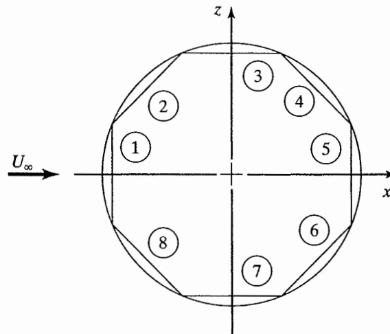
Figure 3.27 Representation of flow around a cylinder of unit radius by eight surface source panels.
