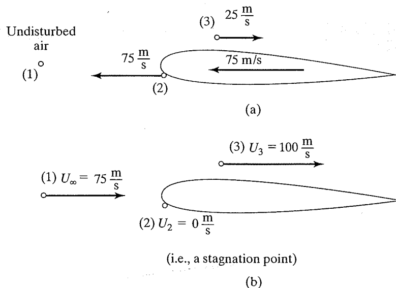
Figure 3.1 Velocity field around an airfoil: (a) ground-fixed coordinate system; (b) vehicle-fixed coordinate system.
