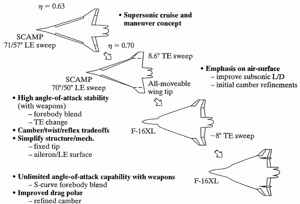
Figure 13.44 F-16XL configuration evolution. [From Hillaker (1982).]
