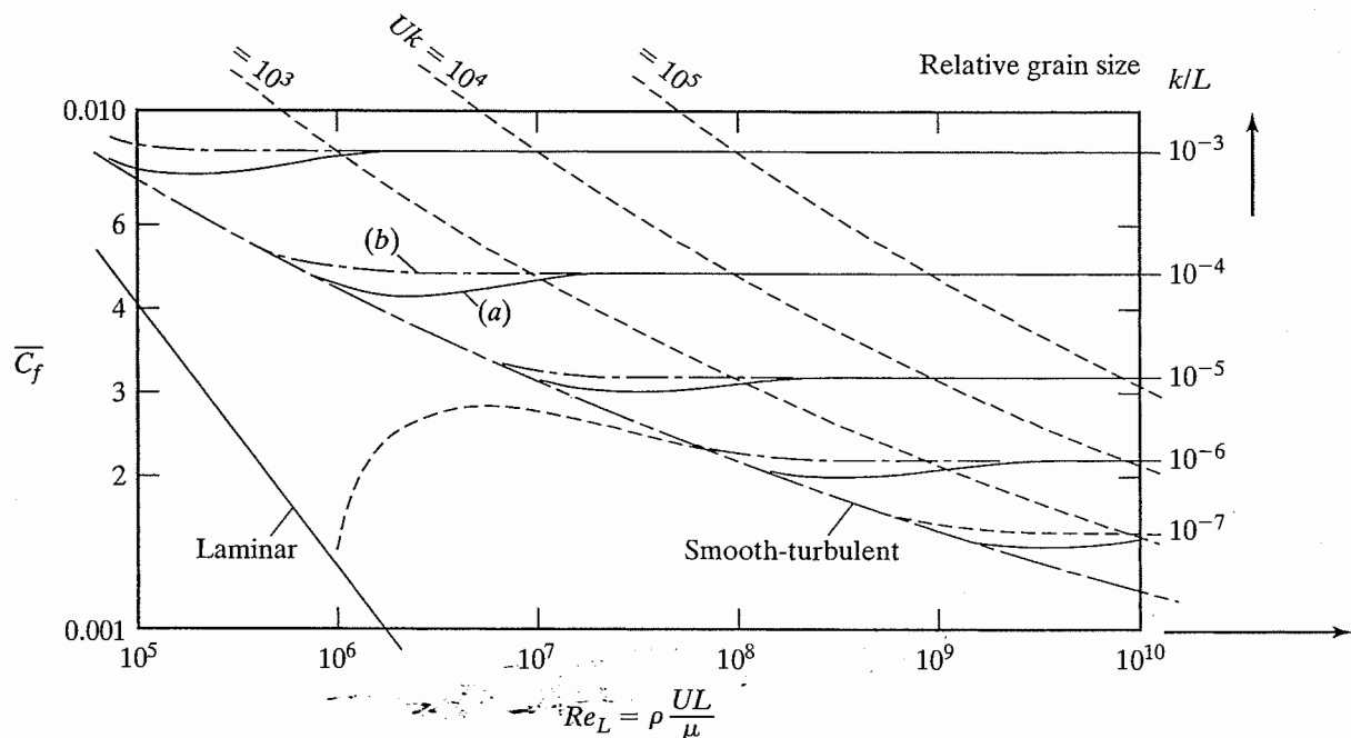
Figure 5.19 Effect of surface roughness on skin-friction drag. [From Hoerner (1965)].
