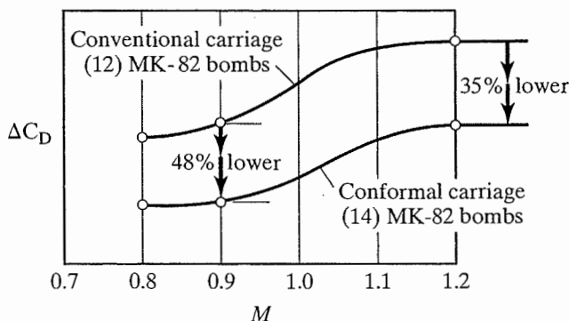
Figure 13.43 Drag comparison—conformal vs. conventional carriage. [From Bradley (1981).]
