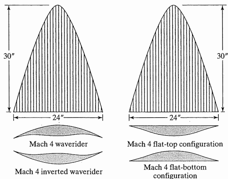
Figure 12.25 Waverider configurations tested in the Langley Unitary Plan Wind Tunnel (UPWT). [Taken from Bowcutt et al. (1987).]
