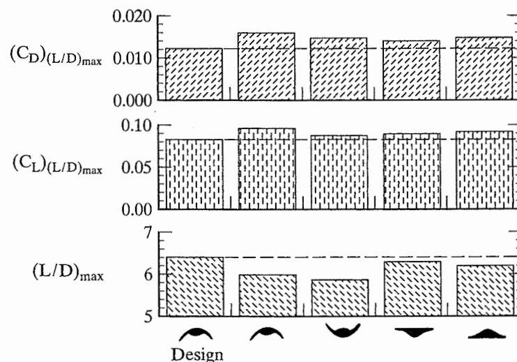
Figure 12.27 Aerodynamic characteristics at maximum L/D conditions, M_\infty = 4 , Re_{\infty/ft} = 2 \times 10^6 . [From Bauer et al. (1990).]
