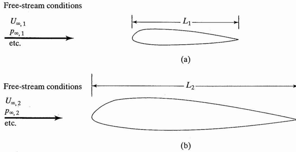
Figure 2.11 Flow around geometrically similar (but different size) configurations: (a) first flow; (b) second flow.
