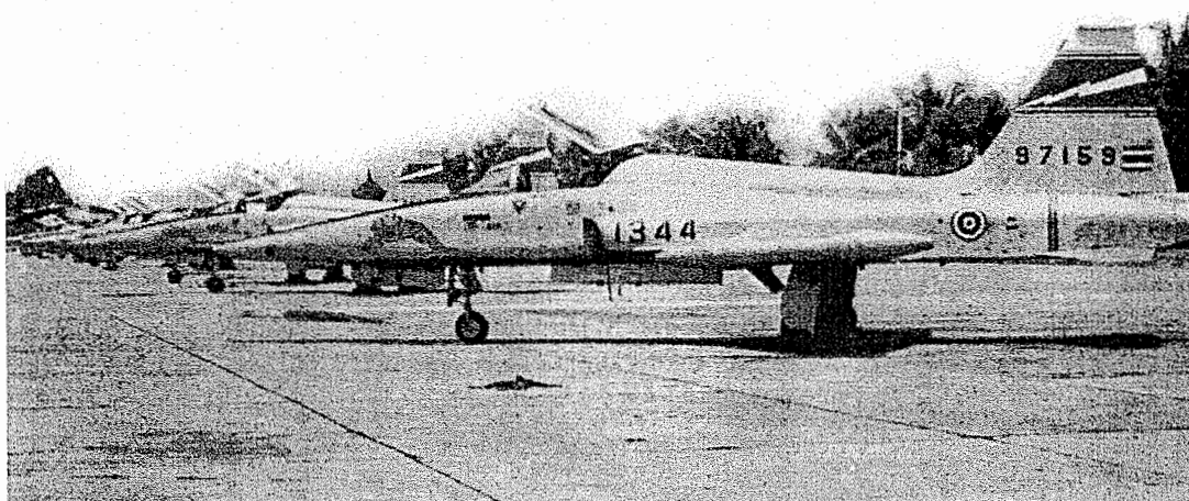
Figure 9.27 Illustration of the application of the area rule to the tip tanks of the F-5. (From the author's collection.)
