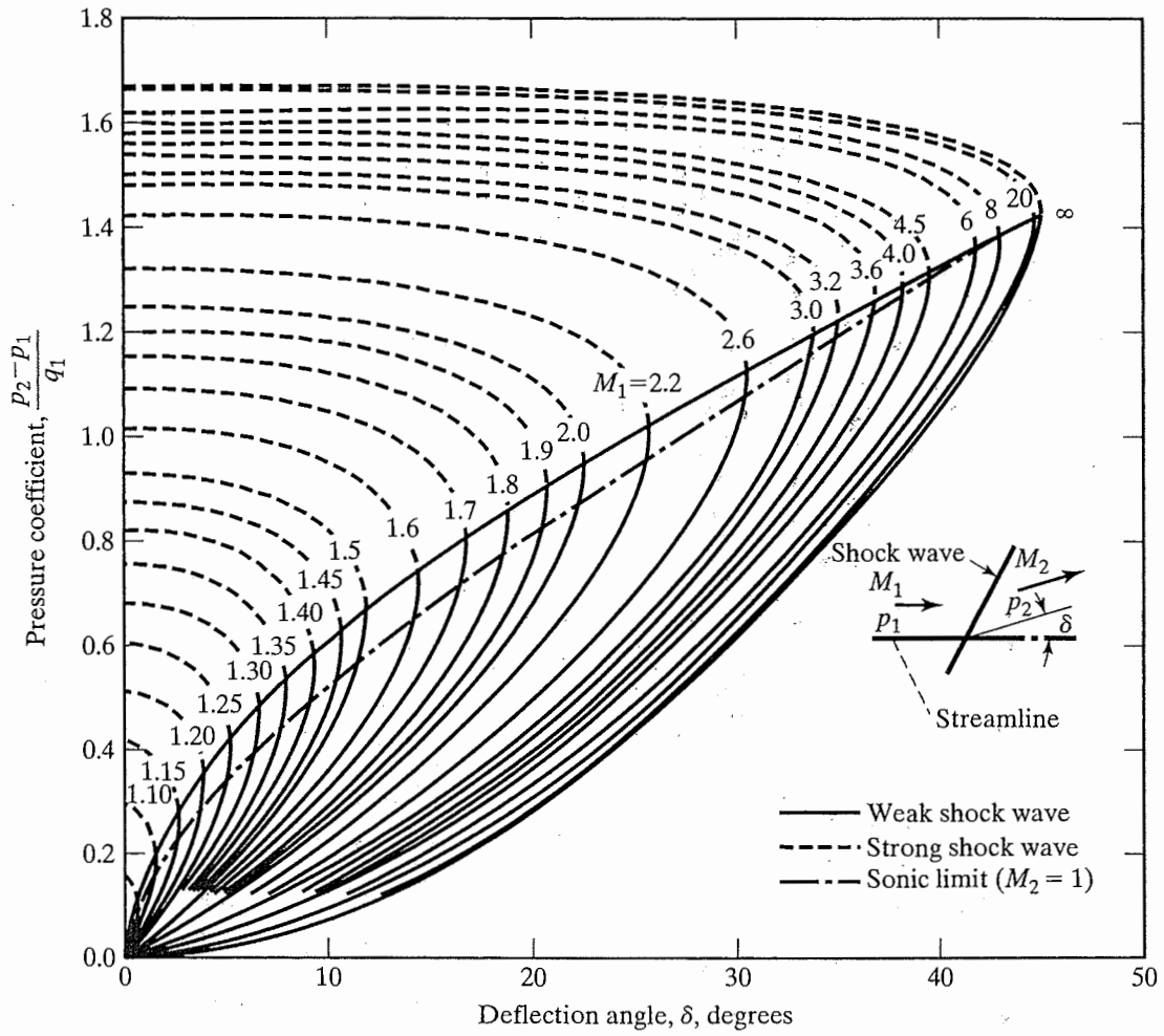
Figure 8.12 (continued) (b) pressure coefficient.
