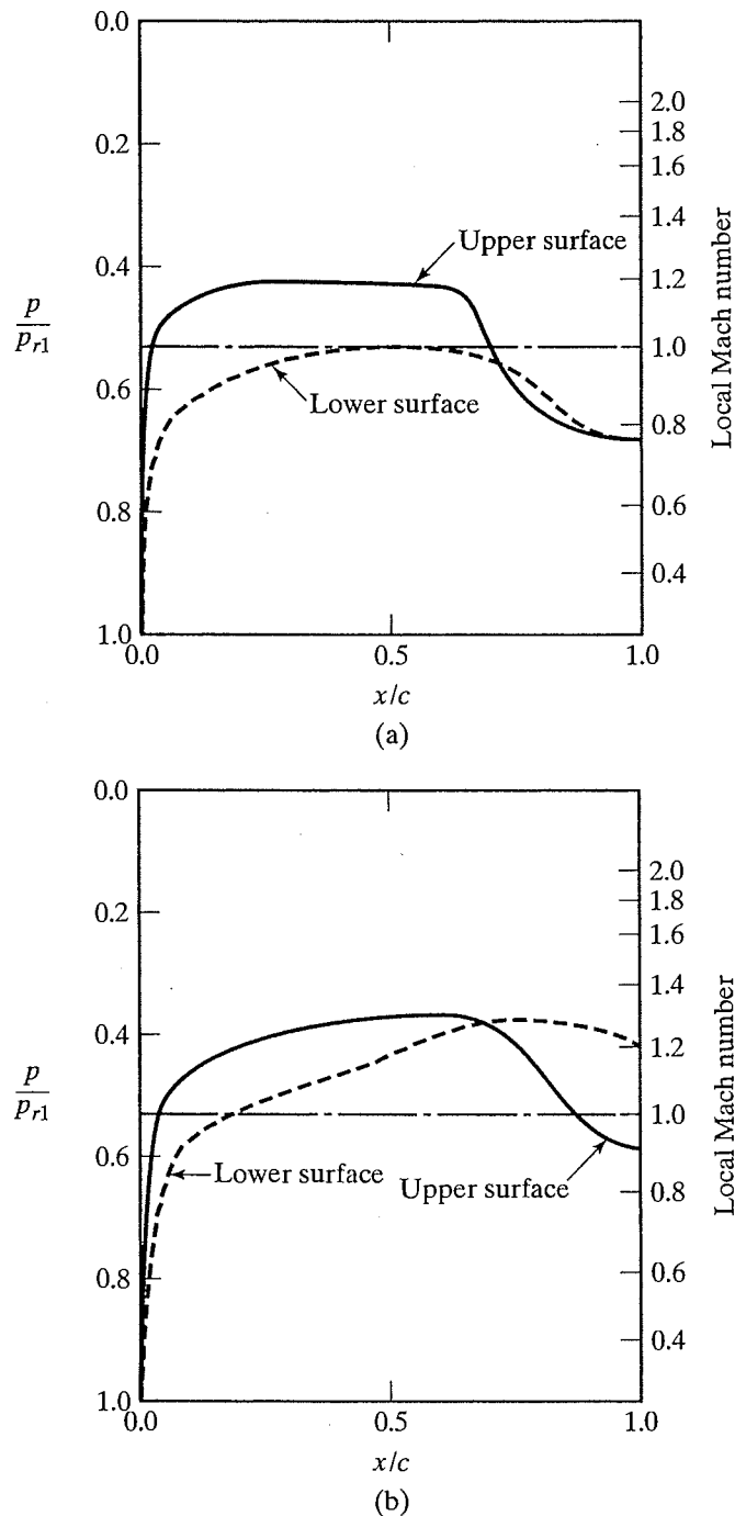
Figure 9.9 Pressure distribution and local Mach number distribution for transonic flows around an airfoil: (a) Flow at the trailing edge is subsonic, M_\infty = 0.81 ; (b) flow at the lower surface trailing edge is supersonic, M_\infty = 0.89 . [From Farren (1956).]
