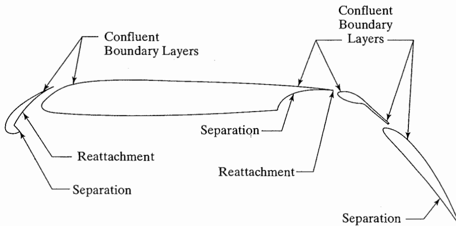
Figure 6.24 Sketch of the cross section of a typical high-lift multi-element airfoil section. [Taken from Jasper et al. (1993).]
