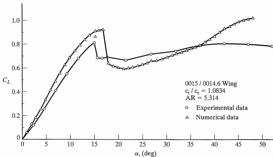
Figure 7.21 Lift coefficient versus angle of attack for a drooped leading-edge wing; comparison between experiment and numerical results. [Taken from Anderson, Corda, and Van Wie (1980).]
