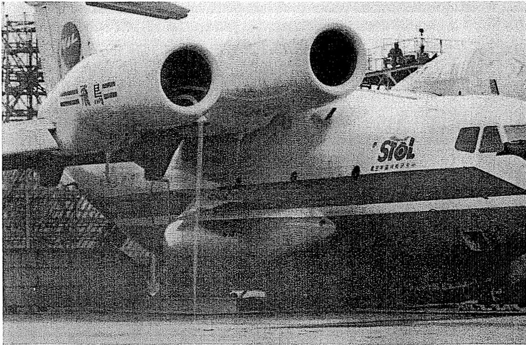
Figure 3.14 Ground vortices between engine intake and ground and between adjacent engines for Asuka STOL research aircraft during static tests. [Taken from Campbell and Chambers (1994).]
