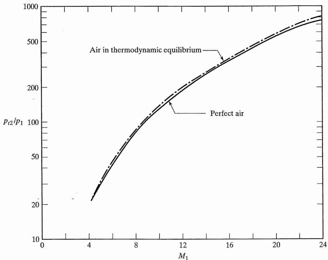
Figure 12.7 Pressure at the stagnation point of a sphere ( R_N = 0.3048 m) at an altitude of 45,721 m.
