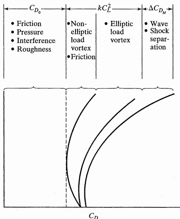
Figure 5.30 Lift/drag polar for a large, subsonic transport. [From Bowes (1974). The original version of this material was first published by the Advisory Group for Aerospace Research and Development, North Atlantic Treaty Organization (AGARD, NATO) in Lecture Series 67, May 1974.]
