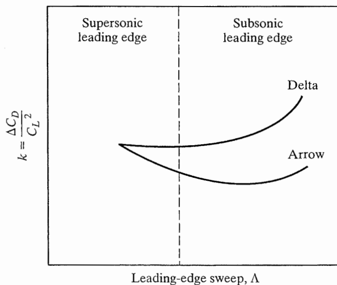
Figure 11.18 Comparison of induced drag for delta- and arrow-wing planforms. Note: \Delta C_D = \Delta C_{D0} . [From Wright et al. (1978).]
