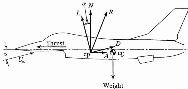
Figure 5.2 Nomenclature for aerodynamic forces in the pitch plane.
