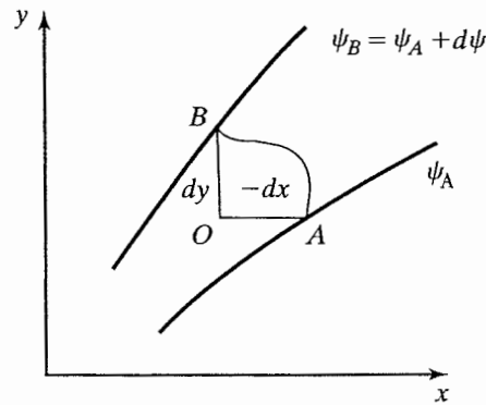
Figure 3.7 The significance of the stream function.
