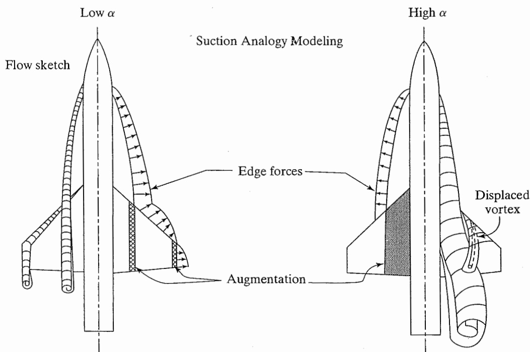
Figure 7.50 Theoretical vortex model for strake/wing configuration. [Taken from Lamar and Frink (1982).]
