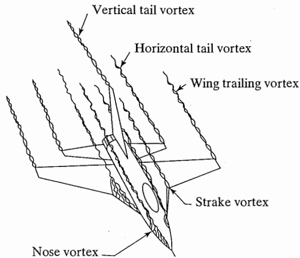
Figure 7.58 Vortex wakes near a maneuvering fighter. [Taken from Mendenhall and Perkins (1996).]
