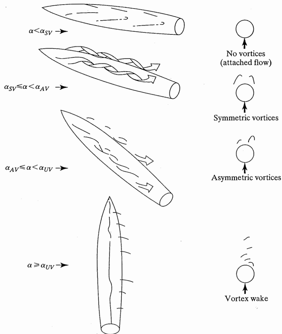
Figure 7.55 Effect of angle of attack on the leeside flowfield. [From Ericsson and Reding (1986).]
