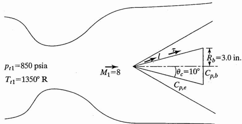
Figure 12.18 Sharp cone mounted in Tunnel B of AEDC.
