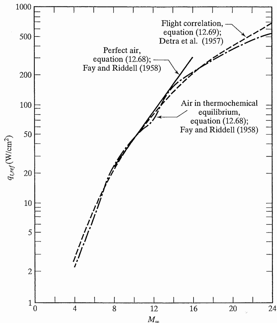
Figure 12.32 Heat-transfer rate at the stagnation point of a sphere ( R_N = 0.3048 m) at an attitude of 45,721 m.
