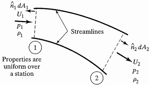
Figure 8.3 One-dimensional flow in a streamtube.
