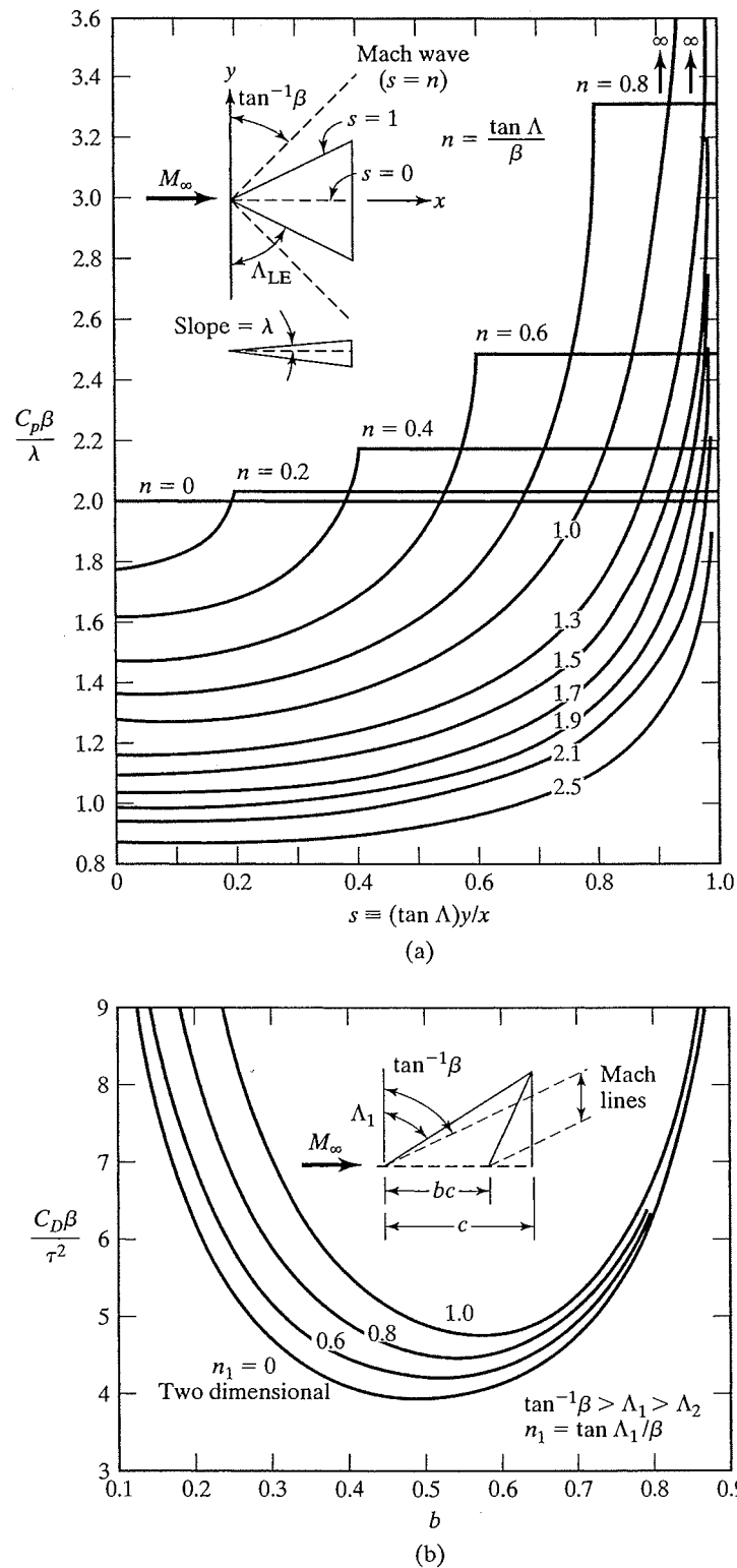
Figure 11.21 Theoretical solutions for a delta wing. (a) pressure distribution for a single-wedge delta wing at \alpha = 0 . (b) Thickness drag of a double-wedge delta wing with a supersonic leading edge and a supersonic line of maximum thickness. [From Puckett (1946).]
