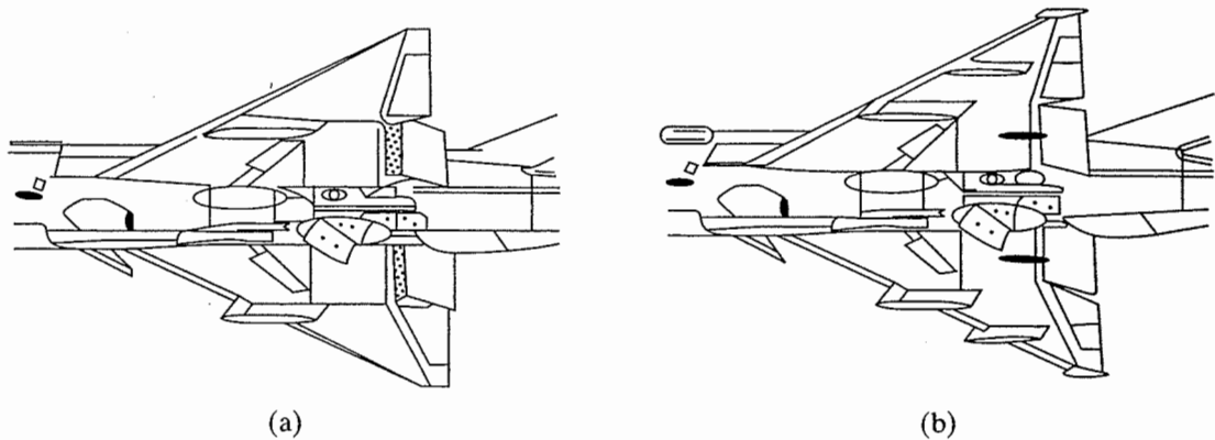
Figure 13.12 Fowler-type flaps used on early series MiG 21s and the blown flaps used on later series: (a) Fowler-type flaps employed on the MiG-21 PF; (b) blown flaps employed on the MiG-21 MF. [From Air Enthusiast International (1974).]
