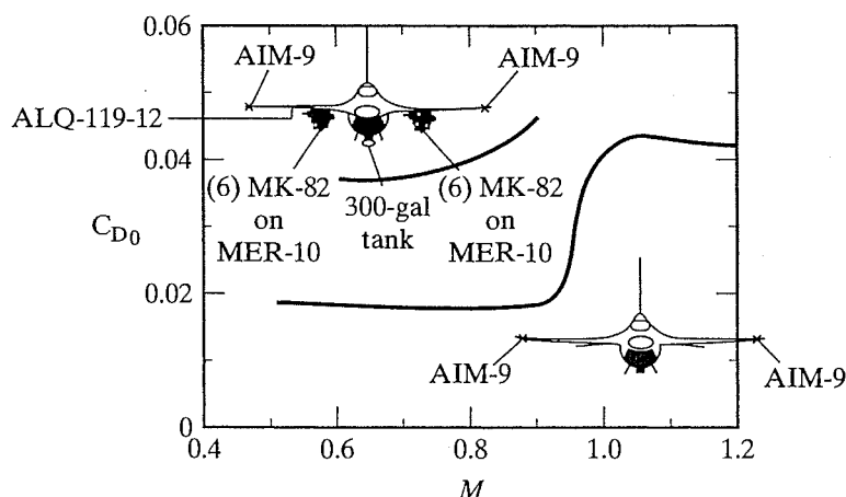
Figure 13.42 Stores drag effect [From Bradley (1981).]
