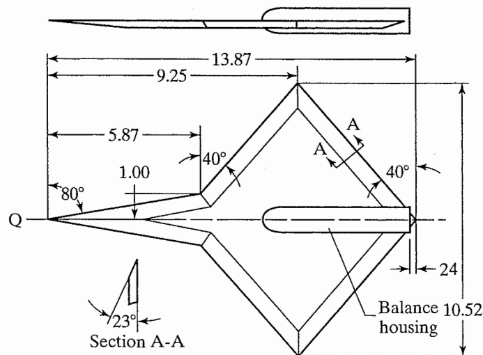
Figure 7.62 Unusual UAV configuration. [From Hammons and Thompson (2006).]
