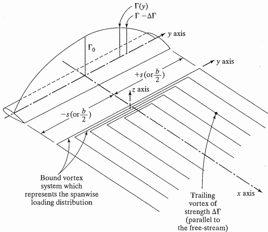
Figure 7.4 (a) Schematic trailing-vortex system.
