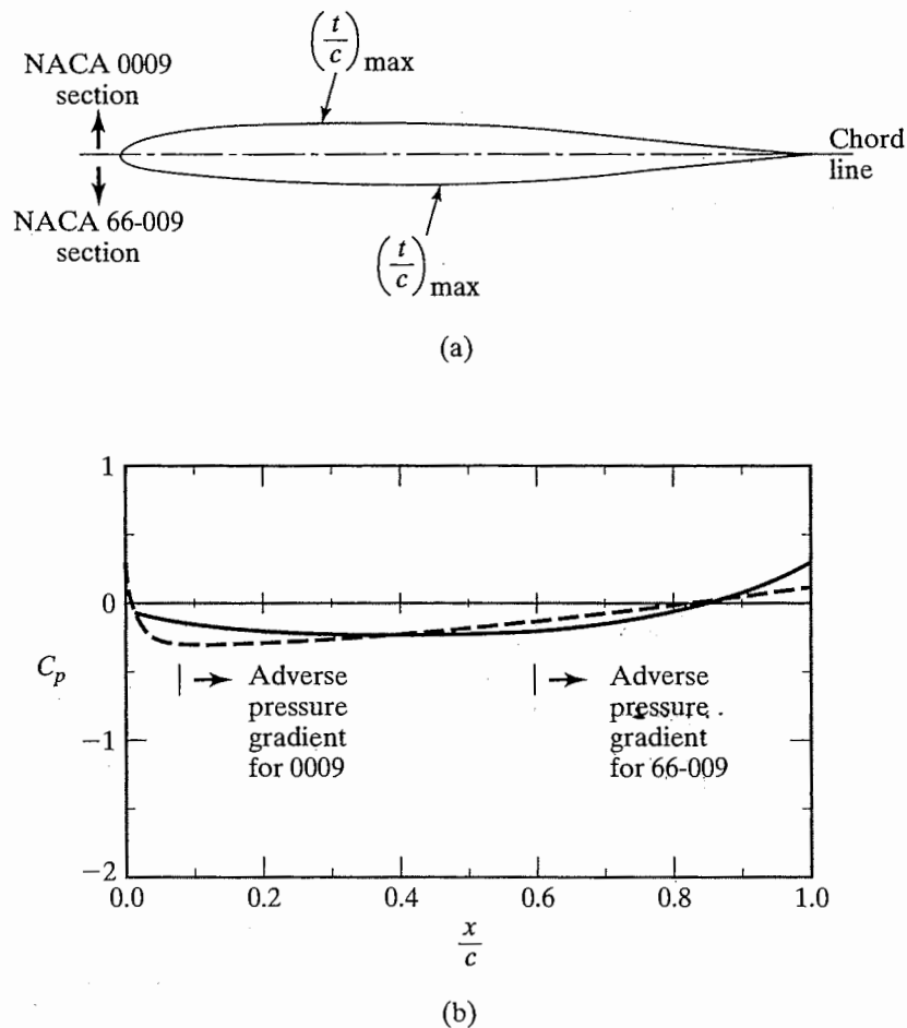
Figure 5.15 Comparison of geometries and resultant pressure distributions for a “standard” airfoil section (NACA 0009) and for a laminar airfoil section (NACA 66-009): (a) comparison of cross section for an NACA 0009 airfoil with that for an NACA 66-009 airfoil; (b) static pressure distribution.
