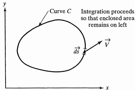
Figure 3.4 Concept of circulation.
