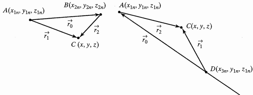
Figure 7.29 Vector elements for the calculation of the induced velocities.
