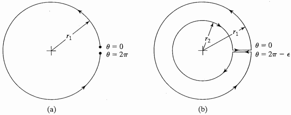
Figure 3.13 Paths for the calculation of the circulation for a potential vortex: (a) closed curve C_1 , which encloses origin; (b) closed curve C_2 , which does not enclose the origin.
