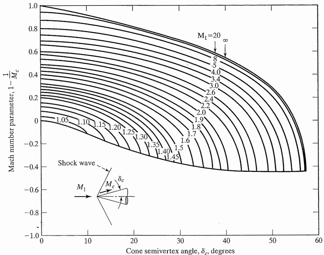
Figure 8.15 (continued) (c) Mach number on the surface of the cone.
