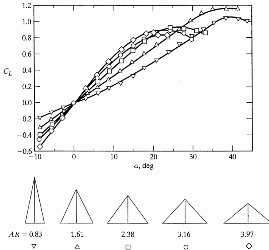
Figure 7.46 Lift coefficients for delta wings of various aspect ratios; t = 0.12c , Re_c \approx 7 \times 10^5 . [Data from Schlichting and Truckenbrodt (1969).]
