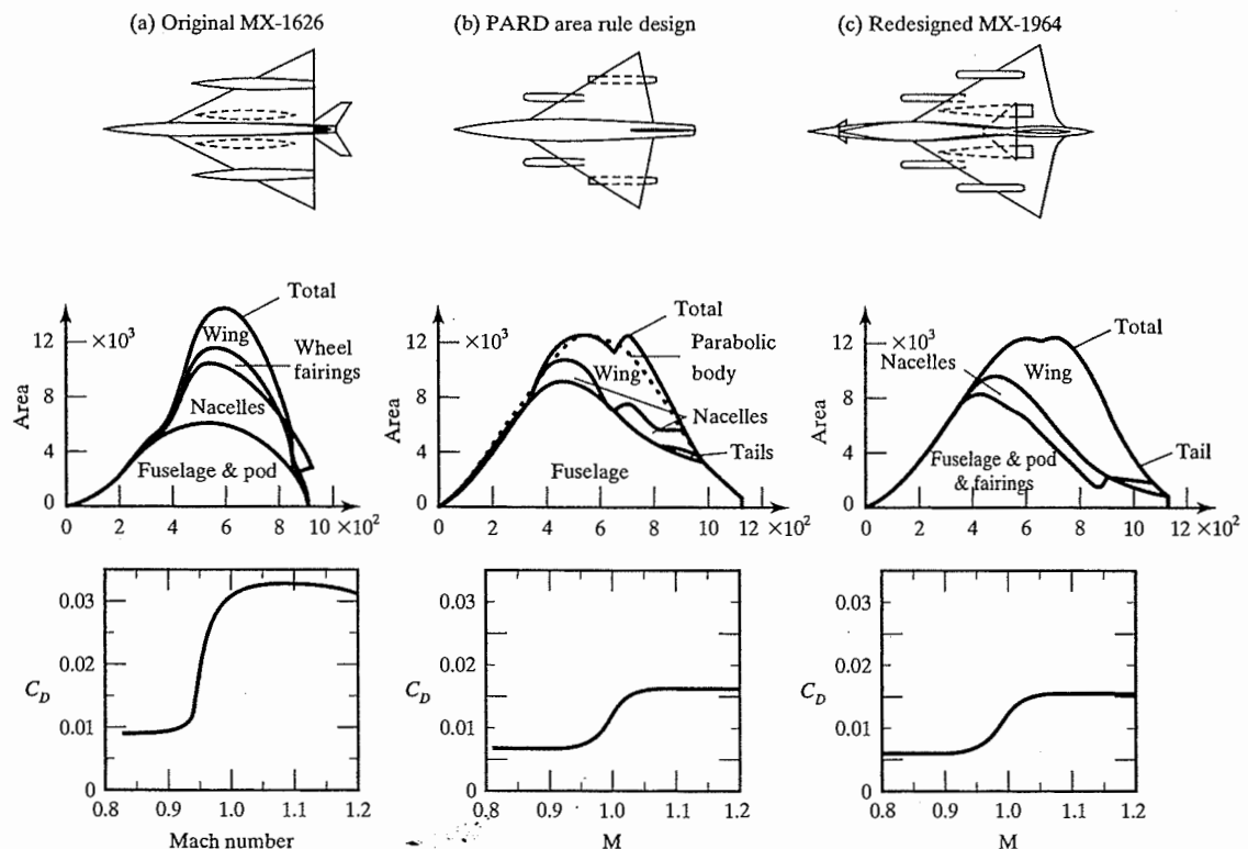
Figure 9.23 Planform sketches, longitudinal distributions of cross-sectional areas, and drag coefficients for equivalent bodies of revolution for supersonic bomber models. [Taken from Shortal (1978).]
