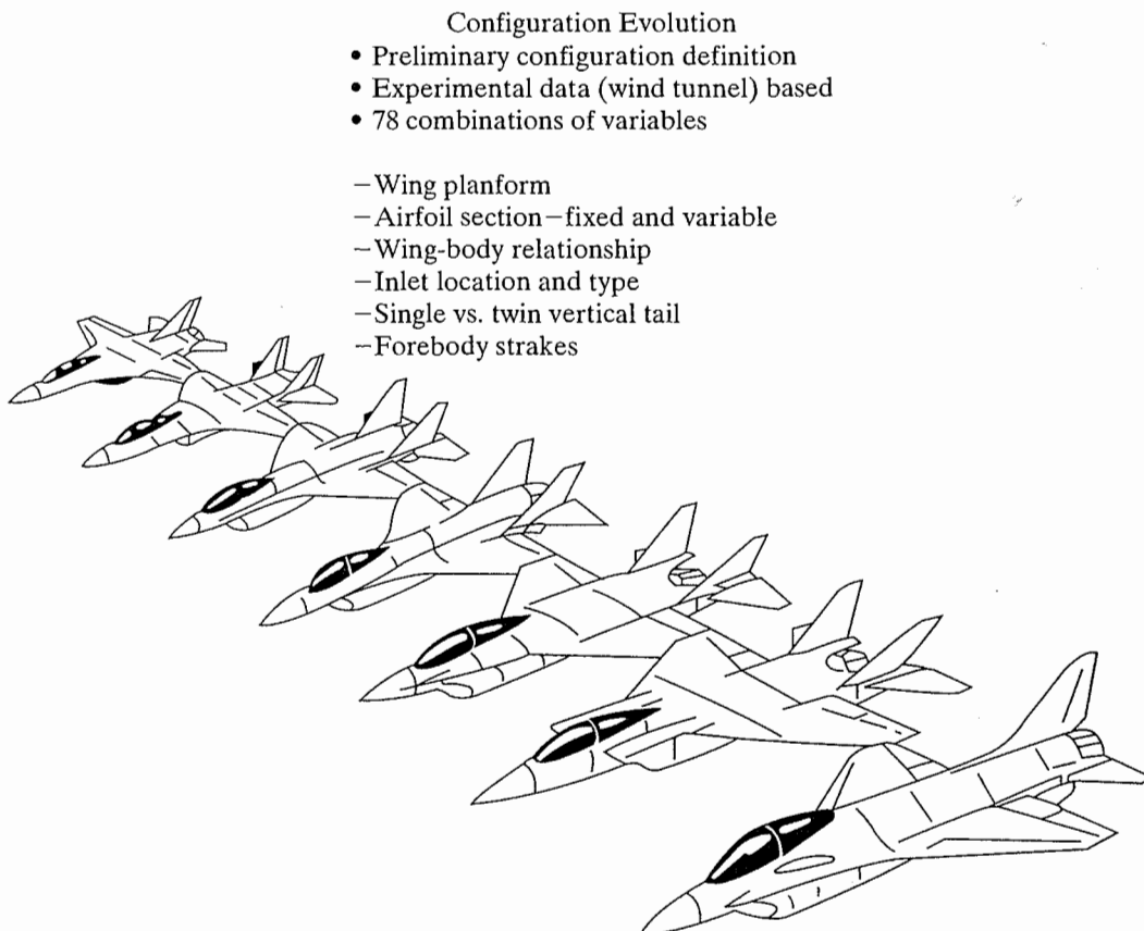
Figure 13.37 Configuration evolution for the F-16.
