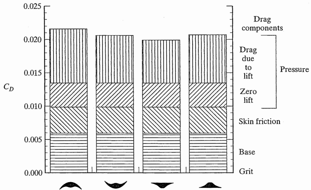
Figure 12.26 Breakdown of drag components at maximum L/D conditions, M_\infty = 4 , Re_{\infty/ft} = 2 \times 10^6 . [From Bauer et al. (1990).]
