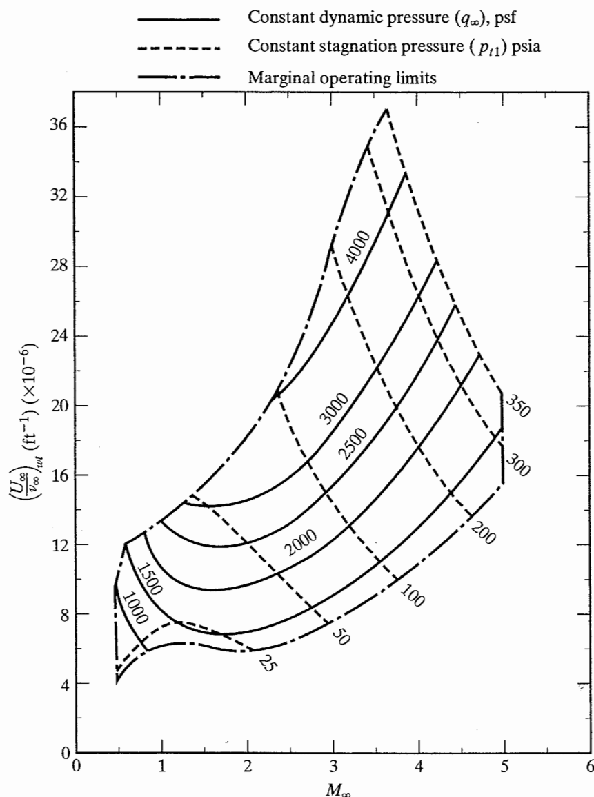
Figure 8.20 Free-stream unit Reynolds number as a function of the free-stream Mach number for T_t = 100^\circ\text{F} in the Vought High-Speed Wind Tunnel. [From Arnold (1968).]
