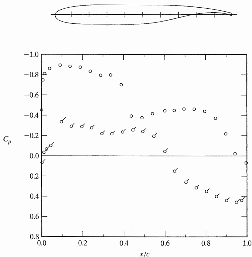
Figure 9.17 Experimentally determined pressure distribution for a supercritical airfoil section, M_\infty = 0.80 , C_l = 0.54 , Re_c = 3.0 \times 10^6 (flagged symbols are for the lower surface). [Data from Hurley et al. (1975).]
