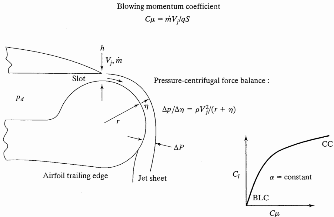
Figure 13.16 Basic principles of circulation control aerodynamics. [From Englar (1987).]
