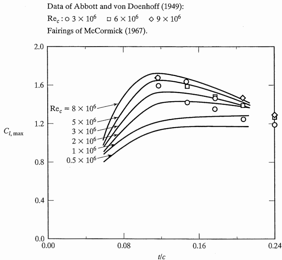
Figure 6.10 Effect of the thickness ratio on the maximum lift coefficient, NACA 24XX series airfoil sections.
