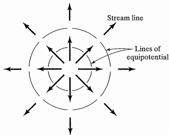
Figure 3.10 Equipotential lines and streamlines for flow from a two-dimensional source.
