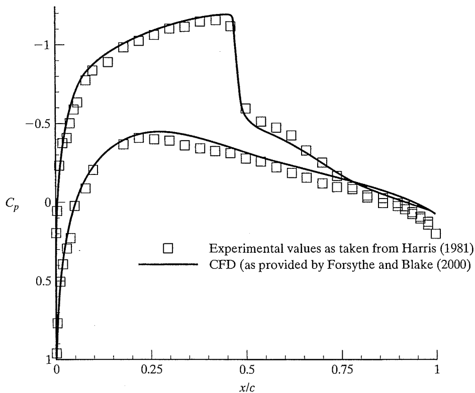
Figure 9.11 Pressure distributions for a NACA 0012 in a Mach 0.8 stream at \alpha = 3^\circ .
