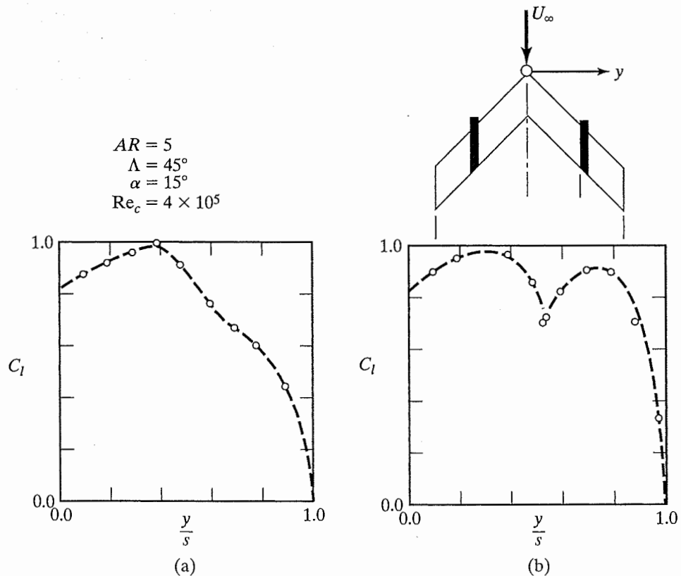
Figure 7.34 Effect of a boundary-layer fence on the spanwise distribution of the local lift coefficient: (a) without fence; (b) with fence. [Data from Schlichting (1960).]
