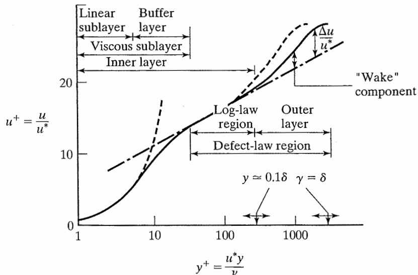
Figure 4.15 Turbulent boundary layer illustrating wall-layer nomenclature.
