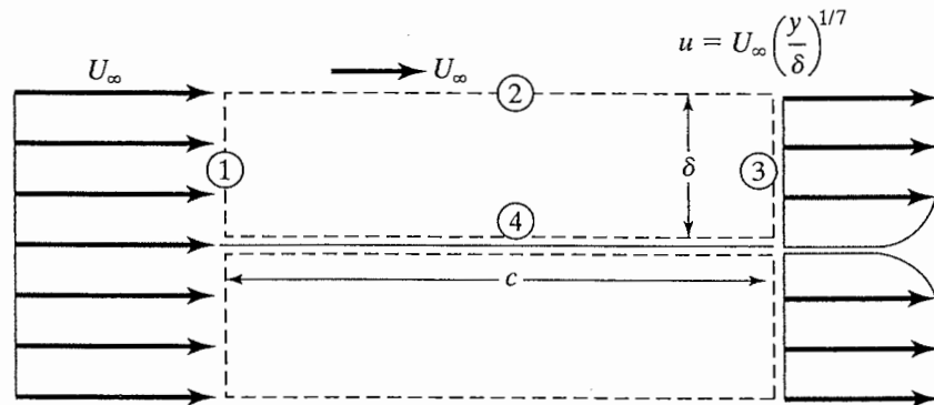
Figure 2.10 Flow diagram for Example 2.3.
