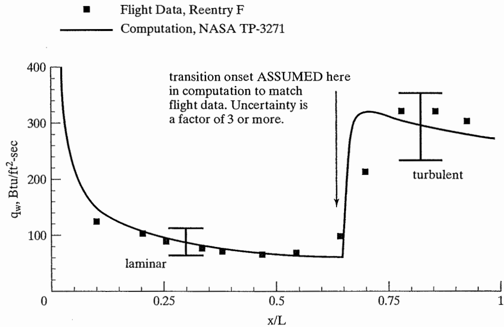
Figure 12.38 Heating-rate distribution along cone for reentry F.
