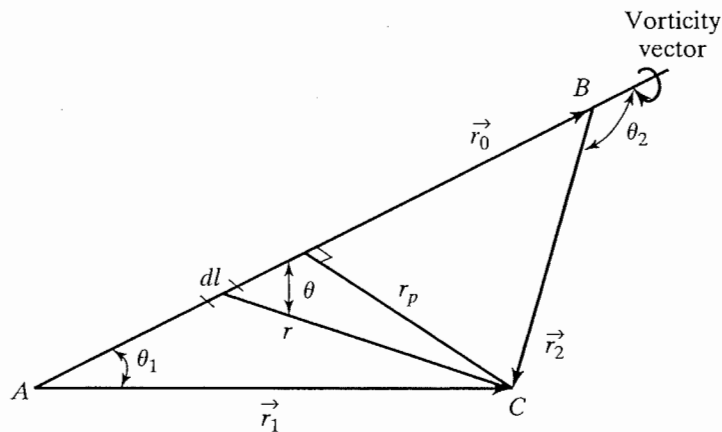
Figure 7.27 Nomenclature for calculating the velocity induced by a finite-length vortex segment.
