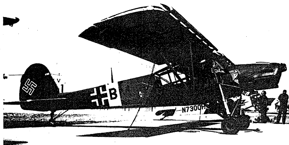
Figure 13.15 Fieseler Storch, Fi 156, showing fixed leading-edge slots and hinged trailing edge. (Courtesy of Jay Miller, "Aerophile.")
