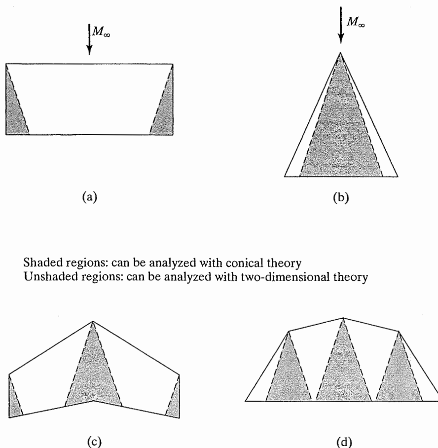
Figure 11.8 Examples of regions that can be treated with conical theory: (a) rectangular wing; (b) delta wing; (c) swept wing; (d) “double” delta wing.
