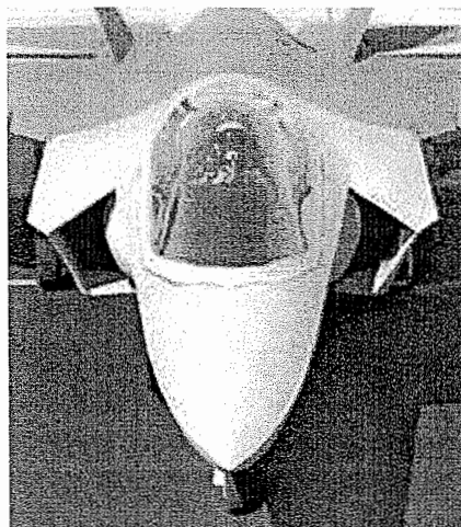
Figure 13.52 The JSF diverterless supersonic inlet. (Photo courtesy of Lockheed Martin.)
