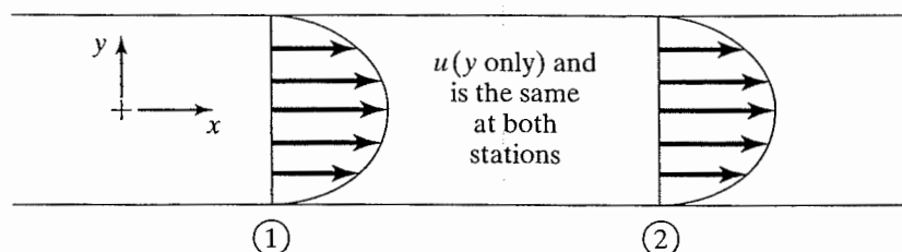
Figure 2.9 Another flow diagram for Example 2.2.
