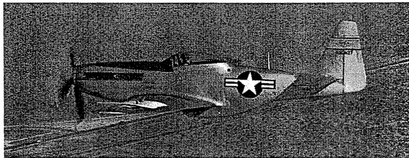
Figure 6.14 Restored NACA P-51 with laminar flow airfoil sections. [Courtesy of NASA Dryden Flight Research Center.]
