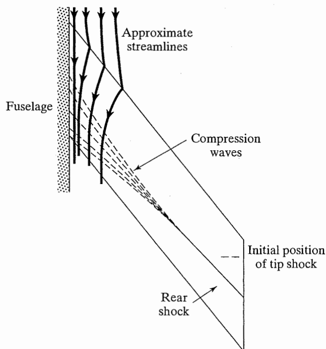
Figure 9.21 Formation of rear shock from compression waves associated with flow near the root. [From Rogers and Hall (1960).]
