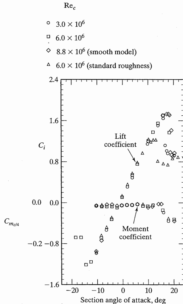
Figure 5.12 Section lift coefficient and section moment coefficient (with respect to c/4 ) for an NACA 23012 airfoil. [Data from Abbott and von Doenhoff (1949).]
