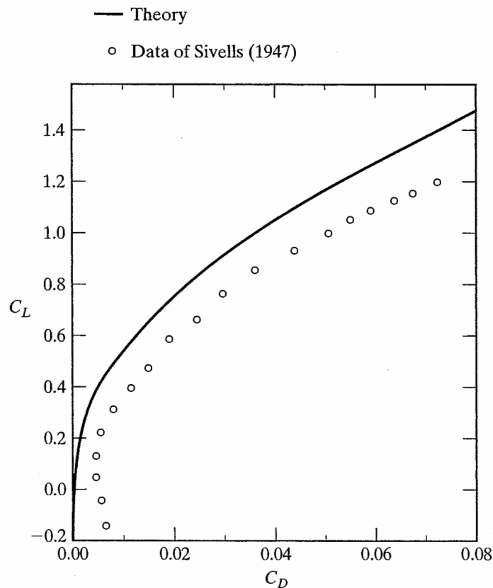
Figure 7.16 Comparison of the theoretical induced drag coefficients and the measured drag coefficients for an unswept wing in a subsonic stream. (Wing is that of Fig. 7.13.)
