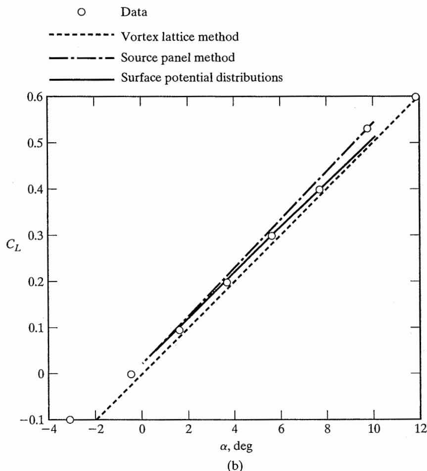
Figure 7.23 (continued) (b) \Lambda_{c/4} = -45^\circ , NACA 64A112 section, AR = 3.55 , \lambda = 0.5 , forward swept wing. [From Margason et al. (1985).]
