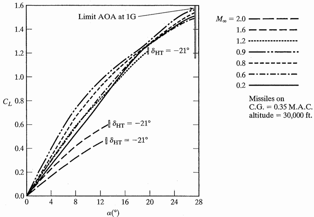
Figure 5.26 Trimmed lift coefficient as a function of the angle of attack for the F-16C. \delta_{HT} is deflection of the horizontal tail. [Provided by the General Dynamics Staff (1976).]
