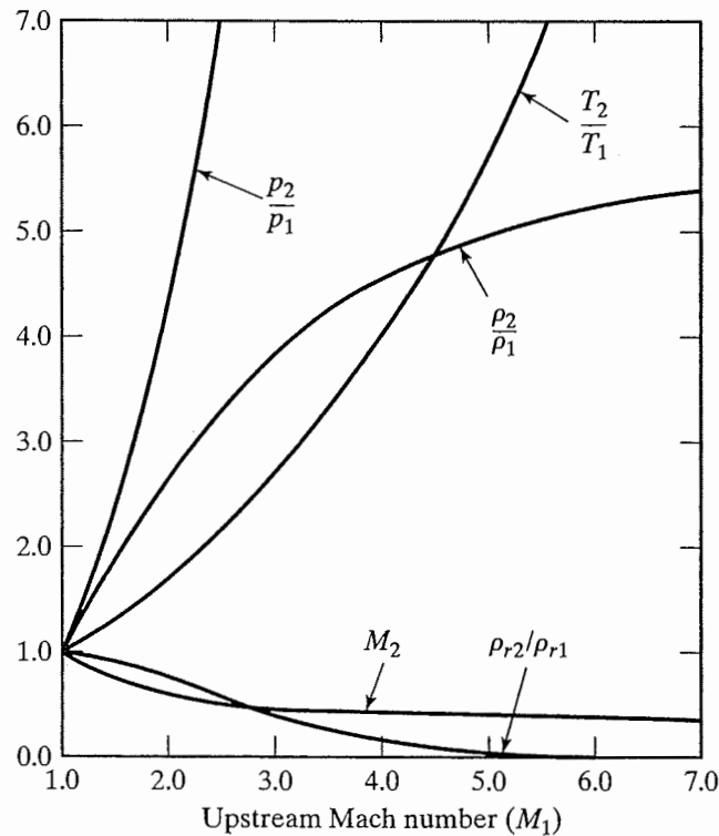
Figure 8.13 Property variations across a normal shock wave.
