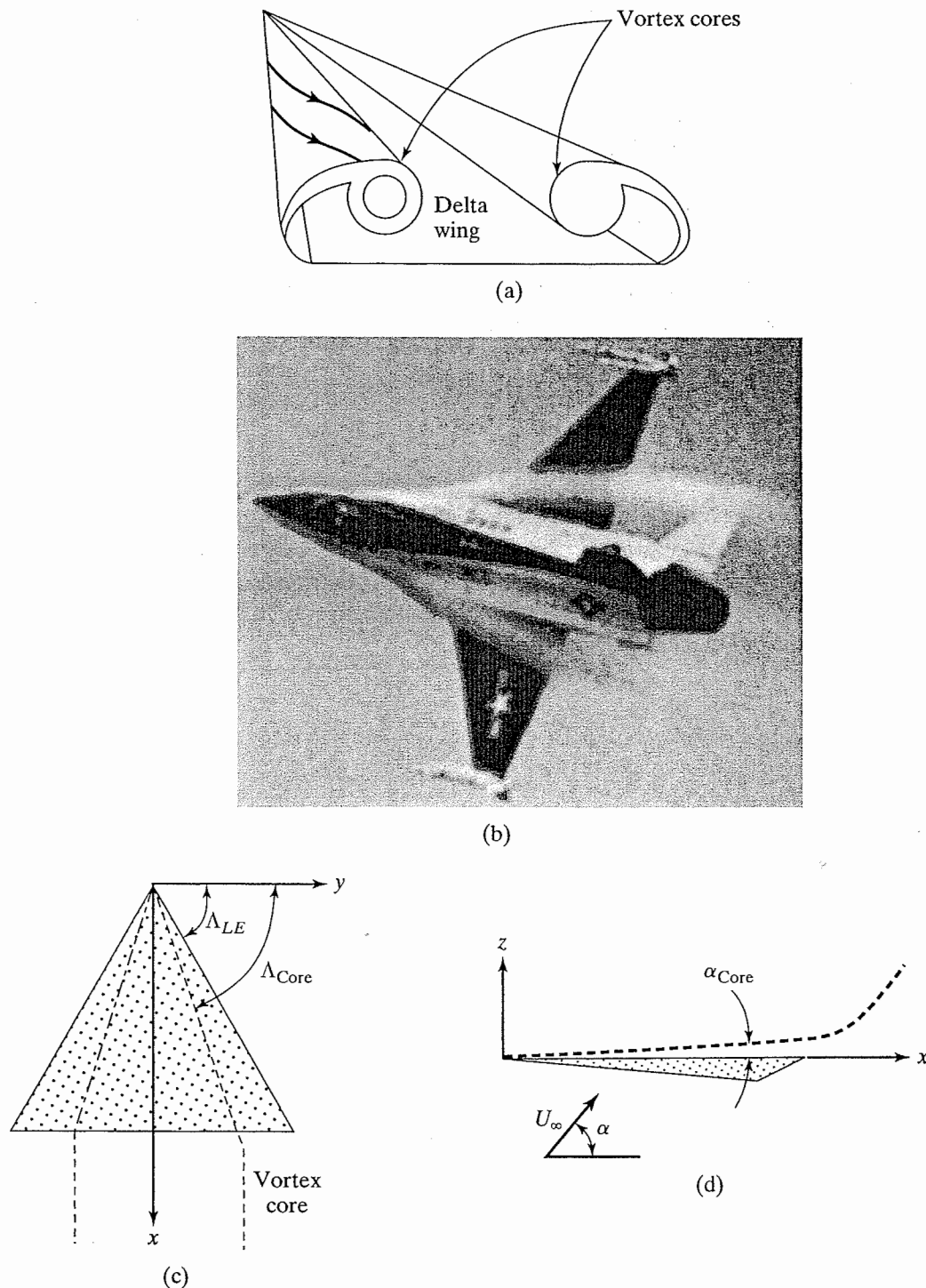
Figure 7.40 (a) Vortex core that develops for flow over a delta wing. (b) Water vapor condenses due to the pressure drop revealing the vortex core for a General Dynamic F-16. (Photograph courtesy of General Dynamics.) (c) Trajectory of the leading-edge vortex. [Taken from Visbal (1995).] (d) Inclination angle of the vortex trajectory. [Taken from Visbal (1995).]
