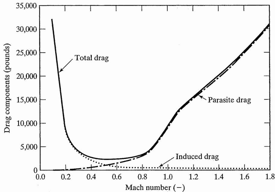
Figure 5.31 Drag components for an F-16C flying in steady, level, unaccelerated flight at 20,000 ft.
