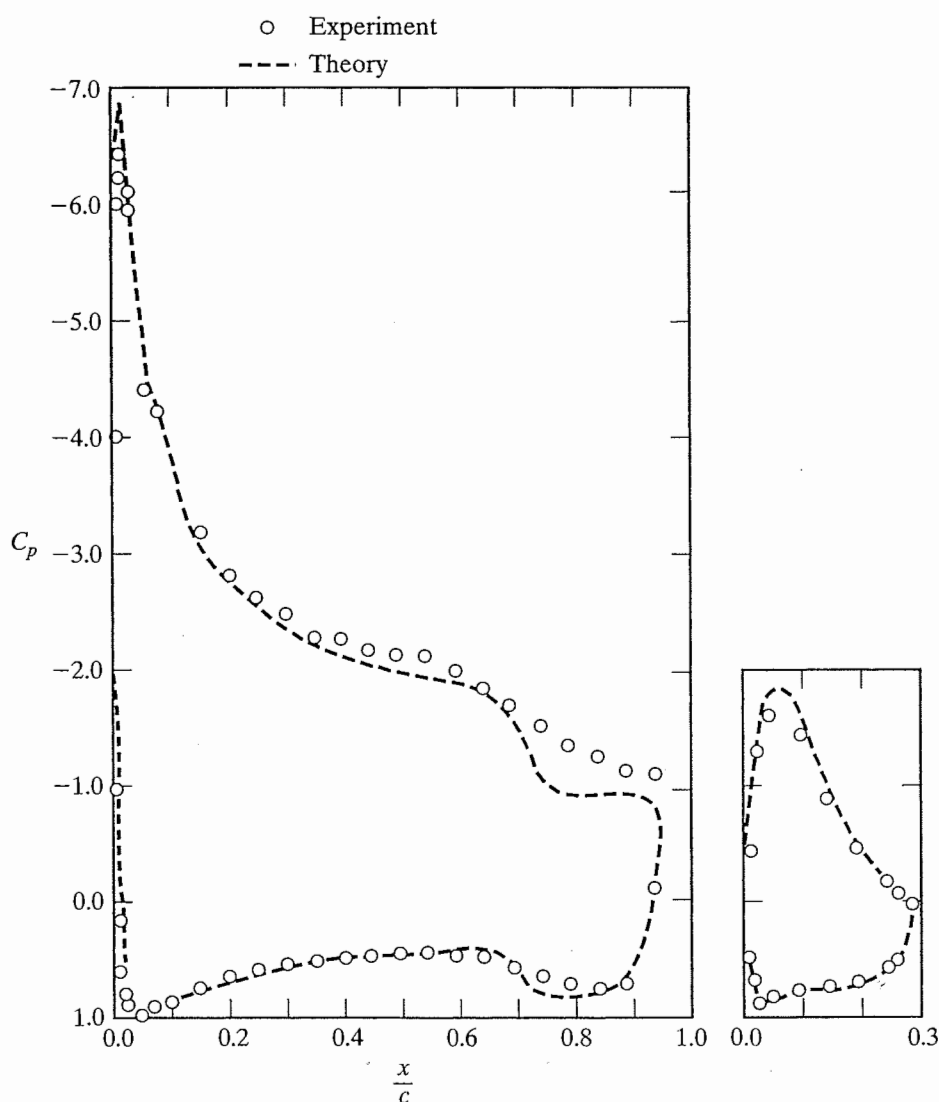
Figure 13.11 Comparison of the theoretical and the experimental pressure distribution for a GA(W)-1 airfoil with a slotted flap, \alpha = 5^\circ , \delta_f = 30^\circ . [From Wentz and Seetharam (1974).]
