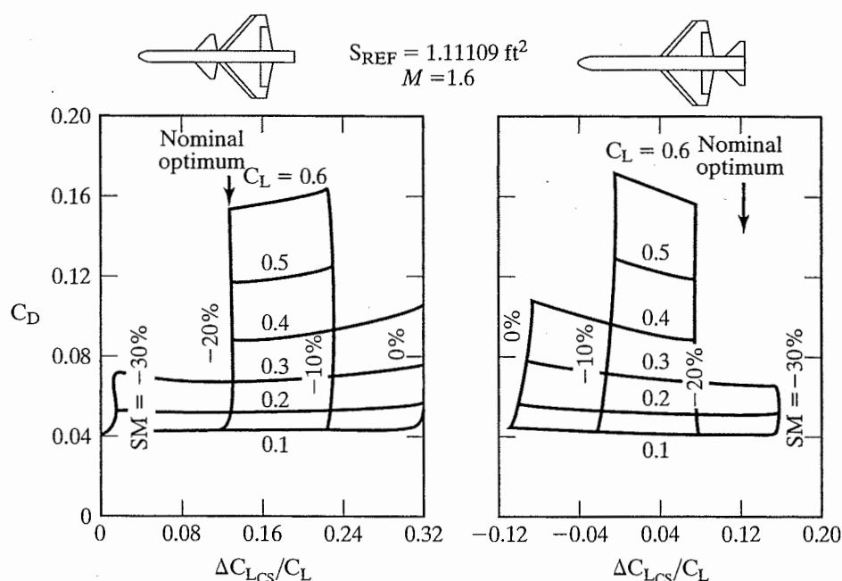
Figure 13.49 Effect of control surface lift on trimmed supersonic drag for canard and tail arrangements with the 44-degree sweep trapezoidal wing. [From Nicholas et al. (1984).]
