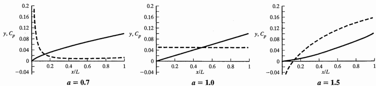
Figure 11.41 Pressure coefficients for various power series body shapes (body shape in solid line, pressure coefficient in dashed line).
