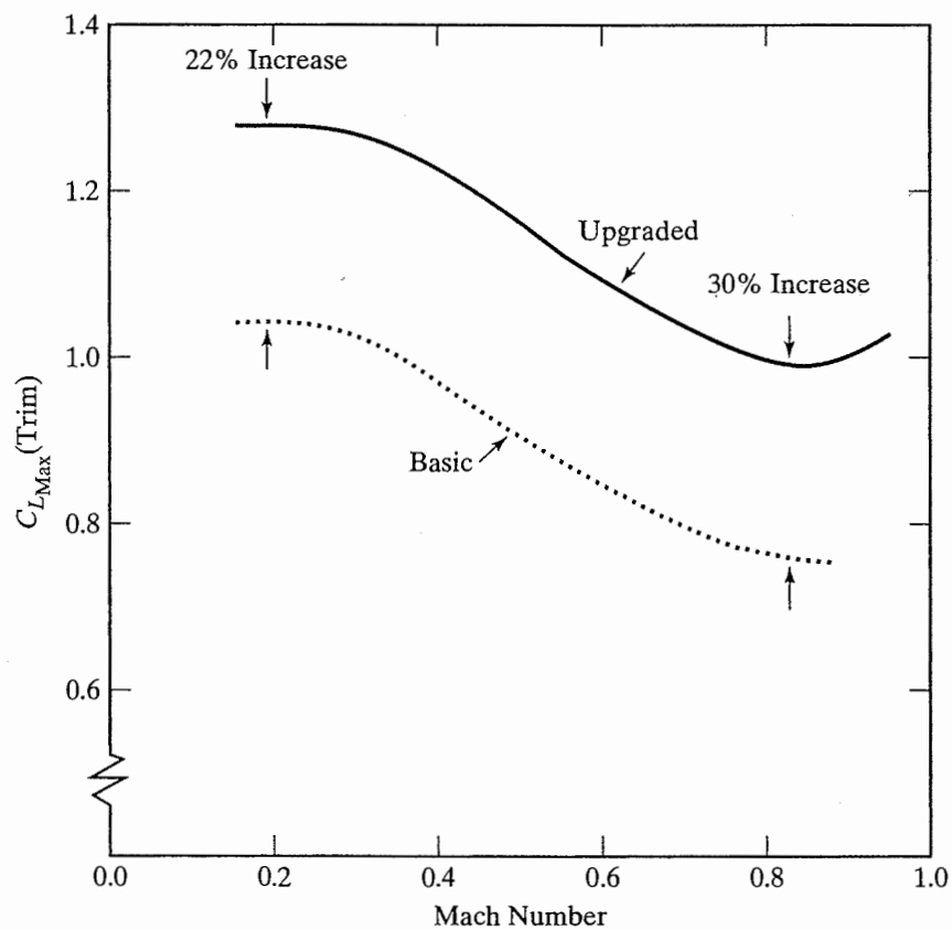
Figure 13.35 Increase in maximum usable lift. [From Gato and Masiello (1987).]
