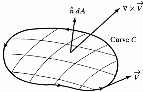
Figure 3.6 Nomenclature for Stokes's theorem.
