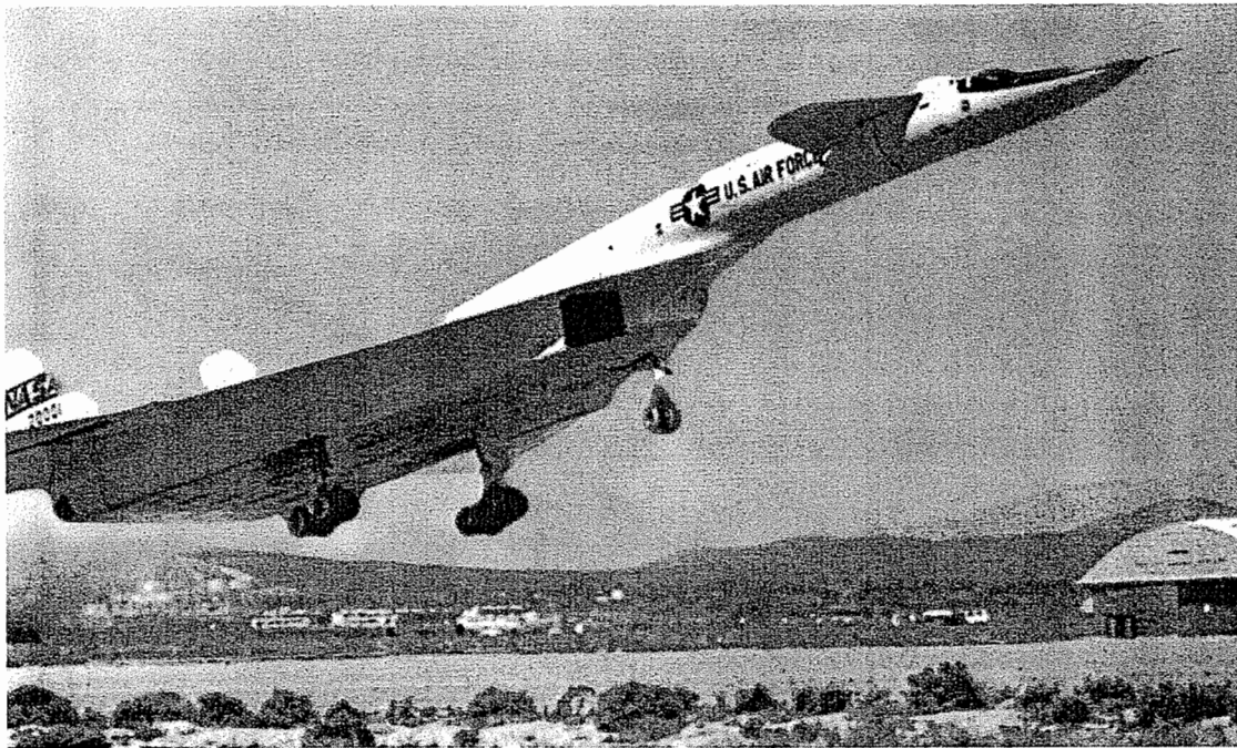
Figure 7.49 North American XB-70 illustrating the use of canards. (Courtesy of NASA.)
