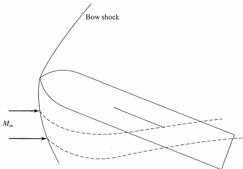
Figure 11.44 Body-on-wing interaction showing upwash-over-wing effect due to the body at angle of attack. [From Hilton (1951).]
