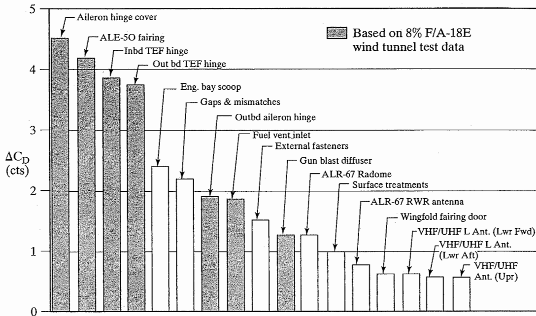
Figure 14.2 Protuberance drag for the F/A-18E. [Taken from Niewald and Parker (2000).]
