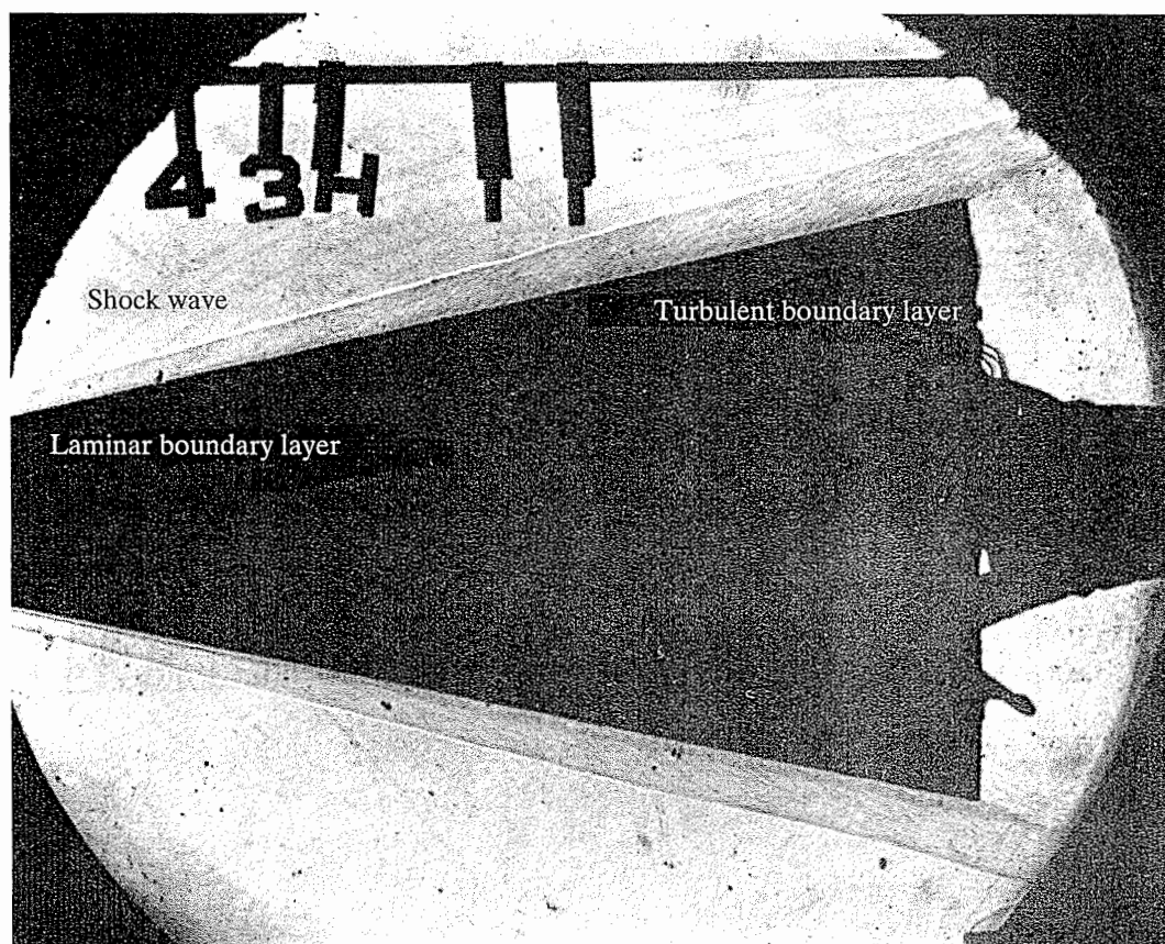
Figure 8.16 Hypersonic flow past a slender cone: M_\infty = 11.5 ; Re_{\infty,L} = 4.28 \times 10^6 ; \delta_c = 12^\circ . (Courtesy of Vought Corp.)
