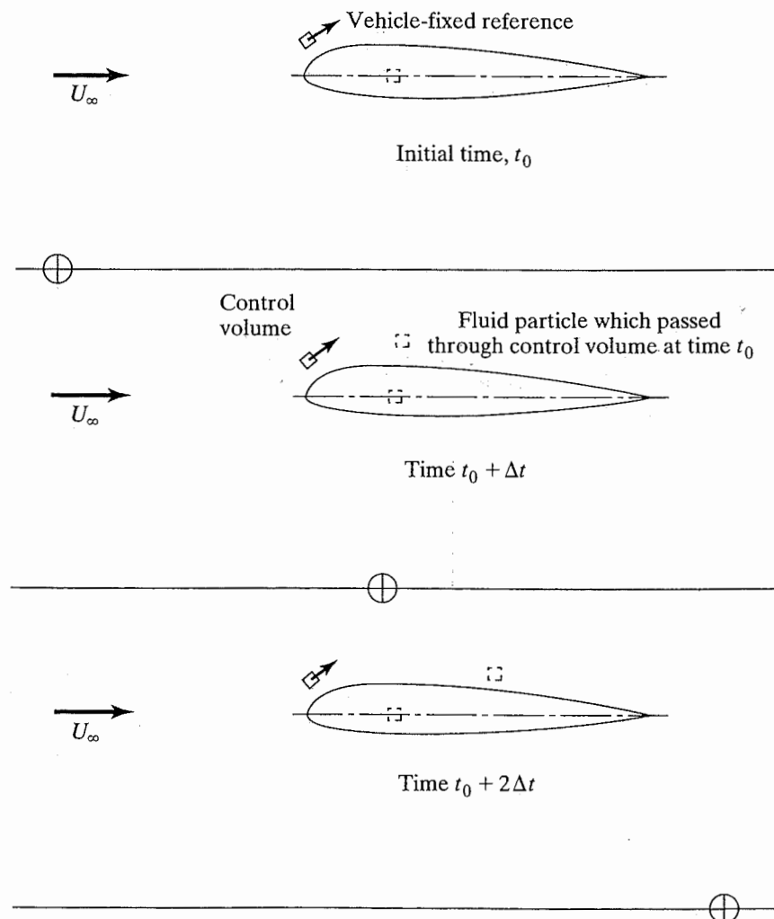
Figure 2.2 (Steady) airflow around a wing in a vehicle-fixed coordinate system.
