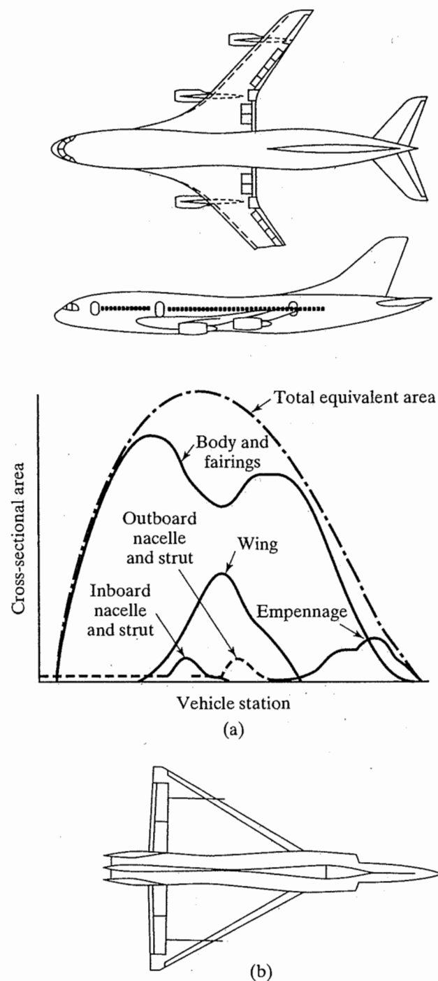
Figure 9.22 Application of the area rule to the axial distribution of the cross-sectional area: (a) area rule applied to the design of a near-sonic transport; (b) sketch of the Convair F 102 A. [From Goodmanson and Gratzner (1973).]
