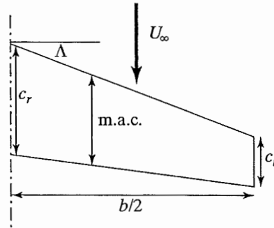
Figure 5.18 Geometry of a wing with a trapezoidal planform.
