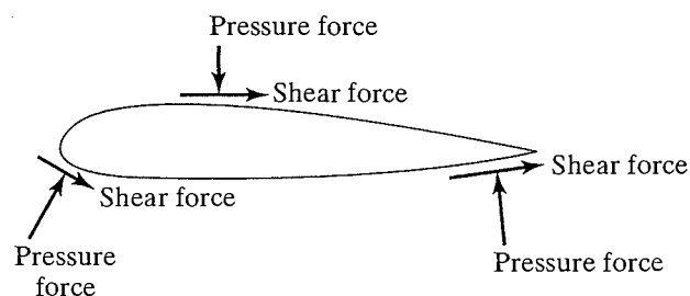
Figure 5.1 Normal (or pressure) and tangential (or shear) forces on an airfoil surface.
