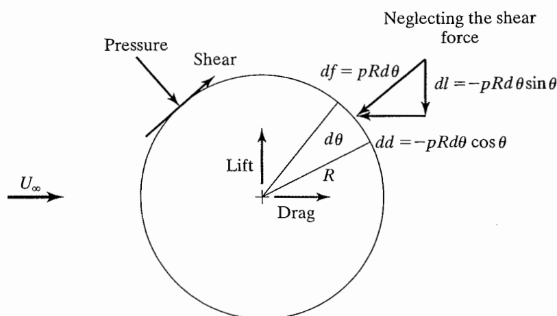
Figure 3.20 Forces acting on a cylinder whose axis is perpendicular to the free-stream flow.
