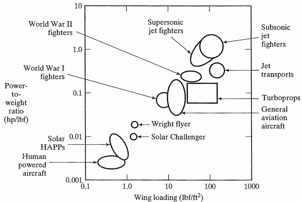
Figure 5.8 Historical ranges of power loading and wing loading. [From Hall (1985).]
