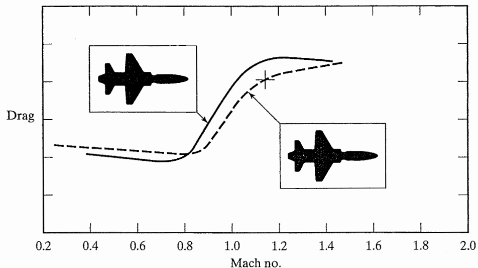
Figure 9.25 Reduction in the transonic drag rise due to the application of area rule to the F-5 fuselage. [From Stuart (1978).]
