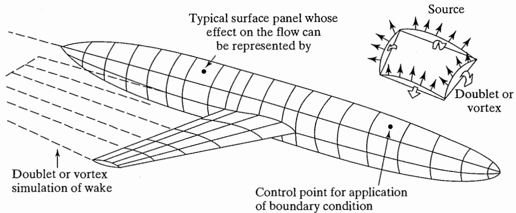
Figure 7.22 Representation of an airplane flowfield by panel (or singularity) methods.
