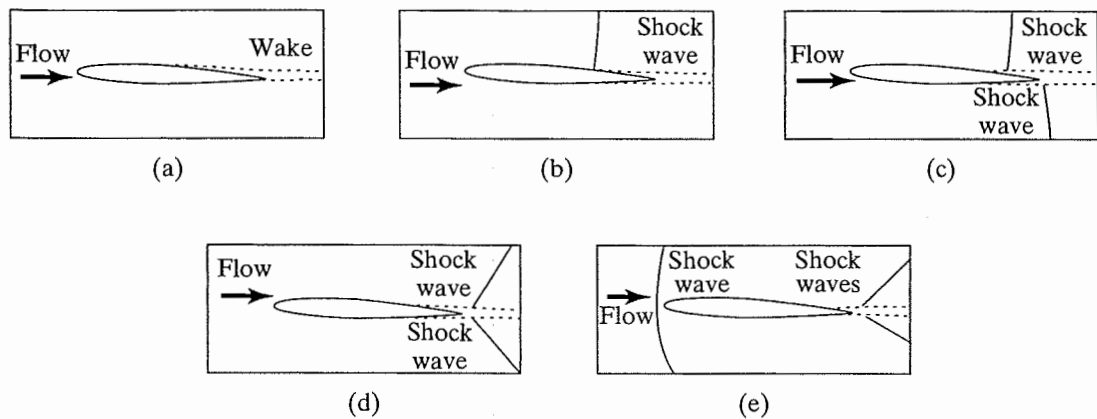
Figure 9.8 Flow field around an airfoil in transonic streams based on schlieren photographs: (a) Mach number M_\infty = 0.75 ; (b) Mach number M_\infty = 0.81 ; (c) Mach number M_\infty = 0.89 ; (d) Mach number M_\infty = 0.98 ; (e) Mach number M_\infty = 1.4 . [From Farren (1956).]
