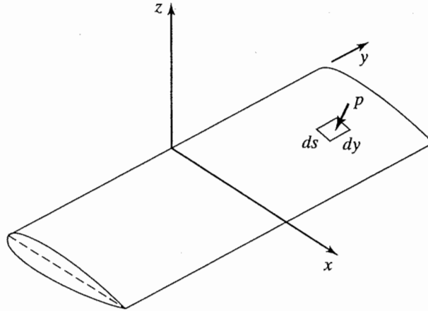
Figure 5.11 Pressure acting on an elemental surface area.
