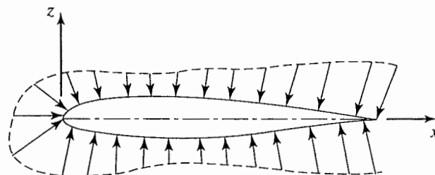
Figure 5.10 Pressure distribution for a lifting airfoil section.
