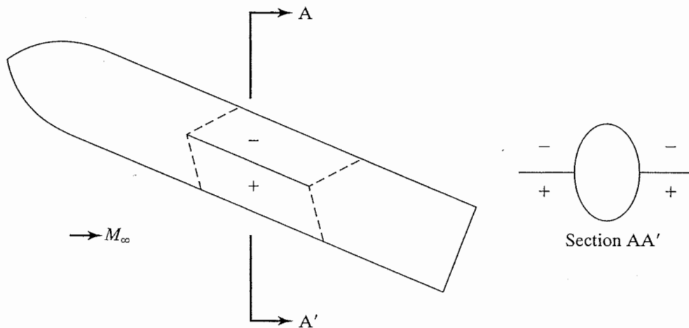
Figure 11.43 Wing-on-body interaction showing regions of positive and negative C_p . [From Hilton (1951).]
