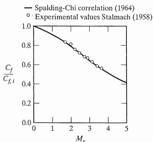
Figure 8.19 Ratio of the compressible, turbulent experimental skin friction coefficient to the incompressible value at the same Reynolds number as a function of Mach number.
