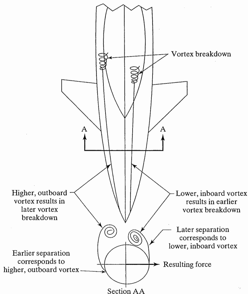
Figure 7.56 Sketch of asymmetric vortices shed from aircraft forebody for \alpha_{AV} \leq \alpha < \alpha_{UV} . [Taken from Cobleigh (1994).]
