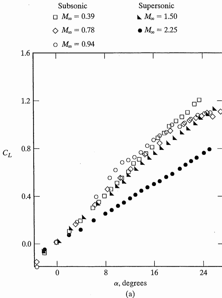
Figure 9.19 Effect of Mach number on the aerodynamic characteristics of a delta wing; AR = 2.31 , \Lambda_{LE} = 60^\circ : (a) lift-coefficient/angle-of-attack correlation. [Data from Stahl and Mackrodt (1965).]
