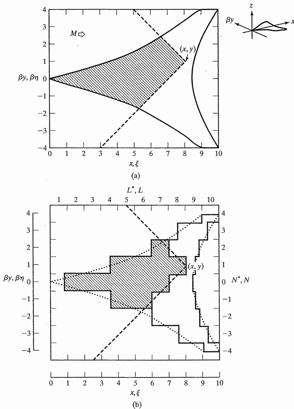
Figure 11.26 Coordinate systems for the linearized, supersonic vortex lattice method: (a) Cartesian coordinate system; (b) grid system used in numerical solution.
