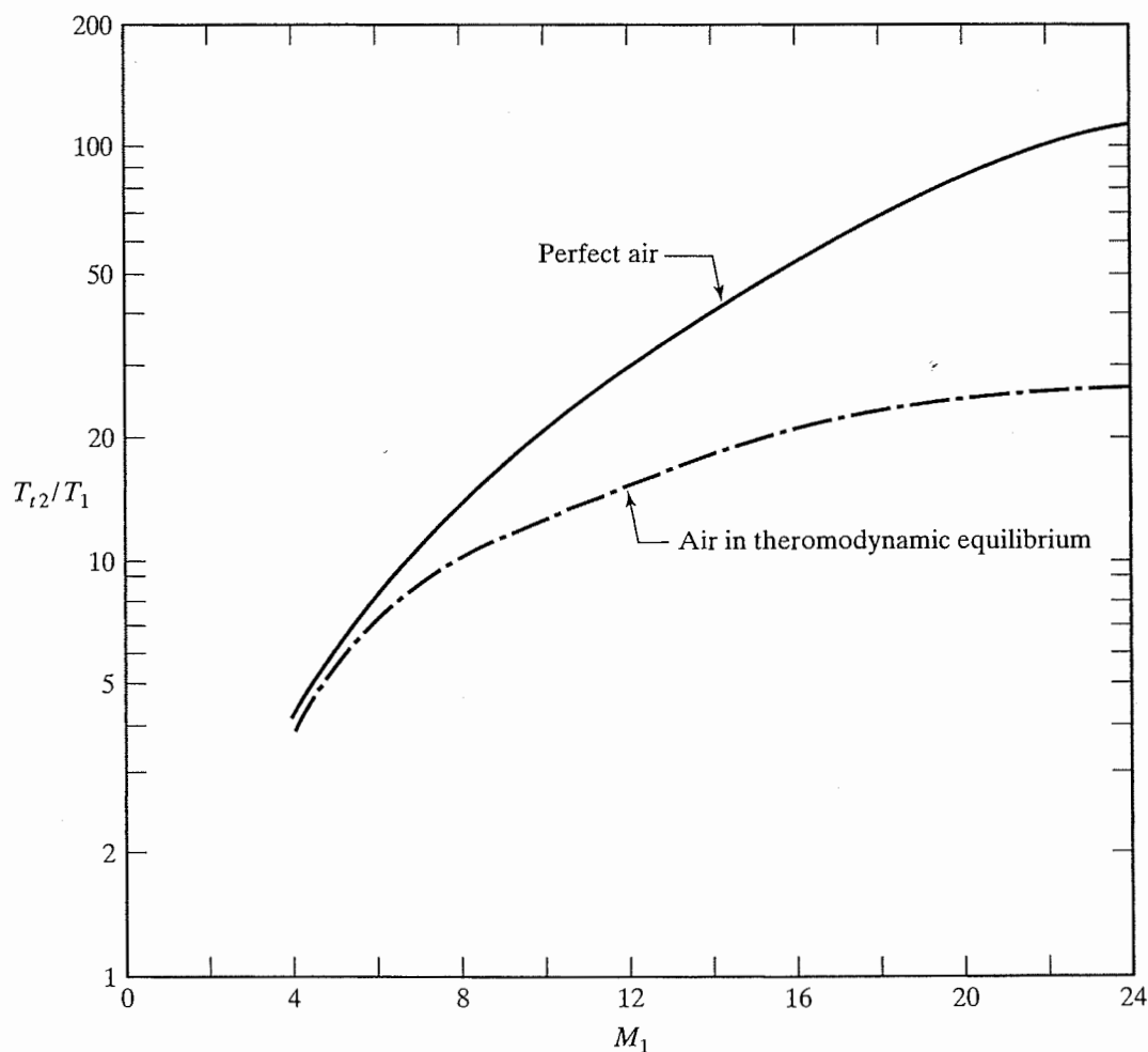
Figure 12.6 Temperature at the stagnation point (at the edge of the boundary layer) of a sphere ( R_N = 0.3048 m) at an altitude of 45,721 m.
