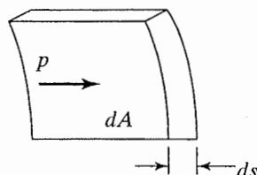
Figure 2.14 Incremental work done by the pressure force, which acts normal to the surface.
