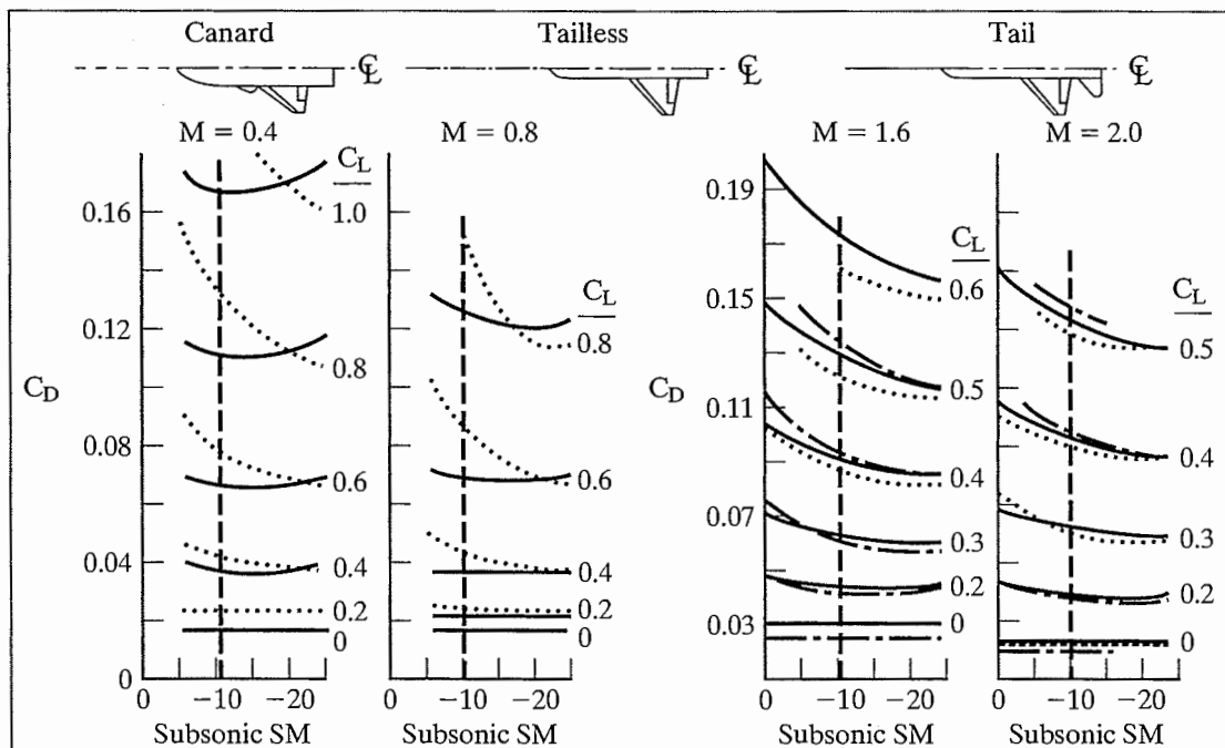
Figure 13.47 Summary of trimmed drag comparison of canard, tail, and tailless arrangements with the 44-degree sweep trapezoidal wing. [From Nicholas et al. (1984).]
