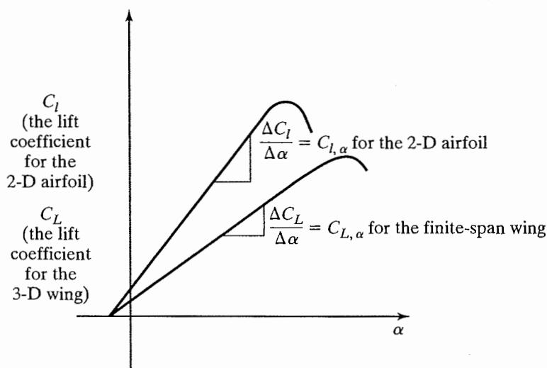
Figure 5.25 Comparison of the lift-curve slope of a two-dimensional airfoil with that for a finite-span wing.
