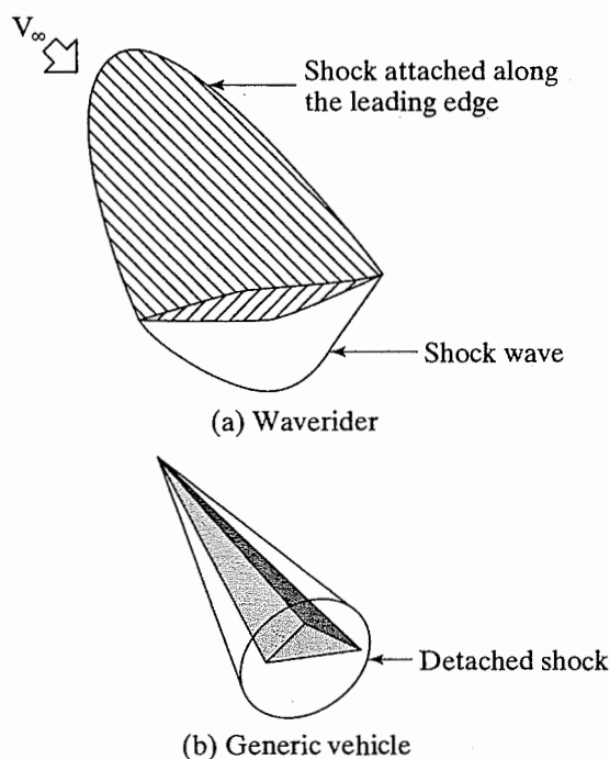
Figure 12.22 Comparison of a waverider with a generic hypersonic configuration. [Taken from Anderson et al. (1990).]
